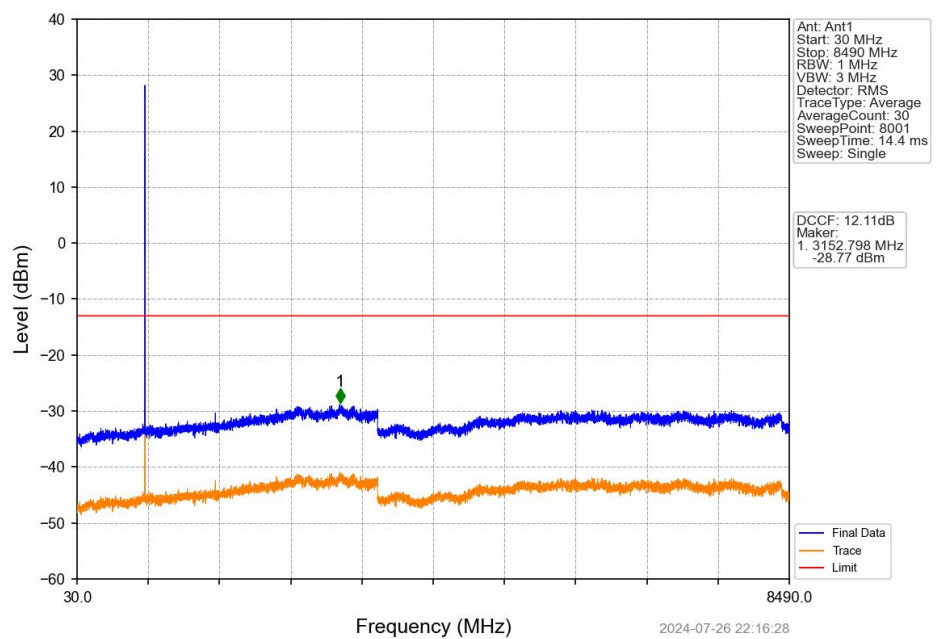
GSM850 GSM_MCH_836.6MHz_GSM_NTNV
