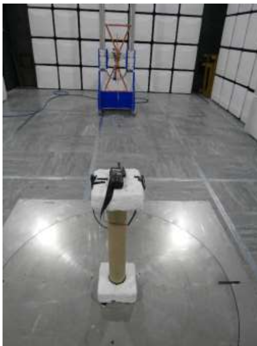
Figure 14 – Test Setup - 30 MHz to 1 GHz – X Orientation
