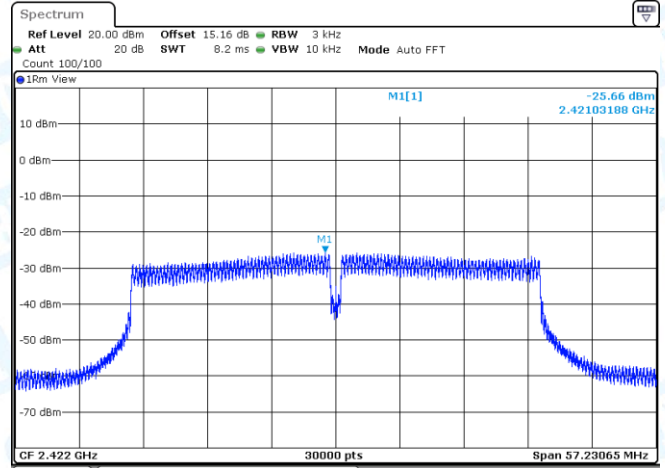
11N40MIMO-Ant1-2422-PASS
