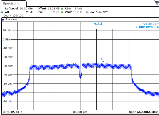
11N40MIMO-Ant2-2422-PASS
