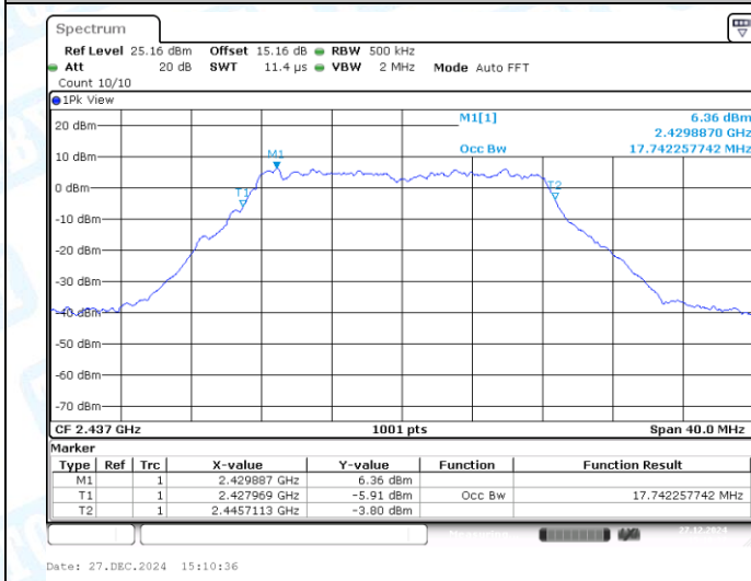
11G-CDD-Ant1-2437
