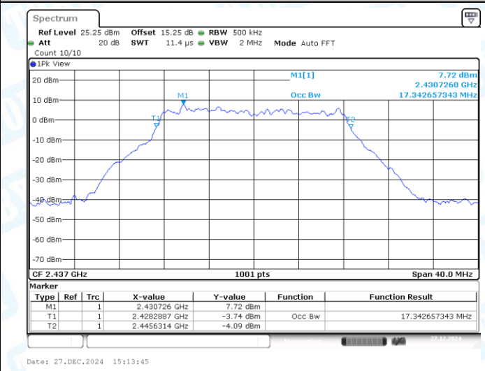
11G-CDD-Ant2-2437
