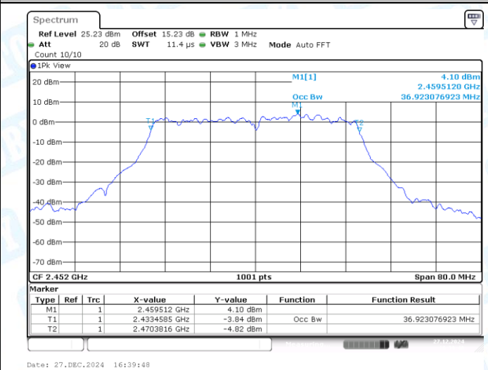
11N40MIMO-Ant2-2452
