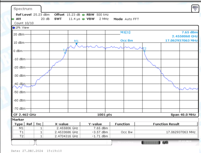
11G-CDD-Ant2-2462
