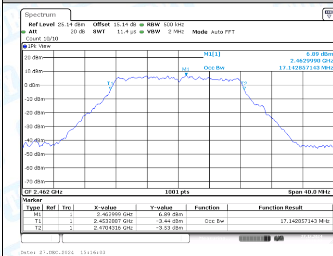
11G-CDD-Ant1-2462
