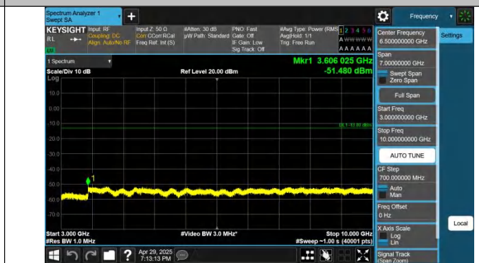
Band5-1.4MHz-QPSK-20643-1RB#5-3000~10000-PASS
