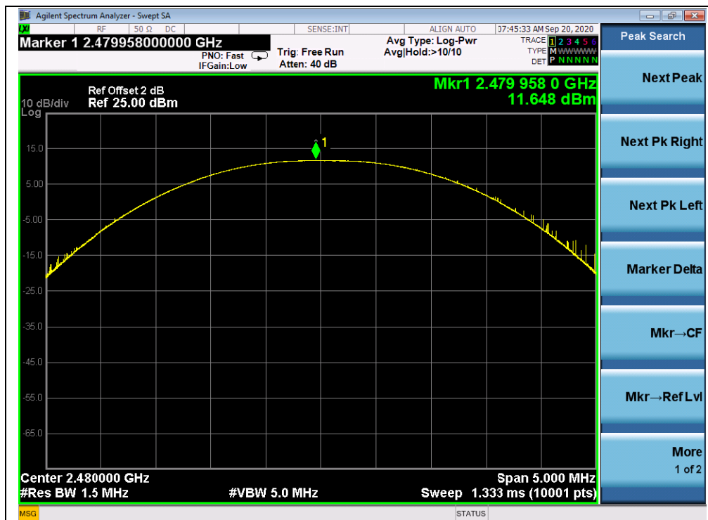
(Channel 78, GFSK)
