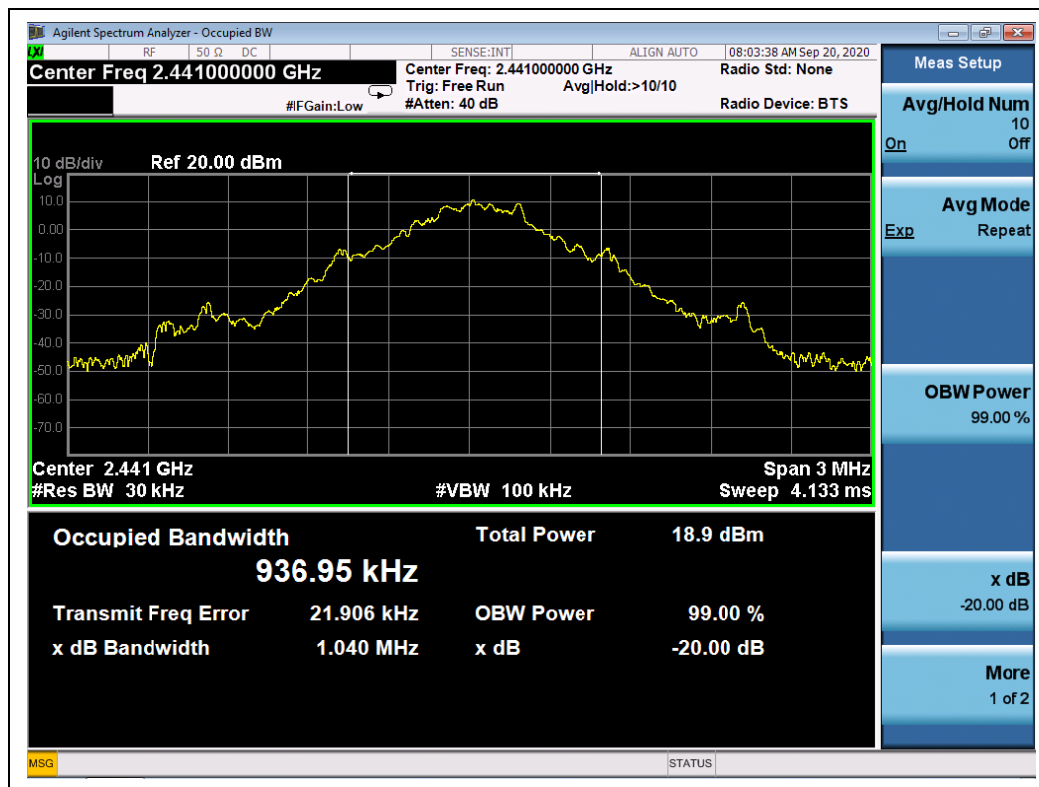
(Channel 39, GFSK)
