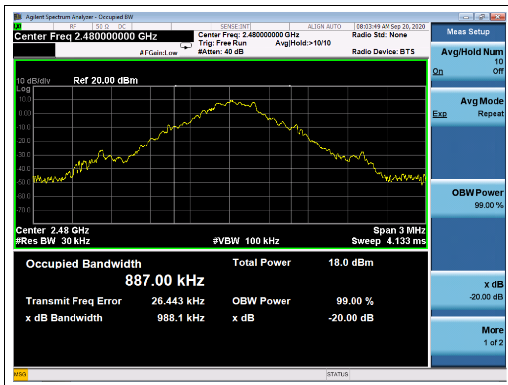
(Channel 78, GFSK)
