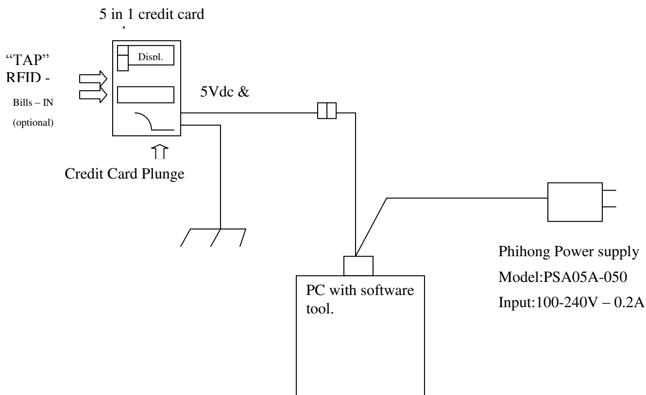
Figure 1: Test Configuration
