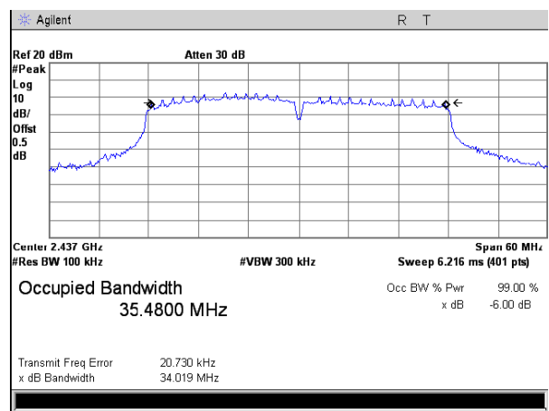
(802.11n40) channel 6
