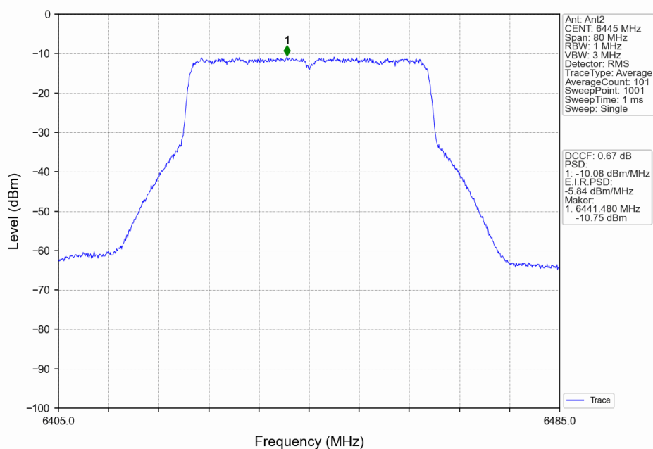
802.11ax(HEW40)_LCH_6445MHz_RU484_Left_MIMO_NTNV
