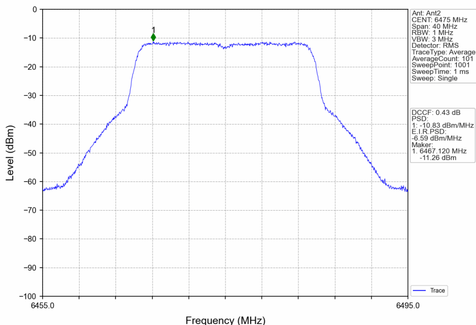
802.11ax(HEW20)_MCH_6475MHz_RU242_Left_MIMO_NTNV
