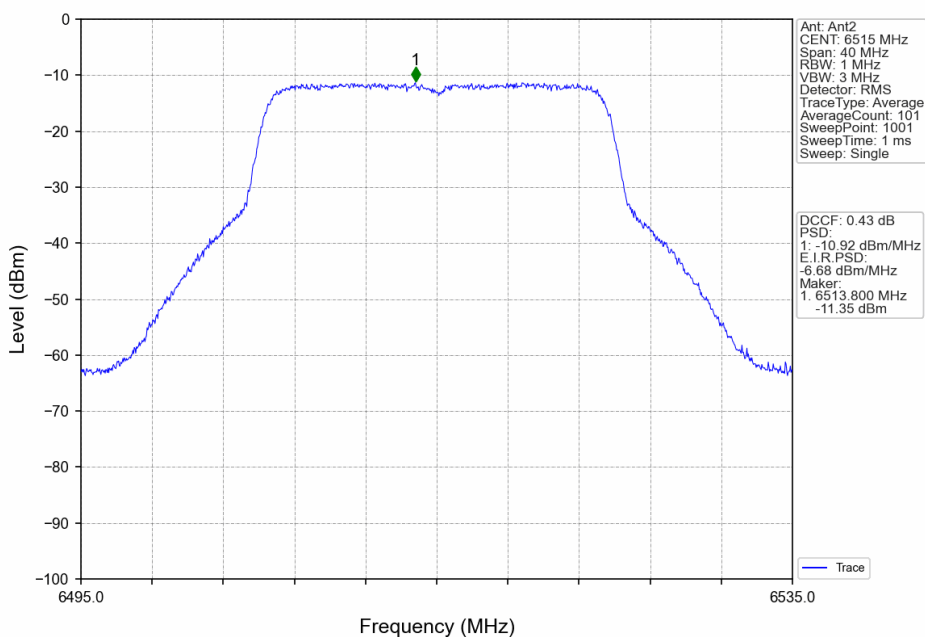
802.11ax(HEW20)_HCH_6515MHz_RU242_Left_Ant2_NTNV
