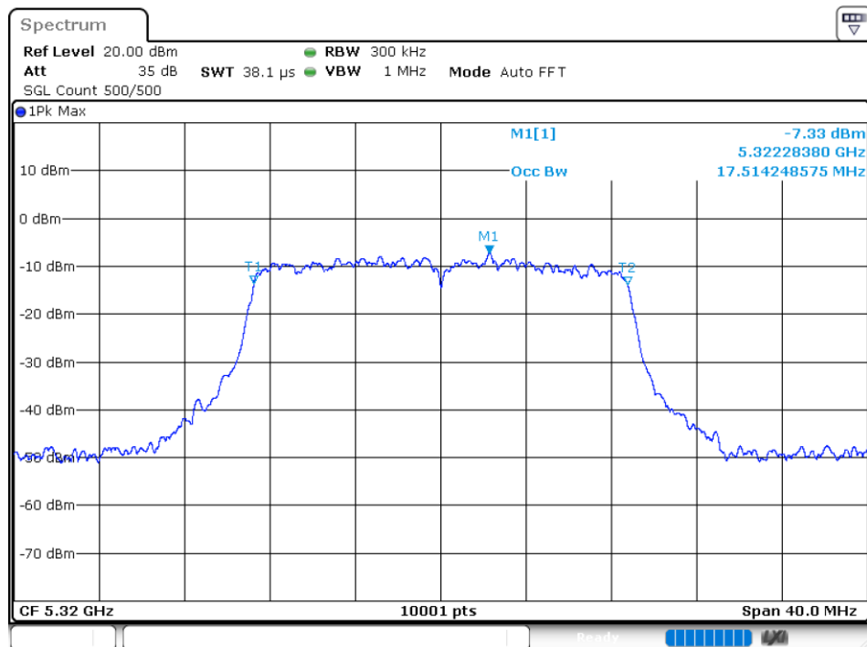
OBW NVNT 802.11ac20 5320MHz Ant 2
