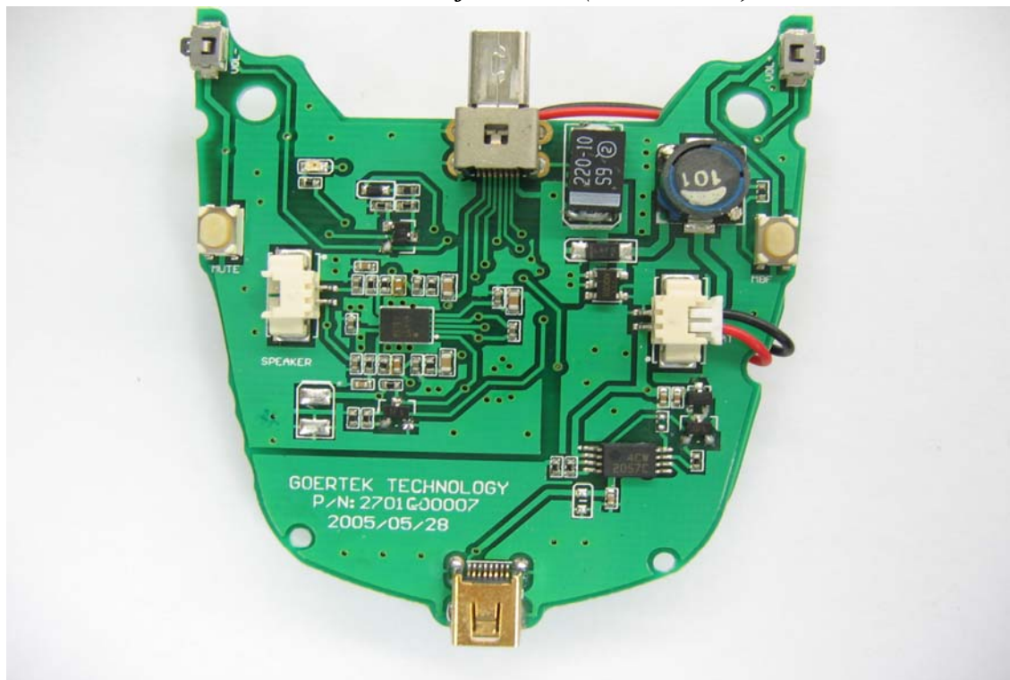
Internal View of EUT – 1 (Car Kit Base)
