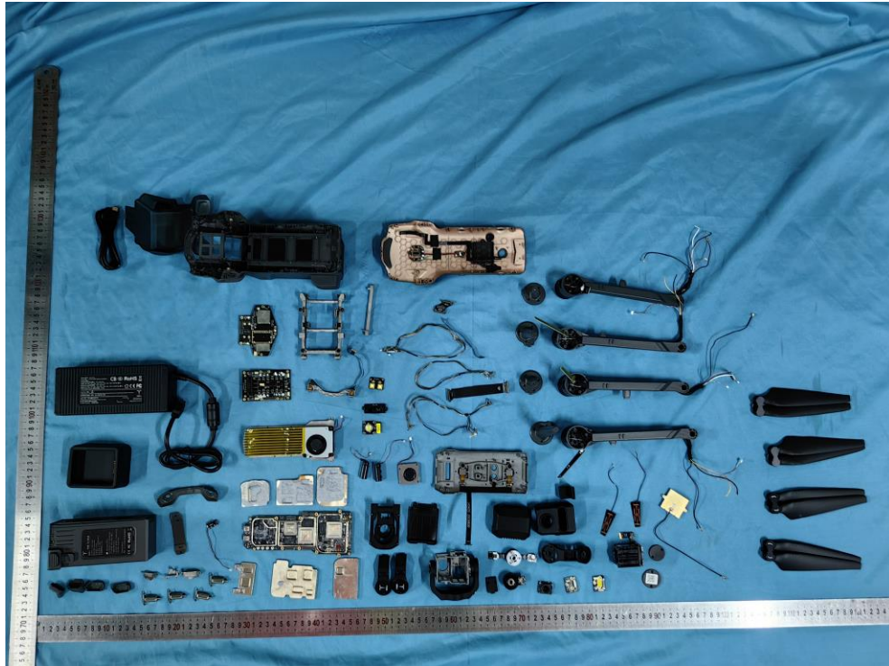
Internal Structure
