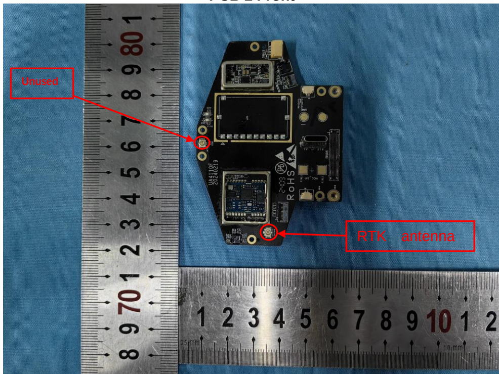
PCB 2 Back
