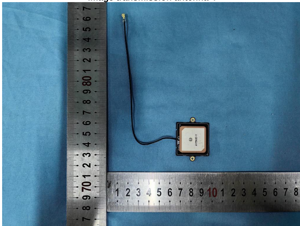
RTK antenna
