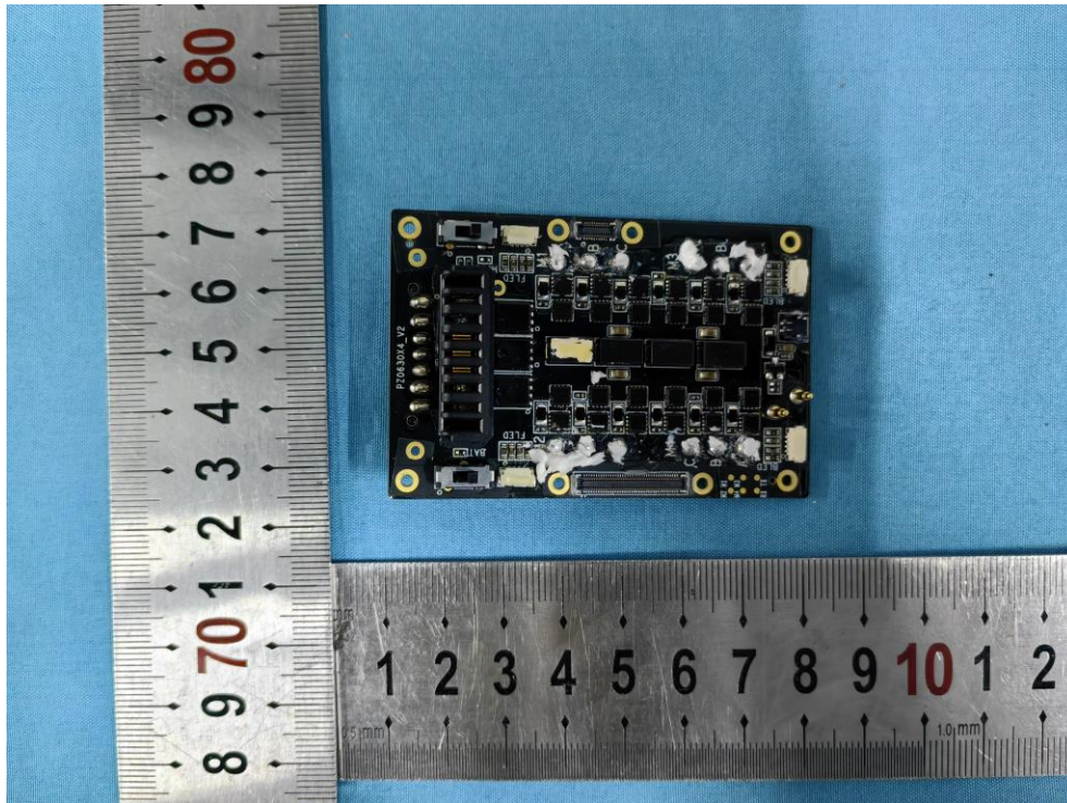
PCB 3 Front
