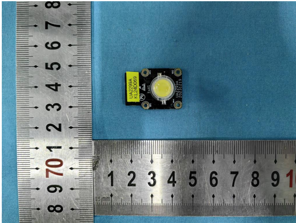
PCB 4 Front
