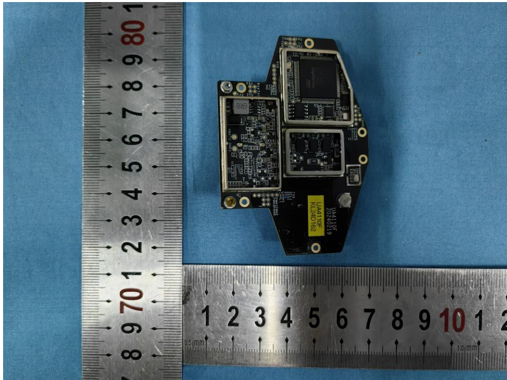
PCB 2 Front
