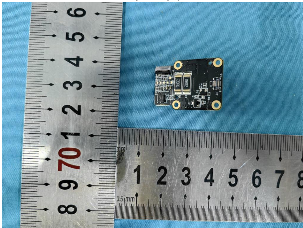
PCB 4 Back
