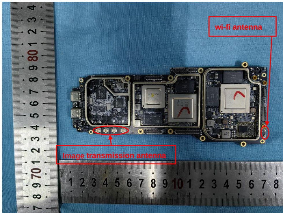
PCB 1 Front
