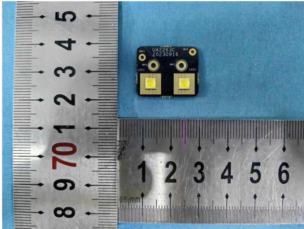
PCB 5 Front
