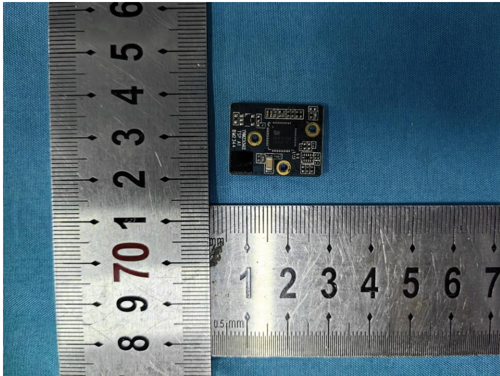
PCB 6 Front
