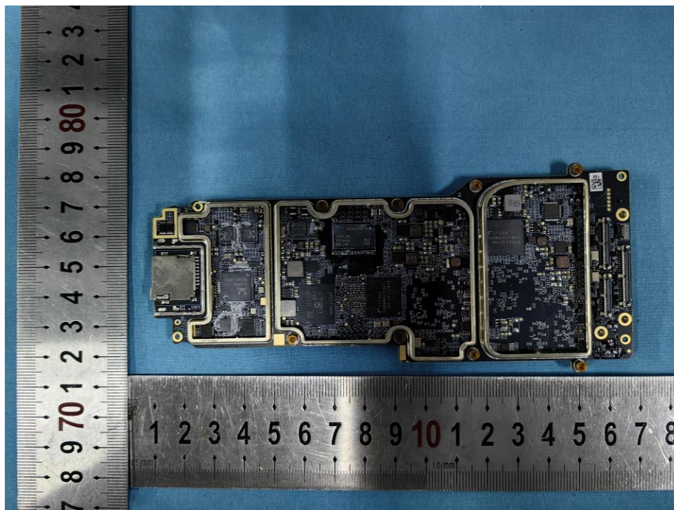
PCB 1 Back
