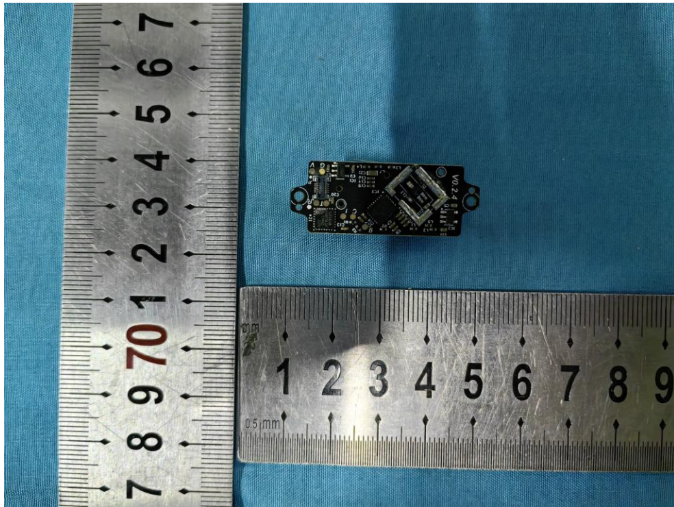
PCB 10 Front
