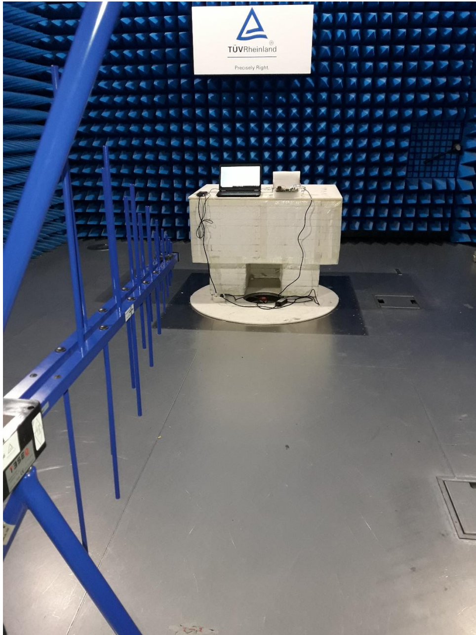
Photo 1 Photograph test setup radiated emissions 30-1000 MHz FCC 15, 2.4 GHz WiFi + BT Mode / 5 GHz Mode
