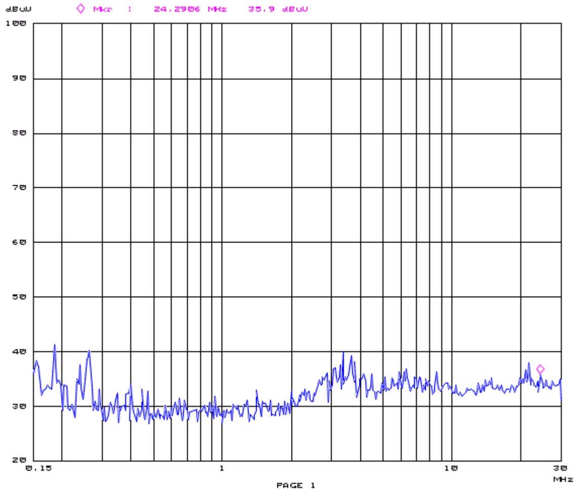
Plot 8: Pre-scan plot with peak detector. Conducted emissions from 0.15 - 30 MHz, 5 GHz WiFi Mode.
