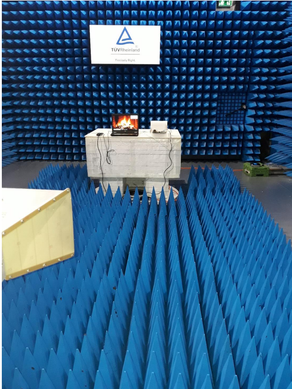
Photo 2: Photograph radiated emissions 1 – 18 GHz
