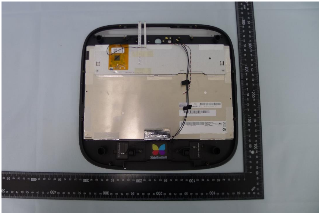
( 46 ) EUT Photo_BUTTERFLYMX.M12.1
