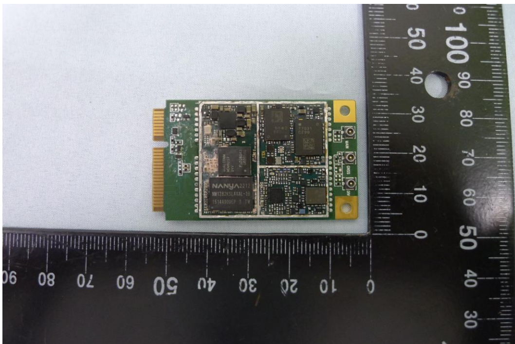
( 10 ) EUT Photo_BUTTERFLYMX.M12.1
