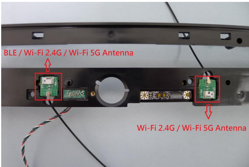
( 50 ) EUT Photo_BUTTERFLYMX.M12.1
