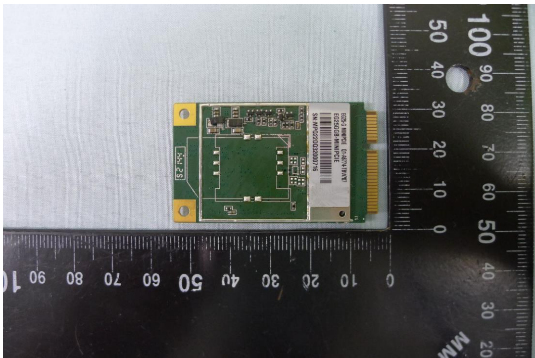
( 12 ) EUT Photo_BUTTERFLYMX.M12.1
