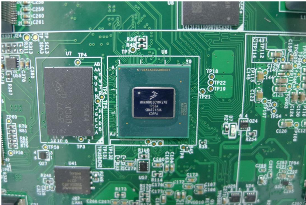
( 26 ) EUT Photo_BUTTERFLYMX.M12.1
