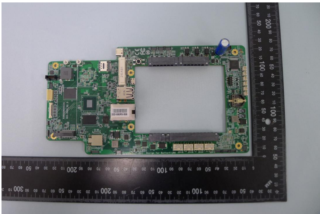
( 18 ) EUT Photo_BUTTERFLYMX.M12.1
