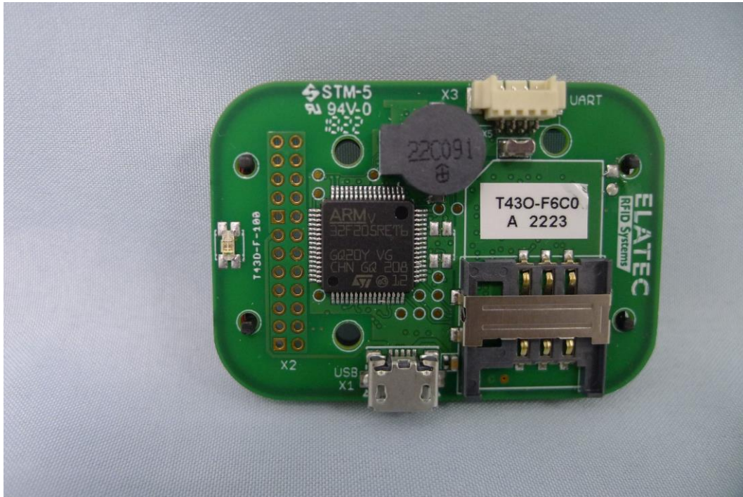
( 40 ) EUT Photo_BUTTERFLYMX.M12.1
