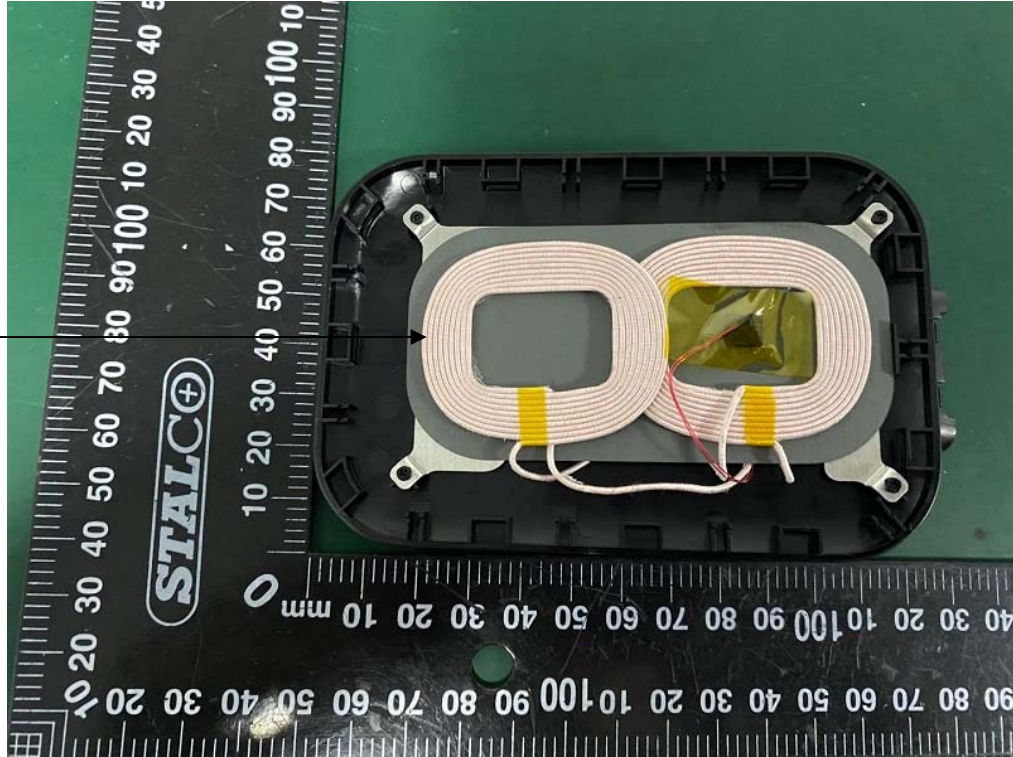
Coil Antenna
