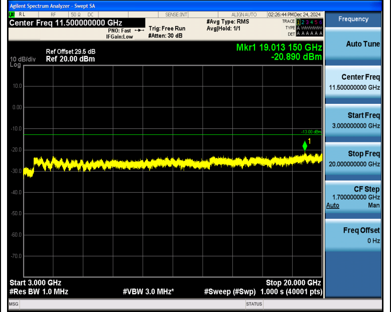
Band4_3MHz_QPSK_19965_1RB#0_3000~20000_3000~20000
