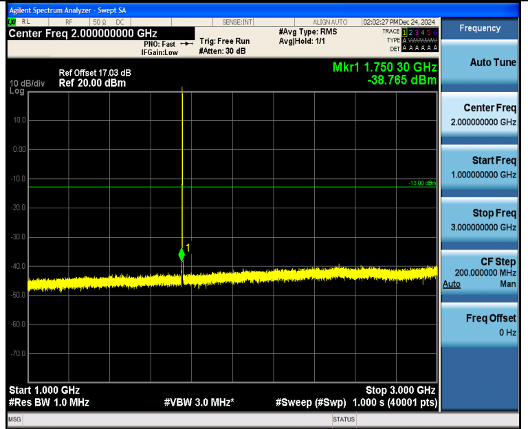
Band4_1.4MHz_16QAM_20393_6RB#0_1000~3000_1000~3000
