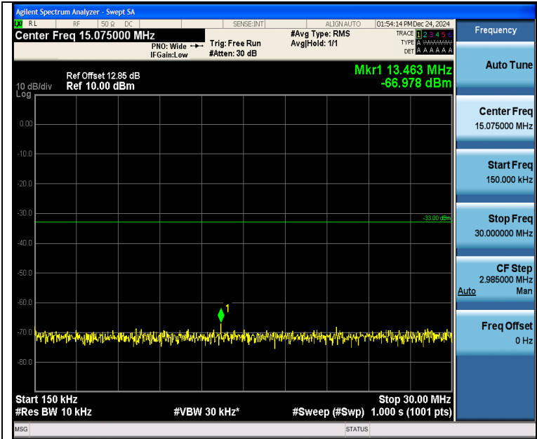
Band4_1.4MHz_QPSK_20175_6RB#0_0.15~30_0.15~30
