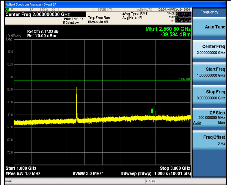
Band4_3MHz_16QAM_19965_1RB#14_1000~3000_1000~3000
