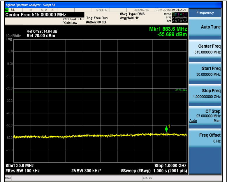
Band4_1.4MHz_QPSK_20175_6RB#0_30~1000_30~1000
