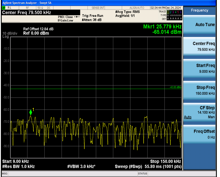
Band4_3MHz_QPSK_20175_1RB#14_0.009~0.15_0.009~0.15
