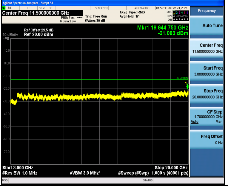
Band4_1.4MHz_QPSK_20393_1RB#5_3000~20000_3000~20000
