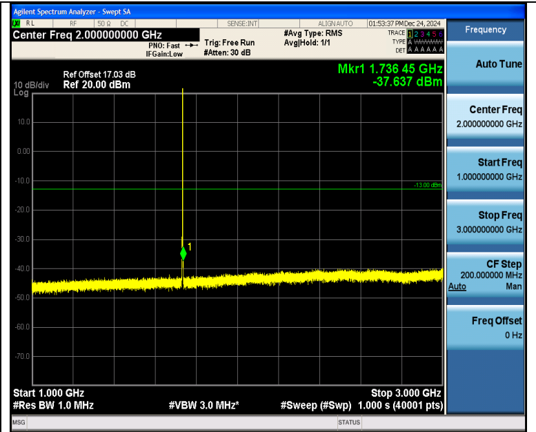
Band4_1.4MHz_16QAM_20175_1RB#5_1000~3000_1000~3000
