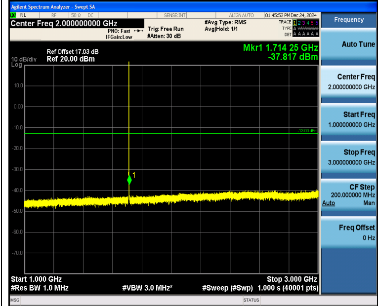
Band4_1.4MHz_QPSK_19957_1RB#5_1000~3000_1000~3000
