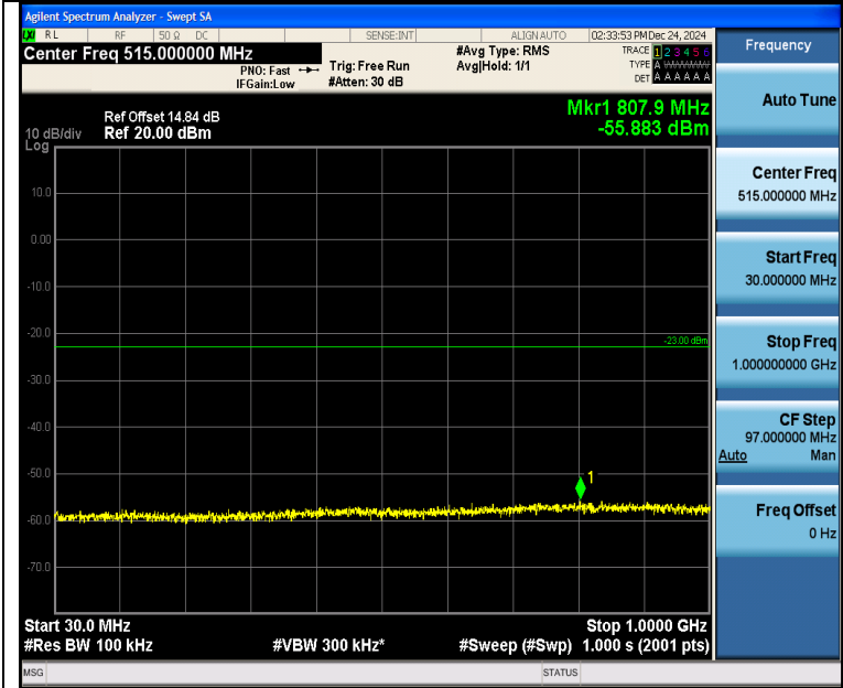
Band4_3MHz_16QAM_20175_1RB#0_30~1000_30~1000
