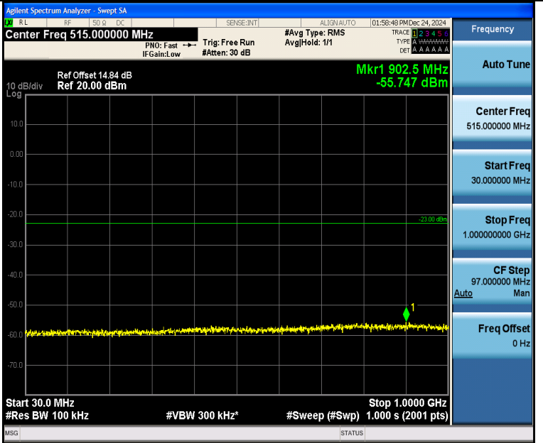
Band4_1.4MHz_QPSK_20393_1RB#5_30~1000_30~1000
