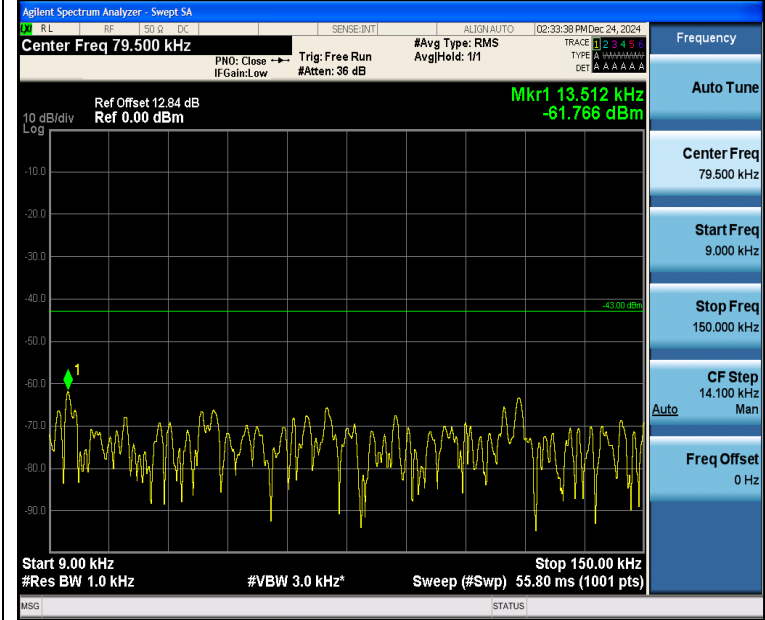
Band4_3MHz_16QAM_20175_1RB#0_0.009~0.15_0.009~0.15
