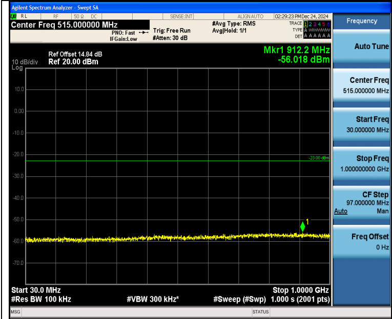
Band4_3MHz_16QAM_19965_1RB#14_30~1000_30~1000
