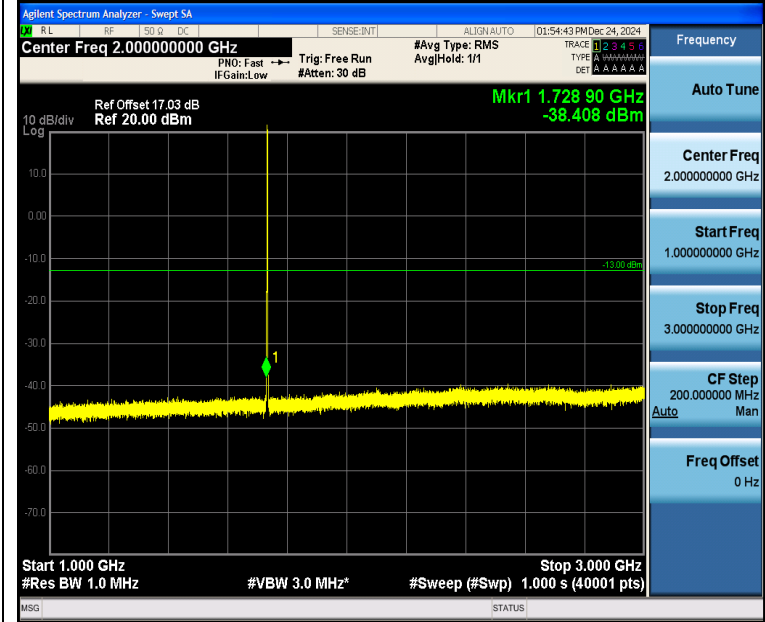
Band4_1.4MHz_QPSK_20175_6RB#0_1000~3000_1000~3000
