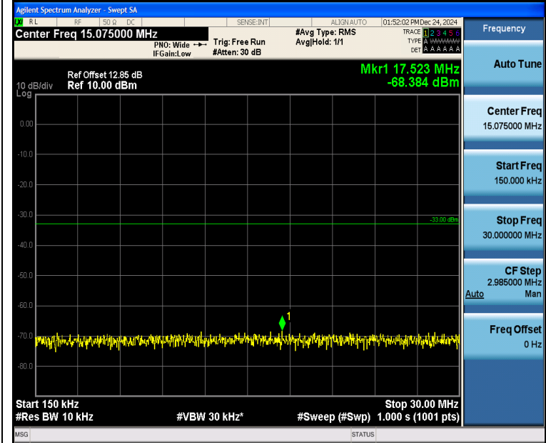
Band4_1.4MHz_QPSK_20175_1RB#5_0.15~30_0.15~30
