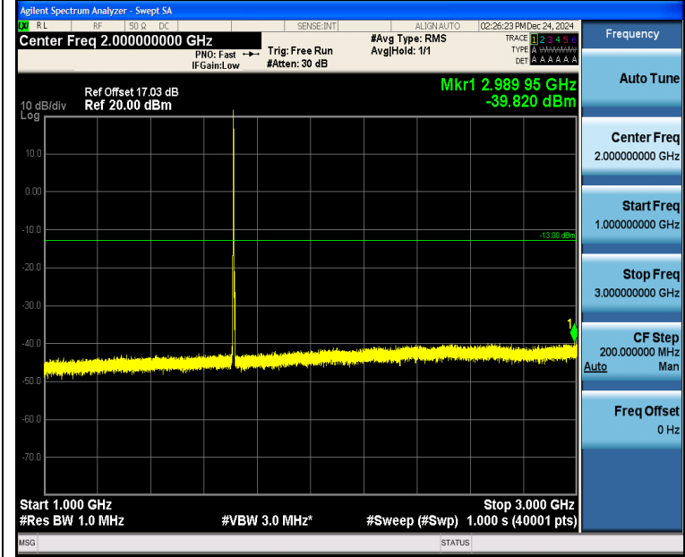
Band4_3MHz_QPSK_19965_1RB#0_1000~3000_1000~3000
