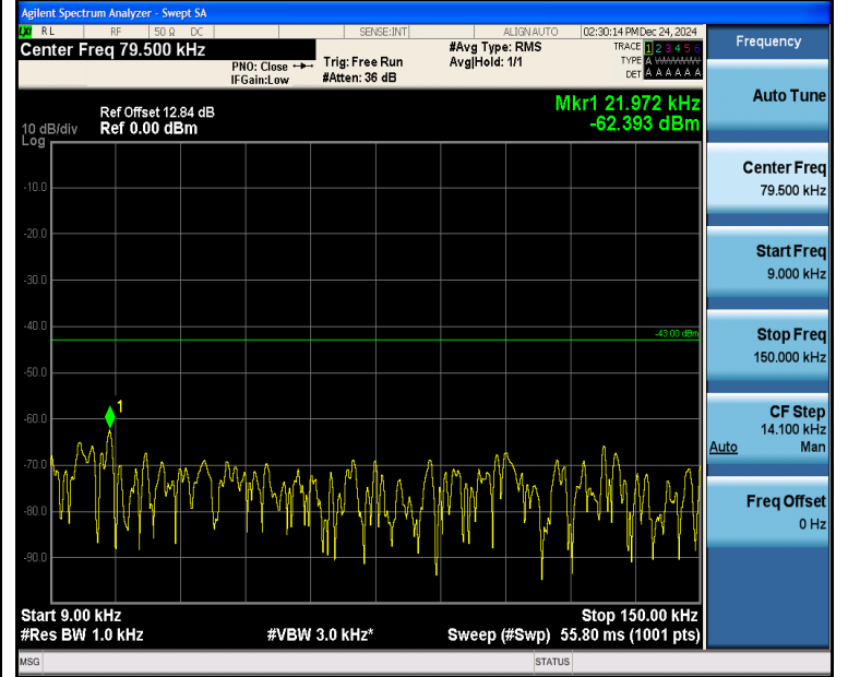
Band4_3MHz_QPSK_19965_15RB#0_0.009~0.15_0.009~0.15
