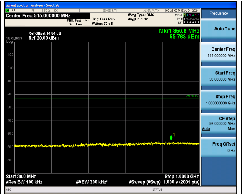
Band4_3MHz_QPSK_19965_1RB#0_30~1000_30~1000
