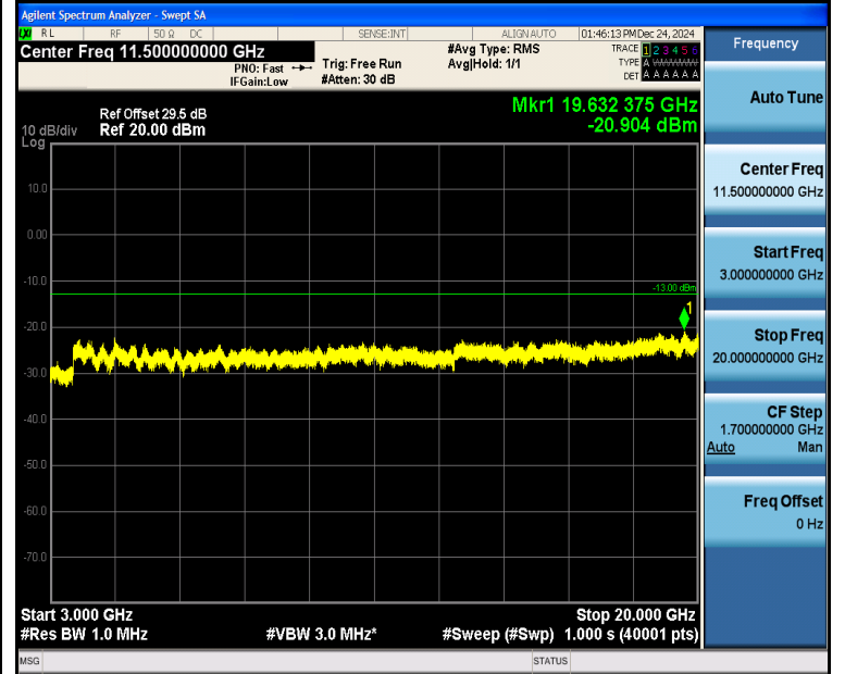
Band4_1.4MHz_QPSK_19957_1RB#5_3000~20000_3000~20000
