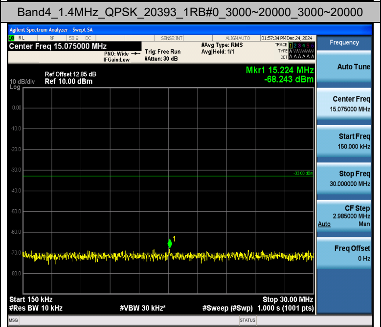
Band4_1.4MHz_QPSK_20393_1RB#0_3000~20000_3000~20000
