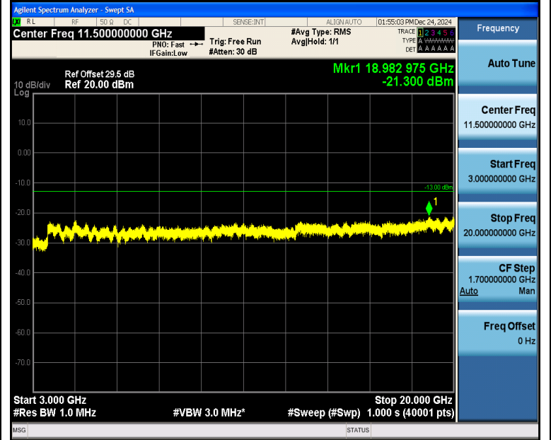
Band4_1.4MHz_QPSK_20175_6RB#0_3000~20000_3000~20000
