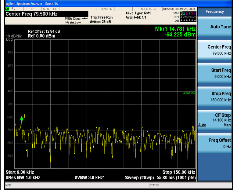
Band4_1.4MHz_QPSK_20175_6RB#0_0.009~0.15_0.009~0.15
