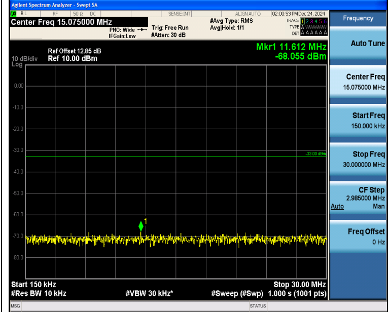
Band4_1.4MHz_QPSK_20393_6RB#0_0.15~30_0.15~30
