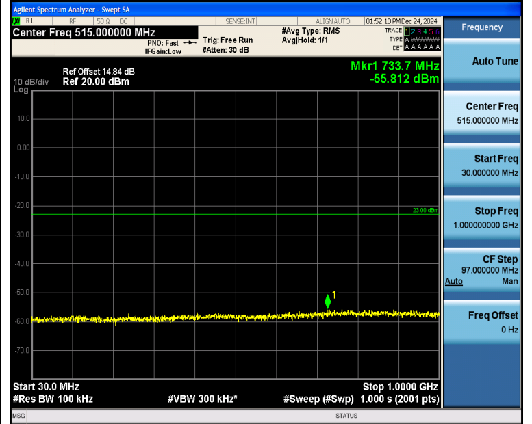
Band4_1.4MHz_QPSK_20175_1RB#5_30~1000_30~1000
