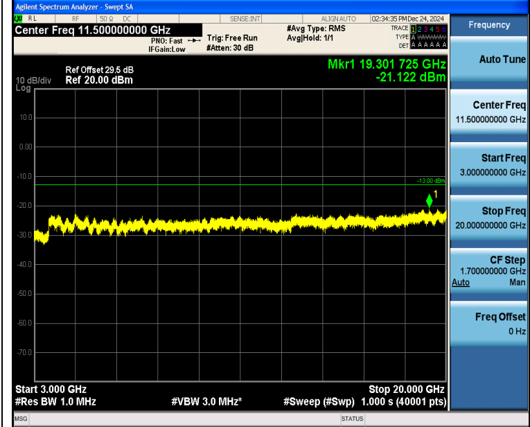
Band4_3MHz_16QAM_20175_1RB#0_3000~20000_3000~20000
