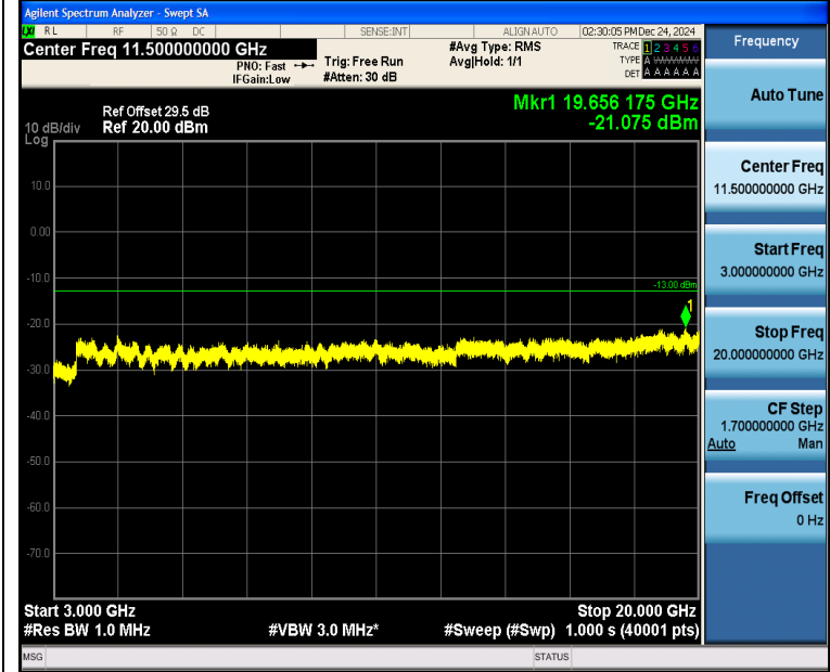
Band4_3MHz_16QAM_19965_1RB#14_3000~20000_3000~20000
