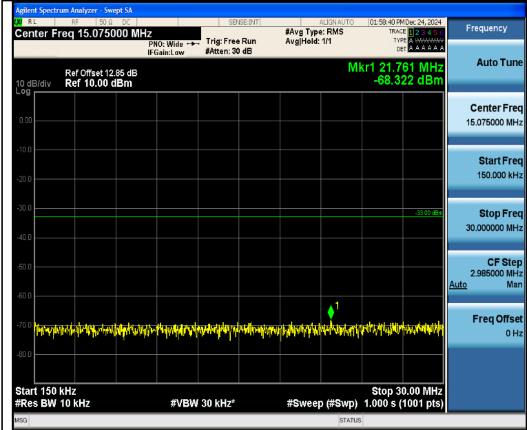
Band4_1.4MHz_QPSK_20393_1RB#5_0.15~30_0.15~30
