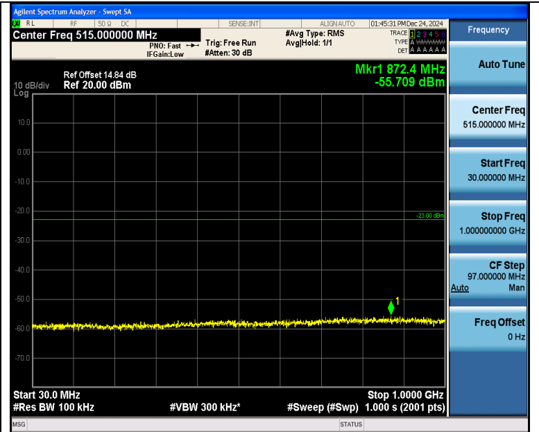
Band4_1.4MHz_QPSK_19957_1RB#5_30~1000_30~1000
