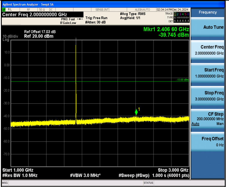
Band4_3MHz_16QAM_20175_1RB#0_1000~3000_1000~3000
