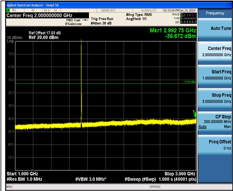
Band4_3MHz_QPSK_20175_1RB#0_1000~3000_1000~3000
