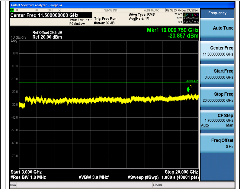
Band4_3MHz_QPSK_20175_1RB#0_3000~20000_3000~20000
