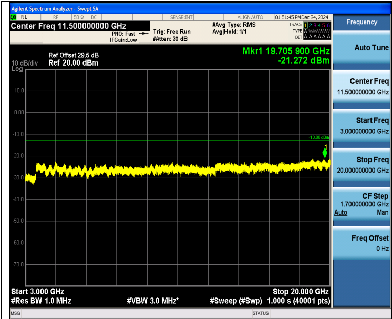
Band4_1.4MHz_16QAM_20175_1RB#0_3000~20000_3000~20000
