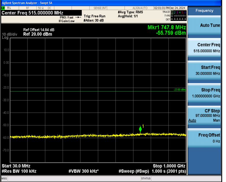
Band4_1.4MHz_QPSK_20393_6RB#0_30~1000_30~1000
