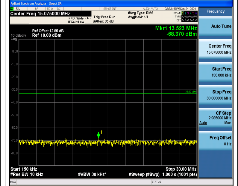
Band4_3MHz_16QAM_20175_1RB#0_0.15~30_0.15~30
