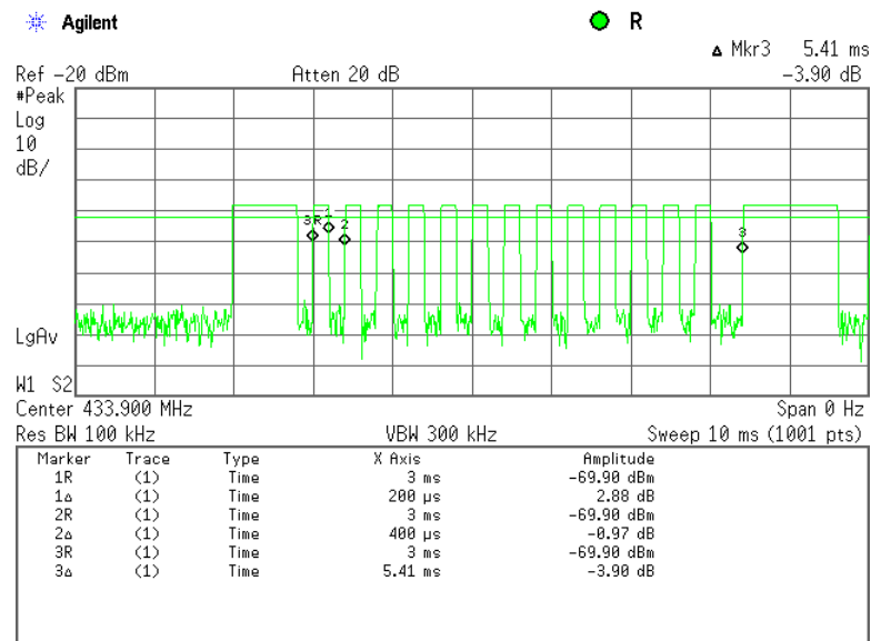
Plot 7.2.26 Pulse transmission duration measurement
