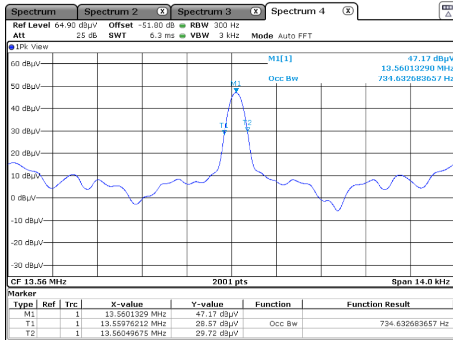
Figure 3 – 99 % Bandwidth, 24 V
