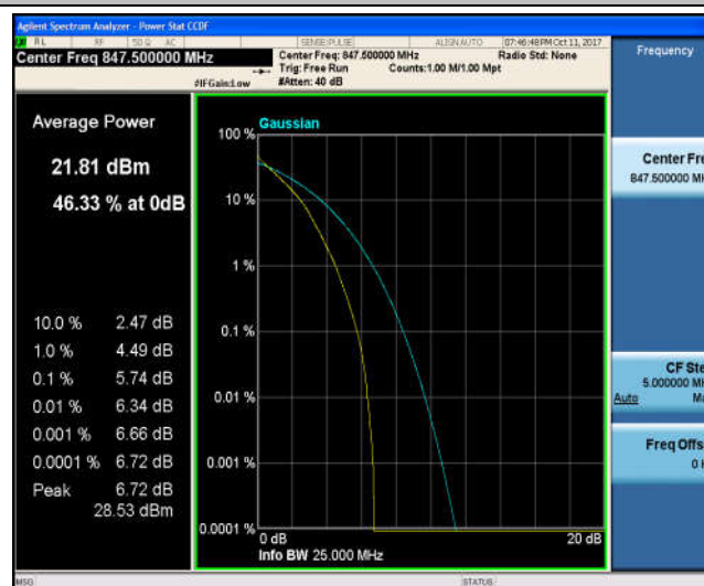
Band5_3MHz_16QAM_20635_15RB#0_6.40_13_PASS
