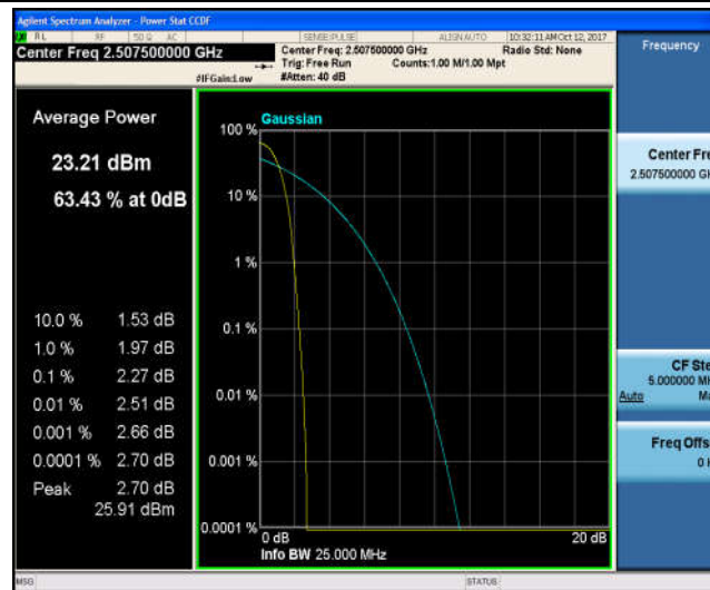
Band7_15MHz_16QAM_20825_1RB#0_3.28_13_PASS
