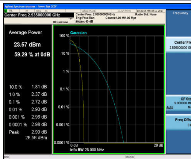
Band7_15MHz_16QAM_21100_1RB#0_3.64_13_PASS
