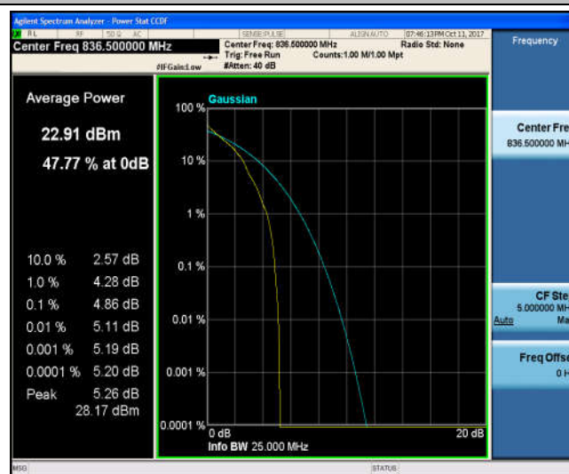
Band5_3MHz_16QAM_20525_1RB#0_5.82_13_PASS
