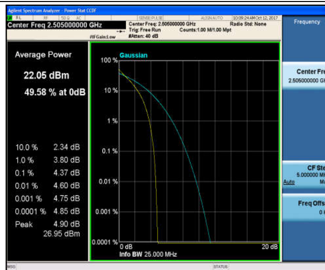
Band7_10MHz_16QAM_20800_50RB#0_5.28_13_PASS
