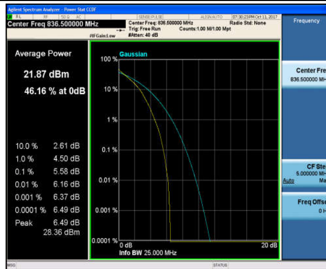
Band5_1.4MHz_16QAM_20525_6RB#0_6.50_13_PASS
