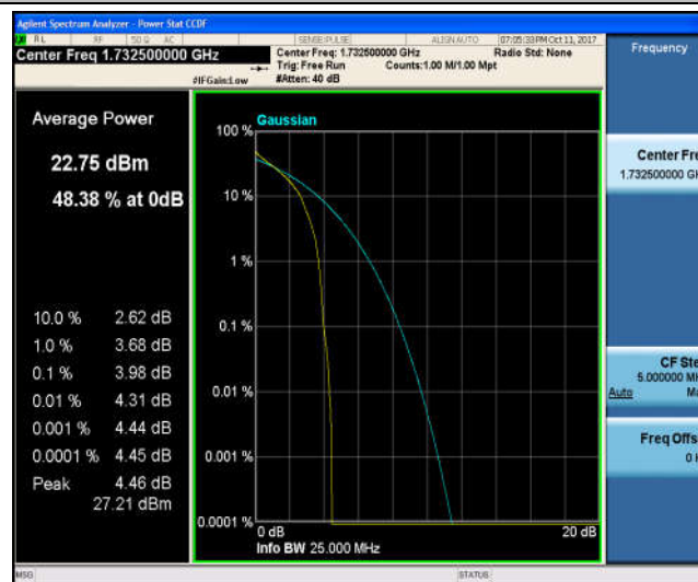
Band4_20MHz_16QAM_20175_1RB#0_4.82_13_PASS
