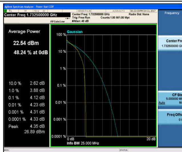
Band4_10MHz_16QAM_20175_1RB#0_5.07_13_PASS
