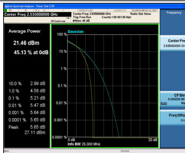
Band7_10MHz_QPSK_21400_1RB#0_2.54_13_PASS
