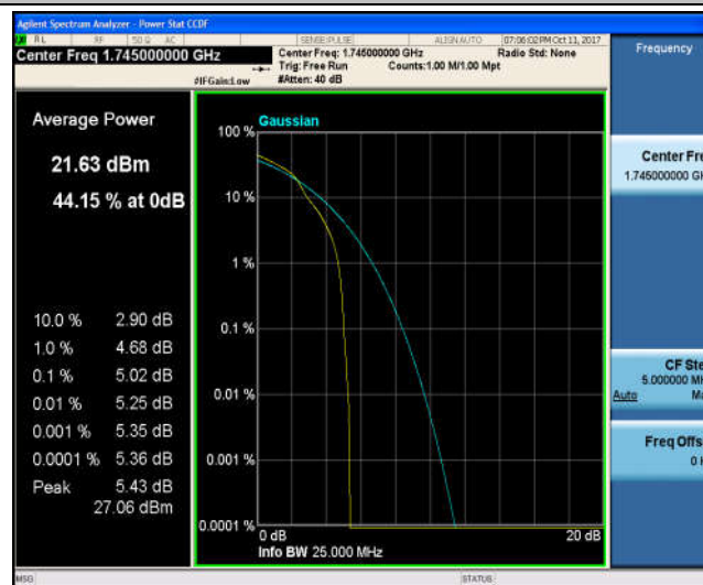
Band4_20MHz_QPSK_20300_100RB#0_5.56_13_PASS
