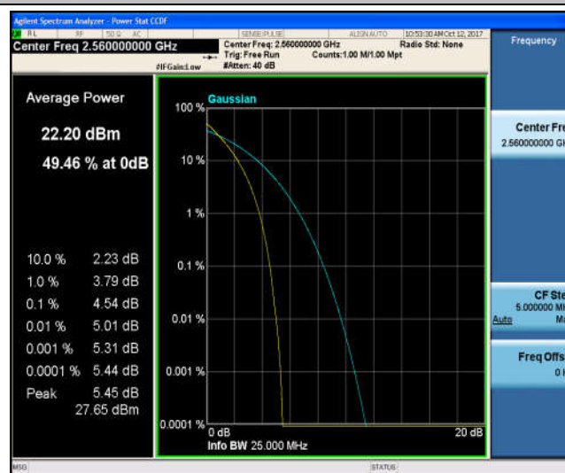
Band7_20MHz_16QAM_21350_100RB#0_5.39_13_PASS
