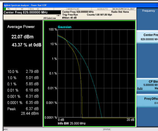
Band5_10MHz_QPSK_20450_50RB#0_5.96_13_PASS
