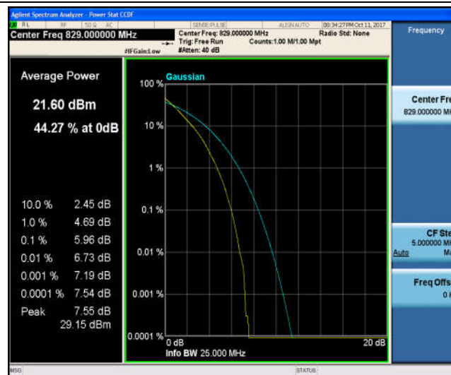
Band5_10MHz_16QAM_20450_50RB#0_6.71_13_PASS
