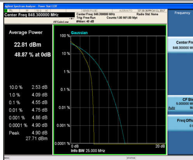
Band5_1.4MHz_16QAM_20643_1RB#0_5.53_13_PASS
