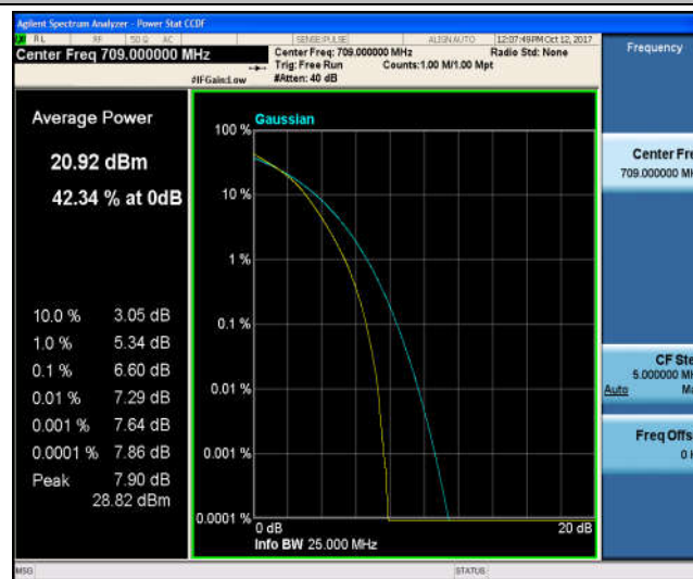
Band17_10MHz_QPSK_23790_1RB#0_5.14_13_PASS
