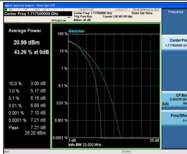
Band4_15MHz_QPSK_20175_1RB#0_3.99_13_PASS
