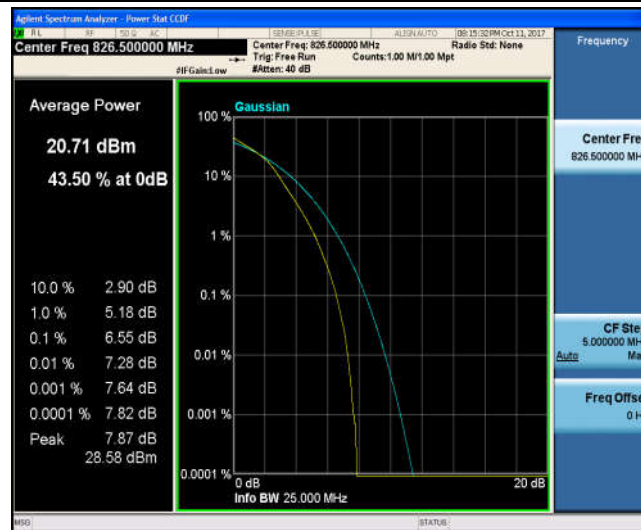
Band5_5MHz_QPSK_20525_1RB#0_5.06_13_PASS
