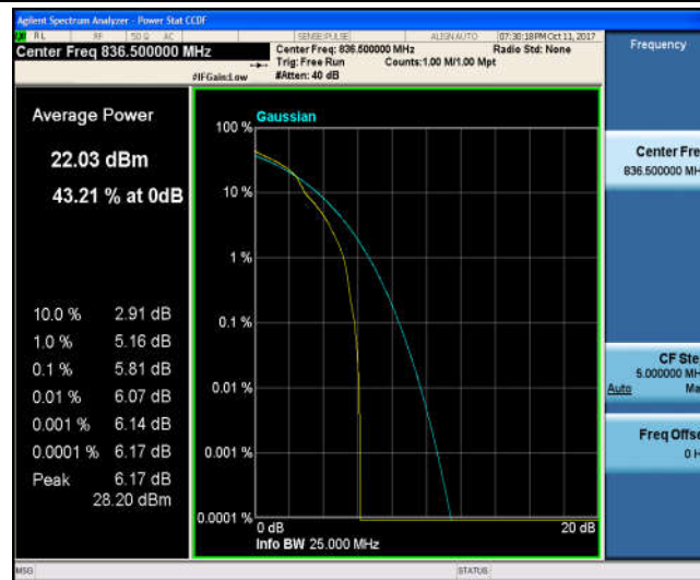
Band5_1.4MHz_QPSK_20525_6RB#0_5.58_13_PASS
