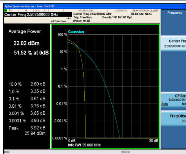
Band7_5MHz_QPSK_20775_25RB#0_4.25_13_PASS
