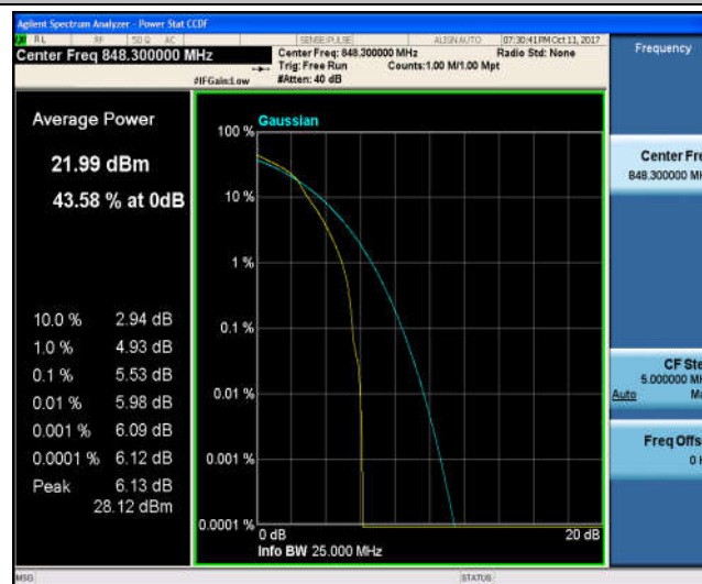
Band5_1.4MHz_QPSK_20643_6RB#0_5.44_13_PASS
