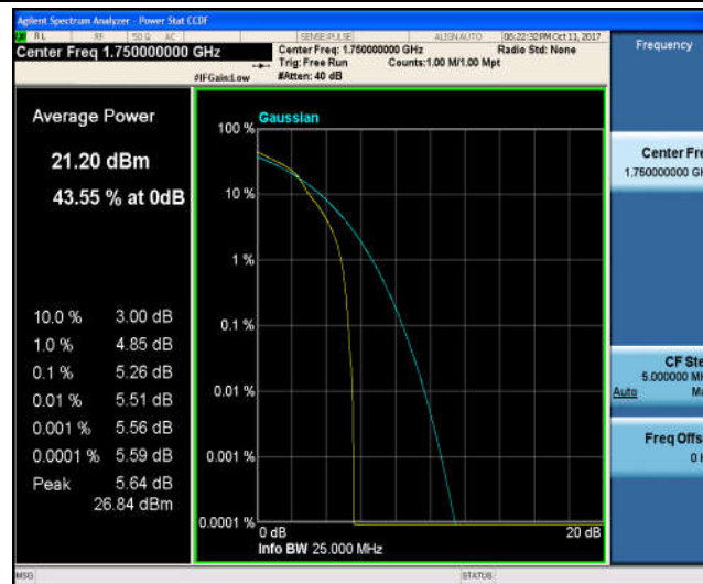
Band4_10MHz_QPSK_20350_50RB#0_5.41_13_PASS
