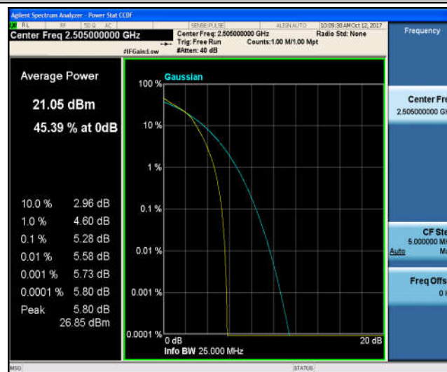
Band7_10MHz_QPSK_21100_1RB#0_2.75_13_PASS
