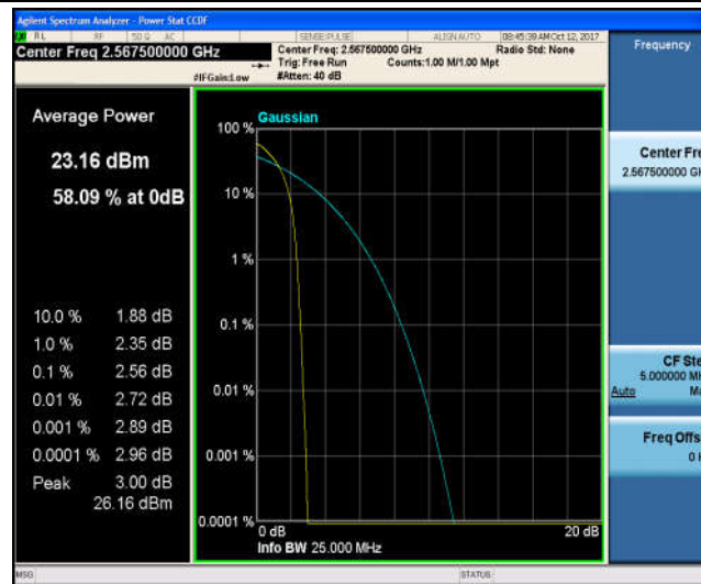
Band7_5MHz_16QAM_21425_1RB#0_3.55_13_PASS
