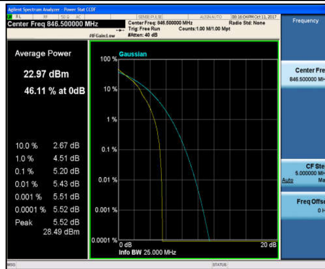
Band5_5MHz_16QAM_20625_1RB#0_6.28_13_PASS
