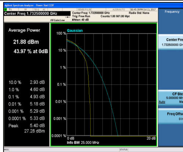
Band4_15MHz_QPSK_20175_75RB#0_5.67_13_PASS
