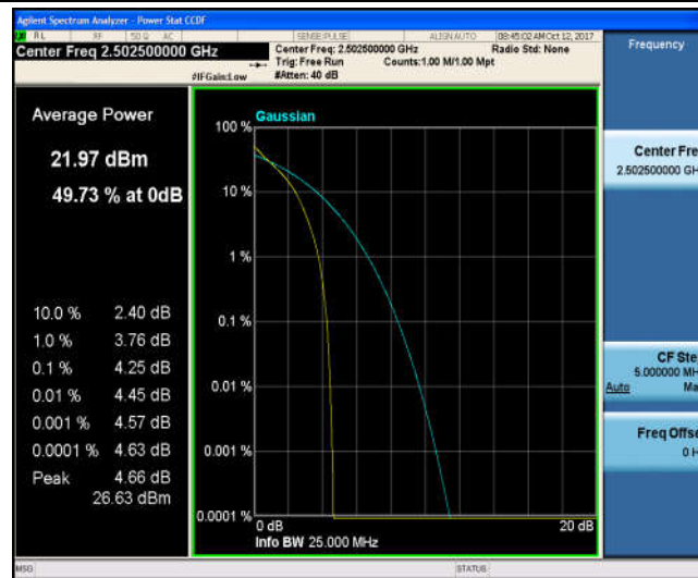
Band7_5MHz_16QAM_20775_25RB#0_5.10_13_PASS
