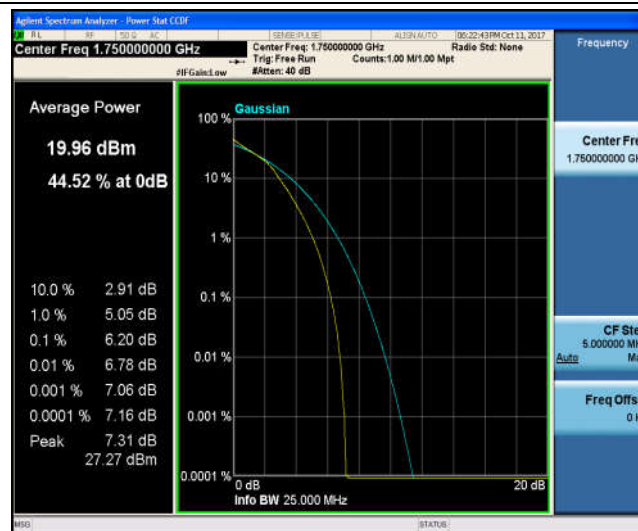
Band4_15MHz_QPSK_20025_1RB#0_3.63_13_PASS
