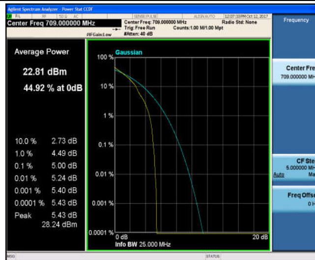
Band17_10MHz_16QAM_23780_1RB#0_6.09_13_PASS
