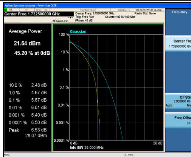
Band4_15MHz_16QAM_20175_75RB#0_6.31_13_PASS
