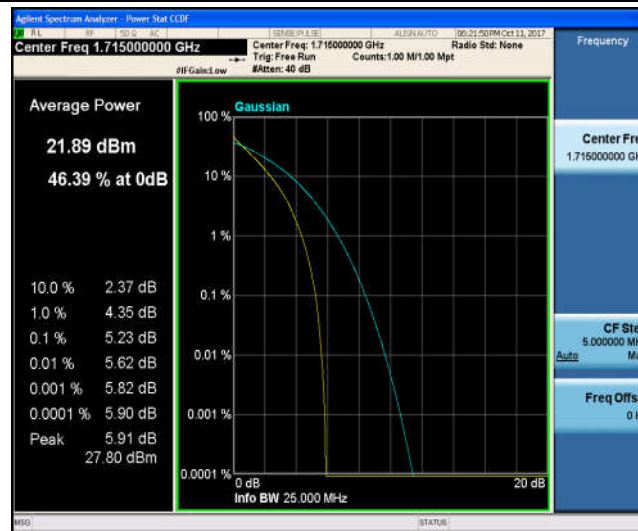
Band4_10MHz_16QAM_20000_50RB#0_6.04_13_PASS
