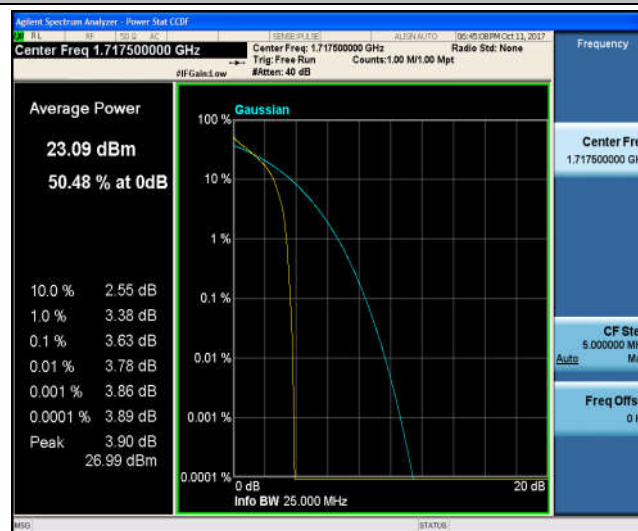
Band4_15MHz_16QAM_20025_1RB#0_4.77_13_PASS
