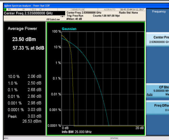
Band7_5MHz_16QAM_21100_1RB#0_3.75_13_PASS
