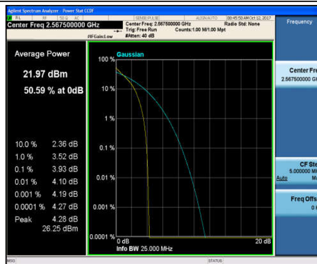
Band7_5MHz_16QAM_21425_25RB#0_4.84_13_PASS
