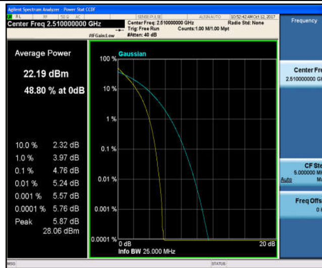
Band7_20MHz_16QAM_20850_100RB#0_5.65_13_PASS
