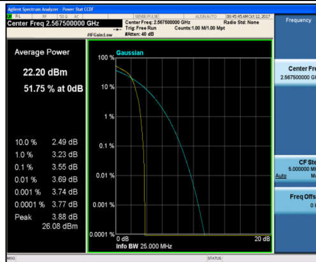
Band7_5MHz_QPSK_21425_25RB#0_3.93_13_PASS
