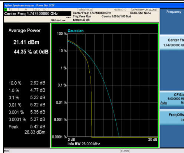
Band4_15MHz_QPSK_20325_75RB#0_5.68_13_PASS
