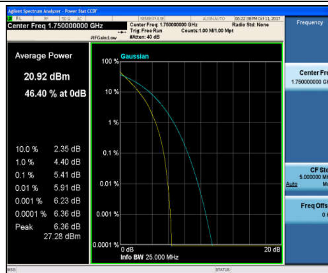
Band4_10MHz_16QAM_20350_50RB#0_6.20_13_PASS
