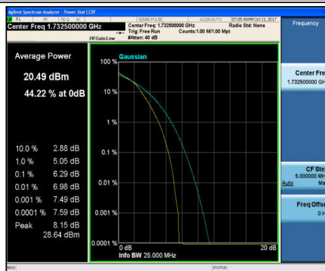
Band4_20MHz_QPSK_20300_1RB#0_4.21_13_PASS
