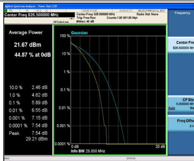
Band5_5MHz_16QAM_20425_25RB#0_6.55_13_PASS
