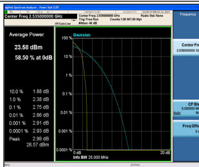
Band7_10MHz_16QAM_21100_1RB#0_3.75_13_PASS
