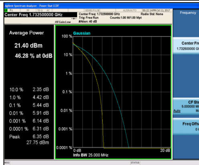
Band4_10MHz_16QAM_20175_50RB#0_6.18_13_PASS
