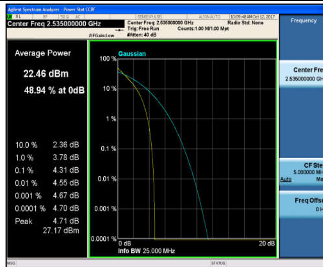
Band7_10MHz_16QAM_21100_50RB#0_5.21_13_PASS
