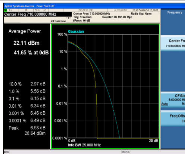
Band17_5MHz_QPSK_23790_25RB#0_5.78_13_PASS
