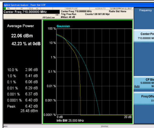
Band17_10MHz_QPSK_23790_50RB#0_5.74_13_PASS
