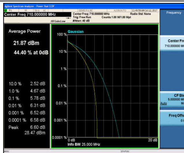
Band17_5MHz_16QAM_23790_25RB#0_6.49_13_PASS
