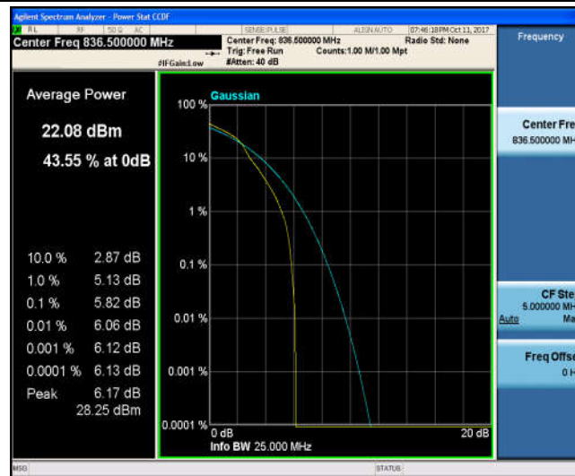
Band5_3MHz_QPSK_20525_15RB#0_5.63_13_PASS
