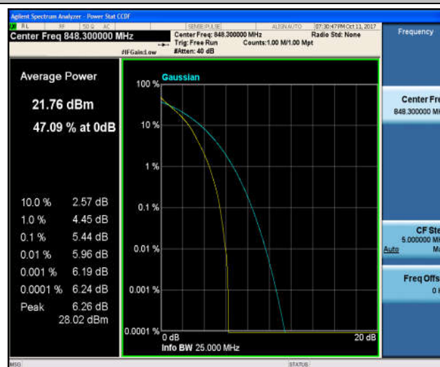
Band5_1.4MHz_16QAM_20643_6RB#0_6.33_13_PASS
