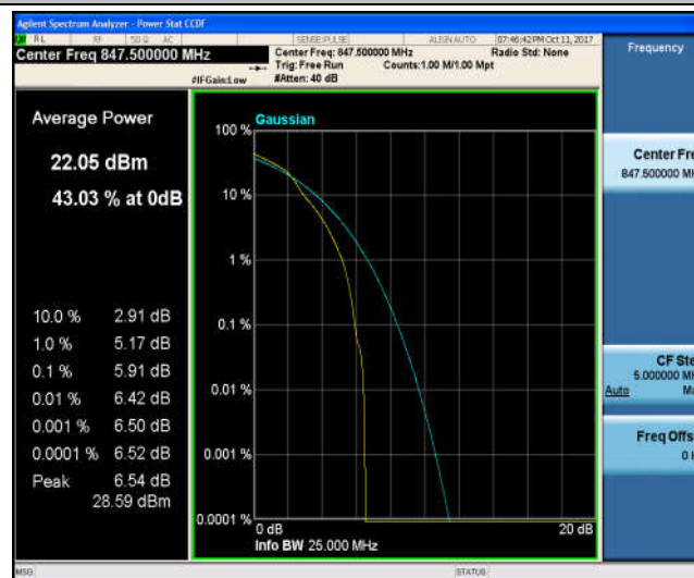
Band5_3MHz_QPSK_20635_15RB#0_5.74_13_PASS
