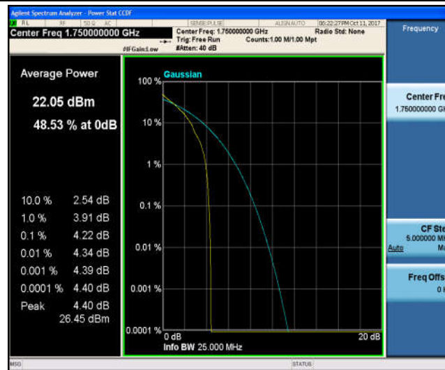
Band4_10MHz_16QAM_20350_1RB#0_5.26_13_PASS
