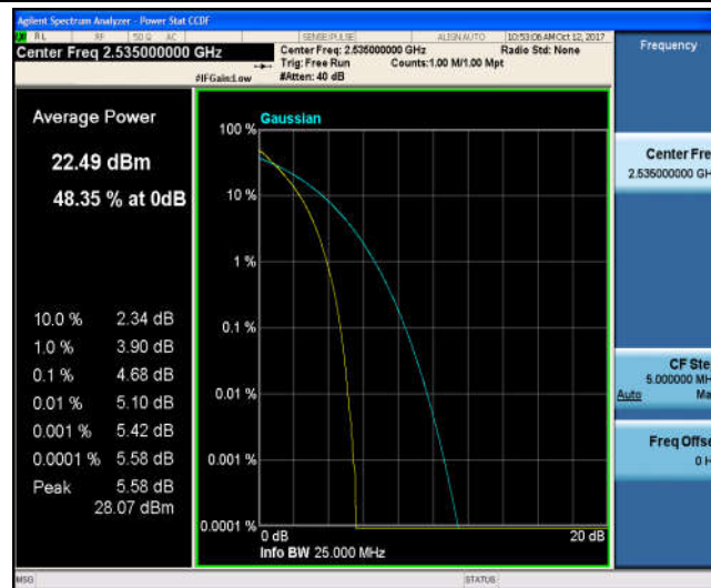
Band7_20MHz_16QAM_21100_100RB#0_5.54_13_PASS
