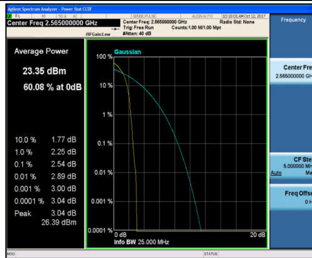
Band7_10MHz_16QAM_21400_1RB#0_3.67_13_PASS
