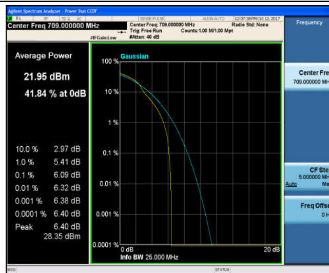
Band17_10MHz_QPSK_23780_50RB#0_5.77_13_PASS
