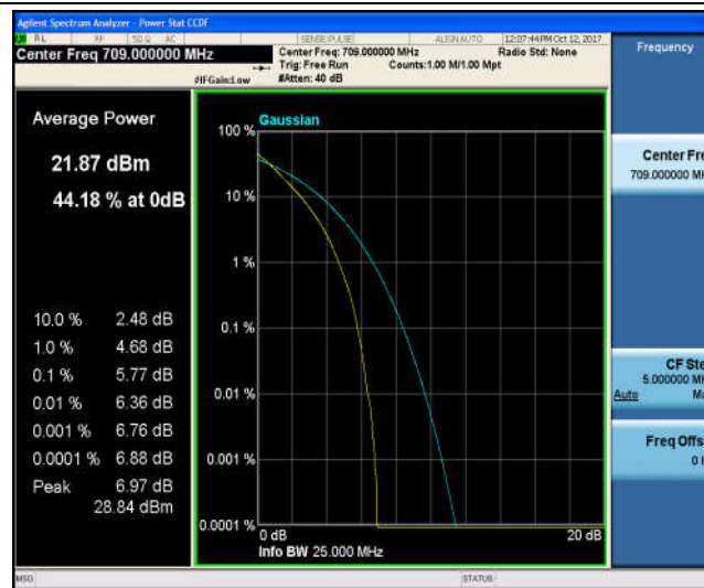
Band17_10MHz_16QAM_23780_50RB#0_6.60_13_PASS
