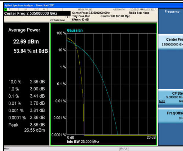
Band7_20MHz_QPSK_21100_100RB#0_4.68_13_PASS
