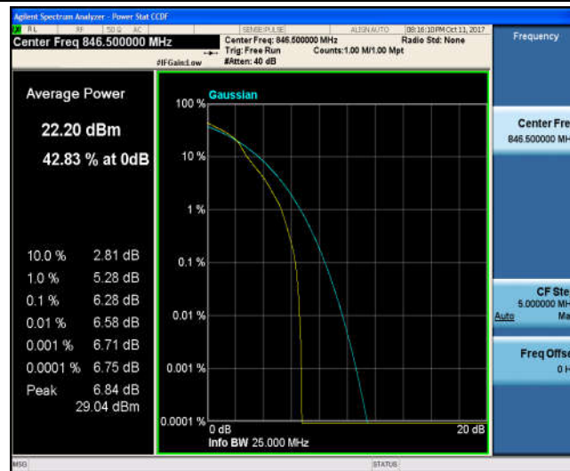
Band5_5MHz_QPSK_20625_25RB#0_5.80_13_PASS
