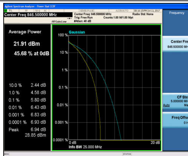
Band5_5MHz_16QAM_20625_25RB#0_6.51_13_PASS
