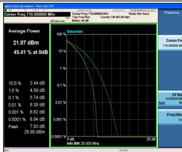
Band17_10MHz_16QAM_23790_50RB#0_6.52_13_PASS
