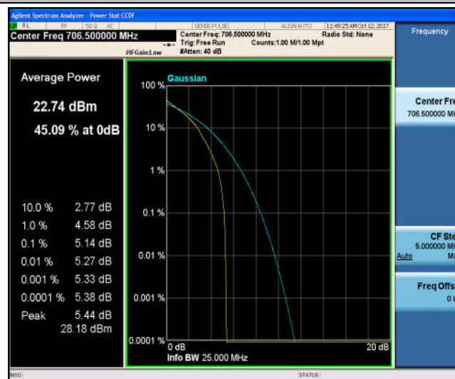
Band17_5MHz_16QAM_23755_1RB#0_5.88_13_PASS
