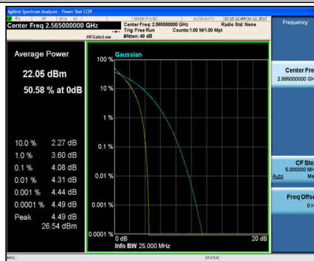
Band7_10MHz_16QAM_21400_50RB#0_4.99_13_PASS
