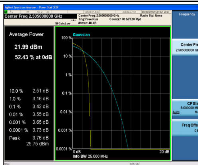
Band7_10MHz_QPSK_20800_50RB#0_4.37_13_PASS
