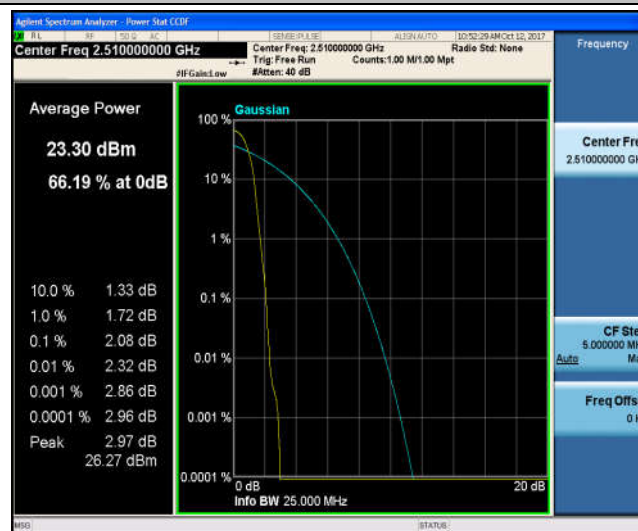
Band7_20MHz_16QAM_20850_1RB#0_3.05_13_PASS
