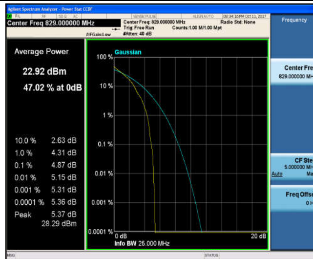
Band5_10MHz_16QAM_20450_1RB#0_5.85_13_PASS
