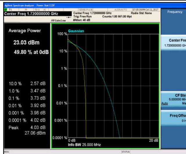
Band4_20MHz_16QAM_20050_1RB#0_4.70_13_PASS
