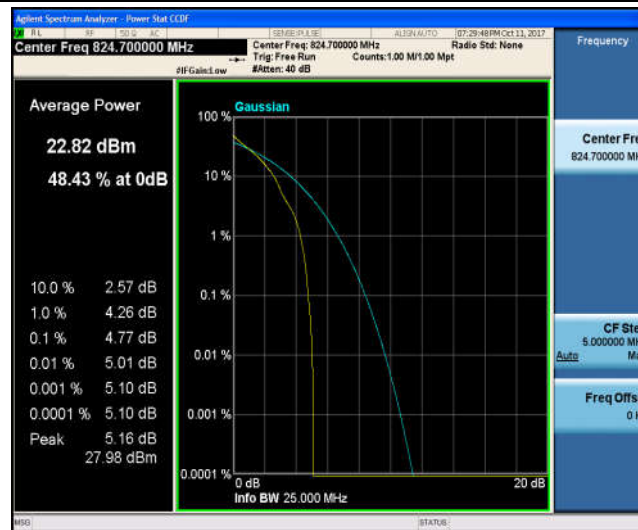
Band5_1.4MHz_16QAM_20407_1RB#0_5.81_13_PASS
