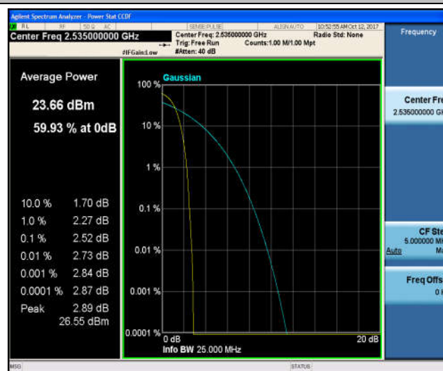
Band7_20MHz_16QAM_21100_1RB#0_3.41_13_PASS
