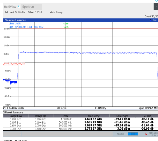
1-N77-3700-3980--30-100-L-3-DFT-PI2BPSK-Out er_Full-270@0-Ant0-PASS-see graph
