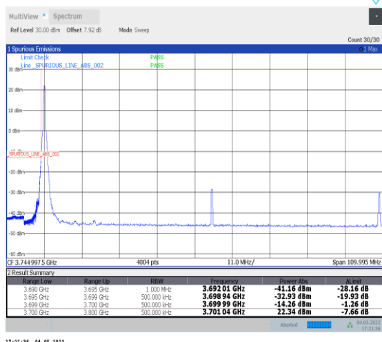
1-N77-3700-3980--30-100-L-1-DFT-PI2BPSK-Edge_1 RB_Left-1@0-Ant0-PASS-see graph
