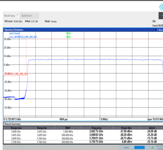
1-N77-3700-3980-PC1-30-60-L-3-DFT-PI2BPSK-O uter_Full-162@0-Ant0-1--PASS-see graph
