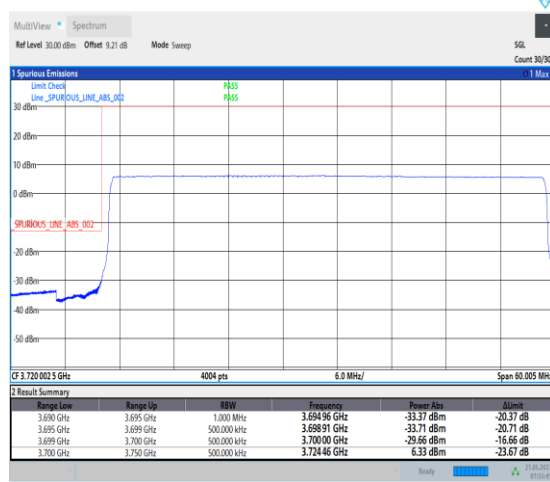
1-N77-3700-3980-PC1-30-50-L-6-CP-QPSK-Outer_Full-133@0-Ant0-1--PASS-see graph
