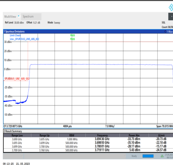
1-N77-3700-3980-PC1-30-60-L-6-CP-QPSK-Outer_ Full-162@0-Ant0-1--PASS-see graph
