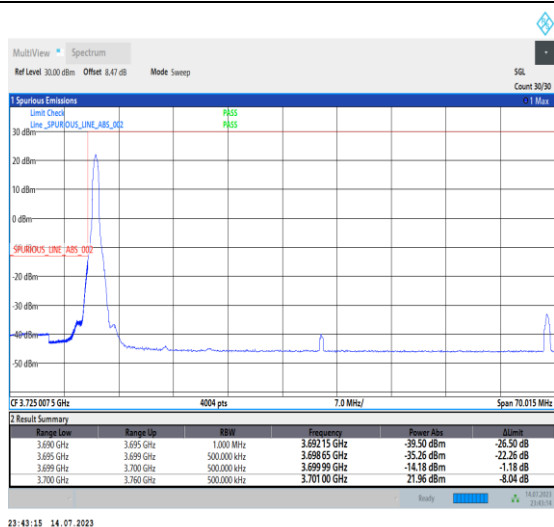
1-N77-3700-3980-PC1-30-60-L-1-DFT-PI2BPSK-Edg e_1RB_Left-1@0-Ant0-1--PASS-see graph
