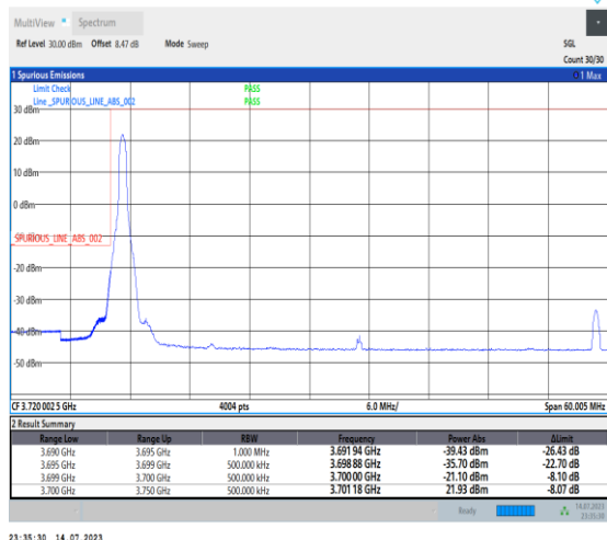
1-N77-3700-3980-PC1-30-50-L-1-DFT-PI2BPSK-Edg_e_1RB_Left-1@0-Ant0-1--PASS-see graph
