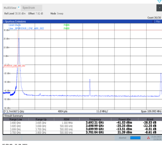
1-N77-3700-3980--30-100-L-4-CP-QPSK-Edge_1RB_ Left-1@0-Ant0-PASS-see graph
