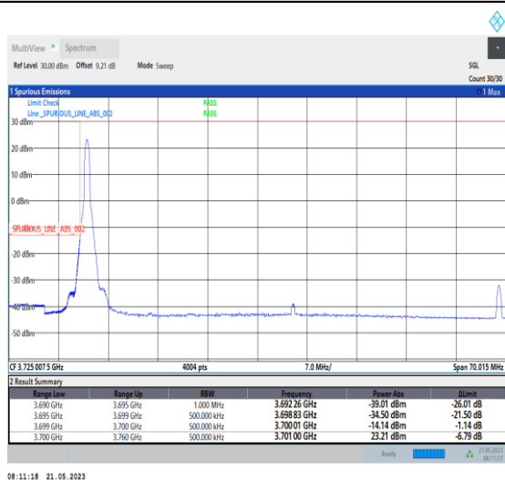
1-N77-3700-3980-PC1-30-60-L-4-CP-QPSK-Edge_1 RB_Left-1@0-Ant0-1--PASS-see graph
