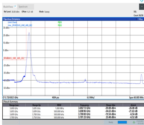
1-N77-3700-3980-PC1-30-50-L-4-CP-QPSK-Edge_1RB_Left-1@0-Ant0-1--PASS-see graph
