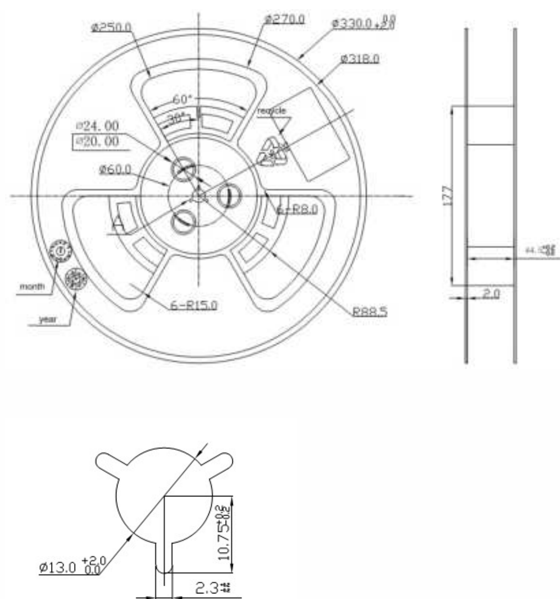
Figure 35: Reel Detail
