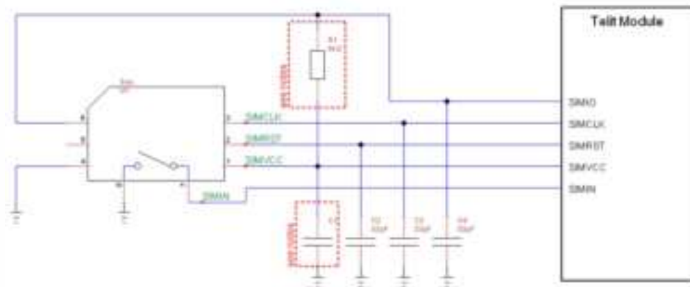
Figure 30: SIM Schematics
