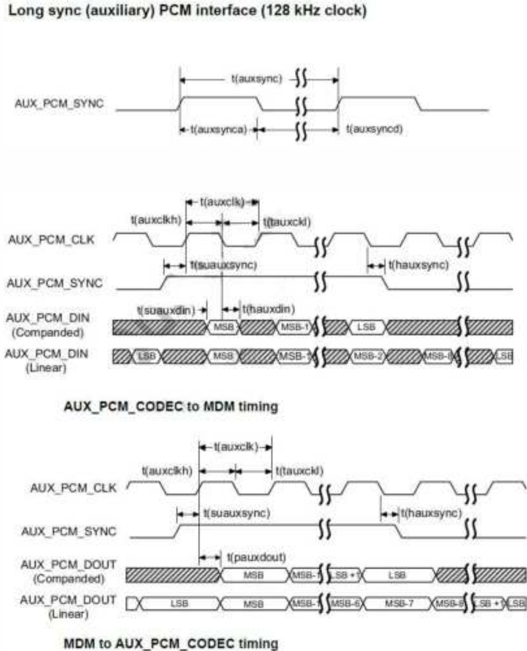
Figure 18: Auxiliary PCM Timing
