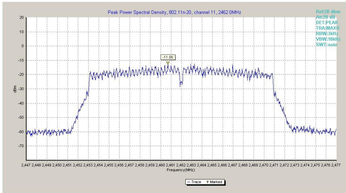
Fig.A.3.9 Power Spectral Density (802.11n-HT20, Ch 11)
