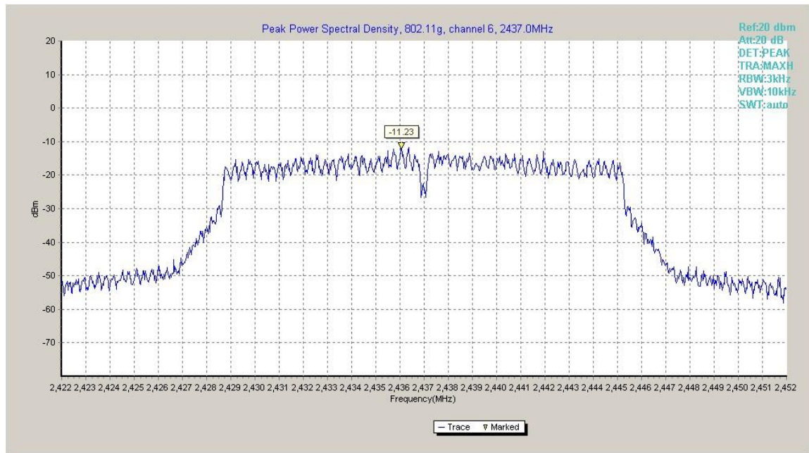
Fig.A.3.5 Power Spectral Density (802.11g, Ch 6)
