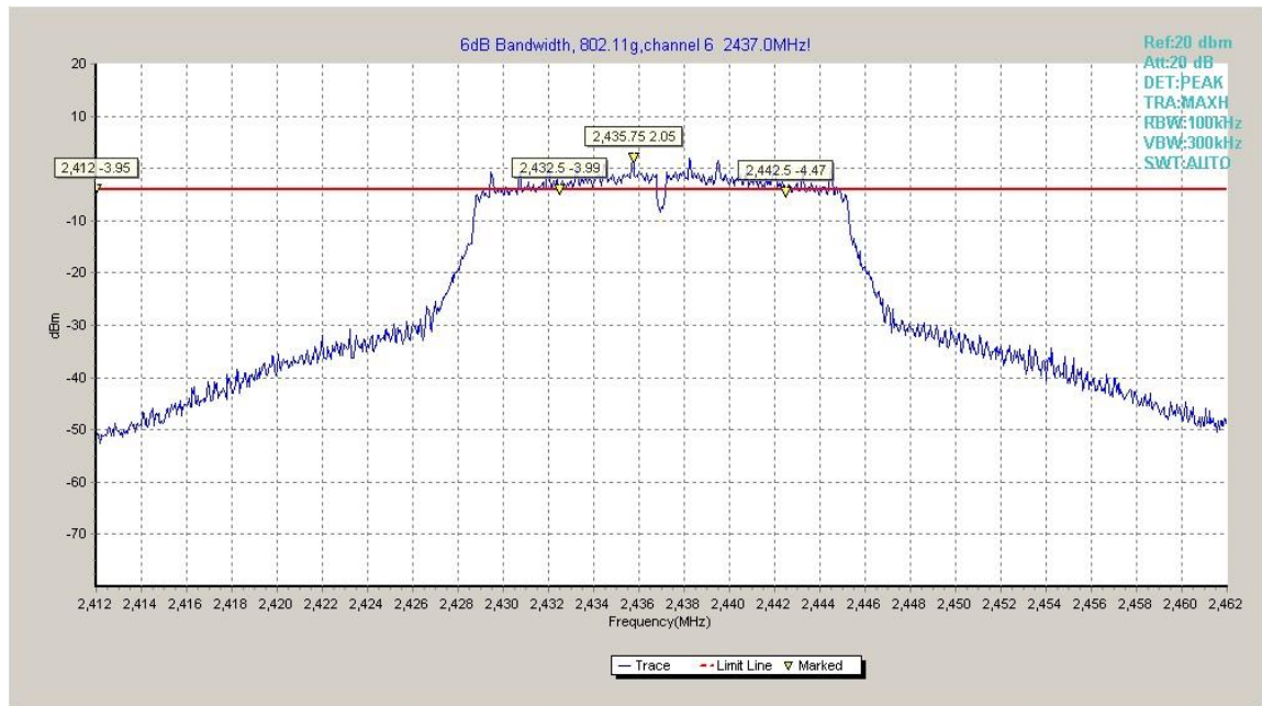
Fig.A.4.5 Occupied 6dB Bandwidth (802.11g, Ch 6)
