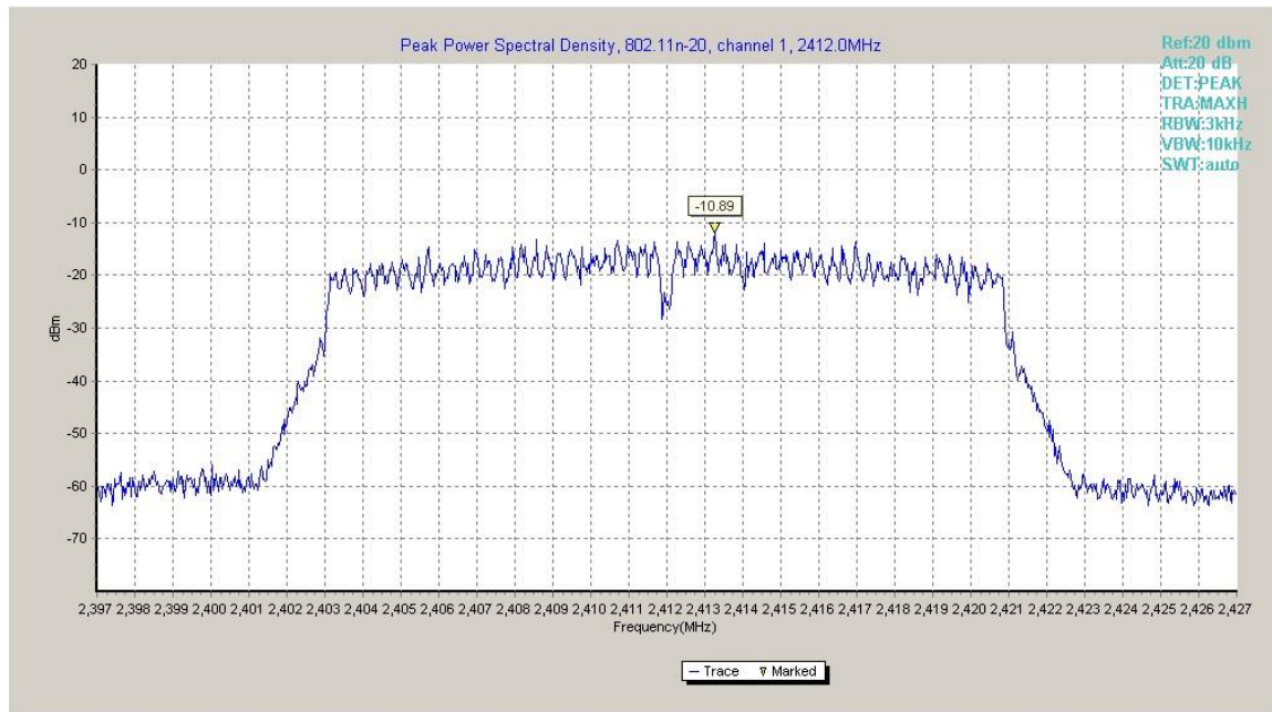
Fig.A.3.7 Power Spectral Density (802.11n-HT20, Ch 1)
