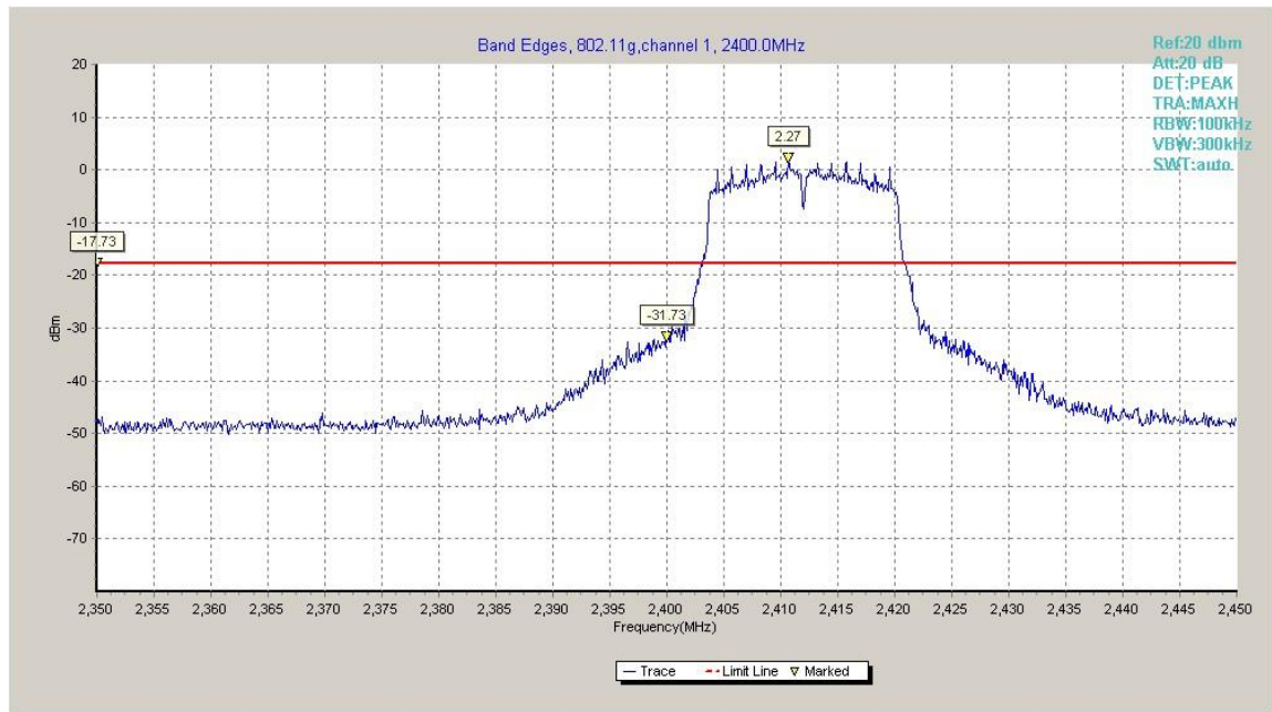
Fig.A.5.3 Band Edges (802.11g, Ch 1)
