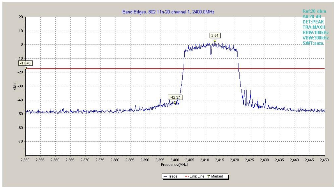
Fig.A.5.5 Band Edges (802.11n-HT20, Ch 1)
