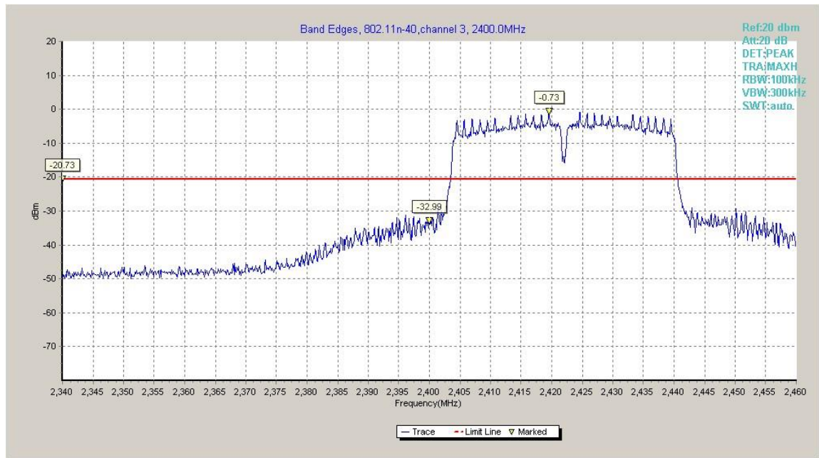
Fig.A.5.7 Band Edges (802.11n-HT40, Ch 3)
