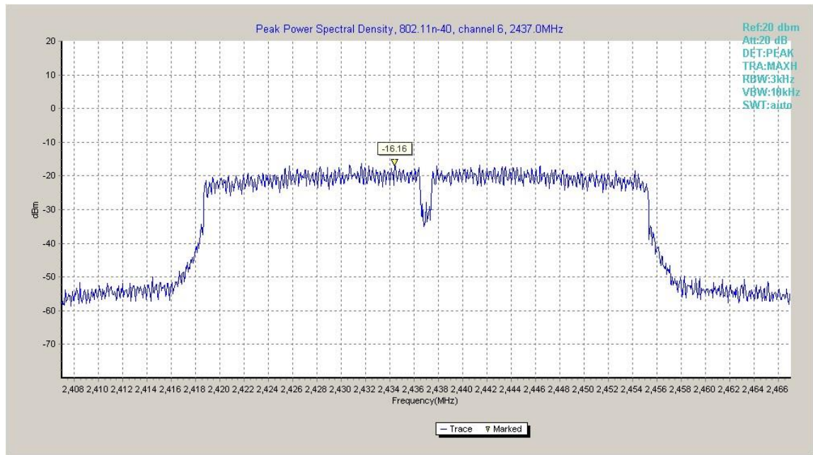
Fig.A.3.11 Power Spectral Density (802.11n-HT40, Ch 6)
