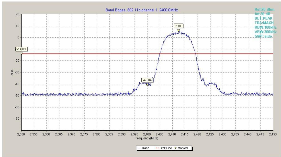
Fig.A.5.1 Band Edges (802.11b, Ch 1)
