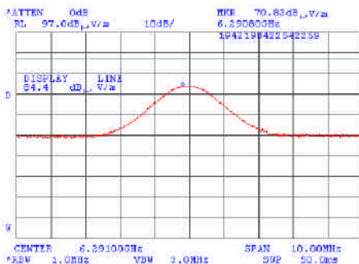
Plot 4.5.10 Radiated emission measurements at the 10 th harmonic
