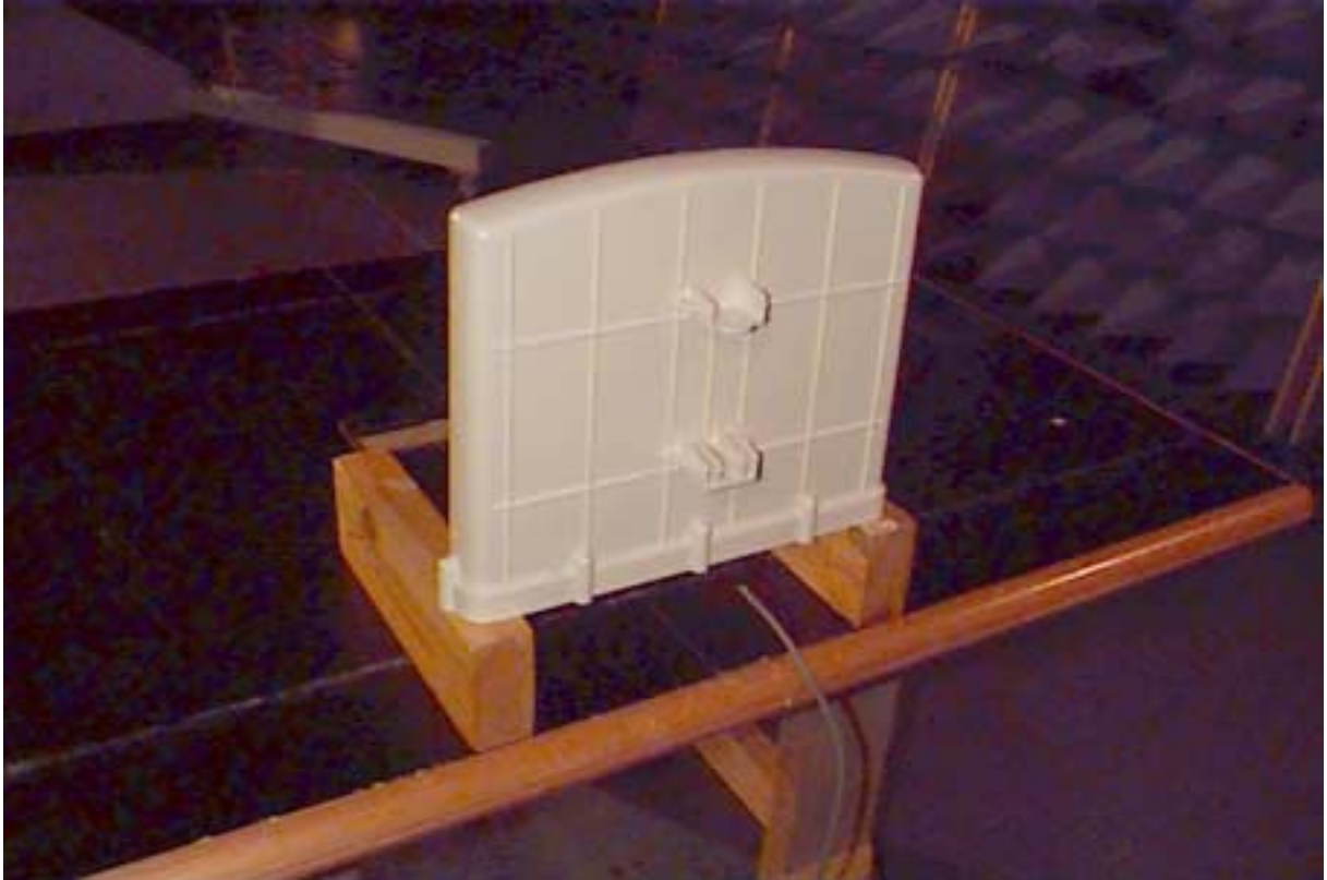
Photograph 4.8.3 Setup for radiated emission measurements, EUT view
