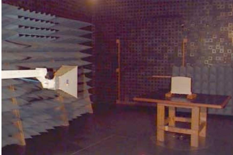
Photograph 4.5.3 Setup for spurious emission field strength measurements in 1 to 6.5 GHz band, general view
