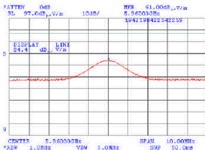
Plot 4.5.28 Radiated emission measurements at the 9 th harmonic
