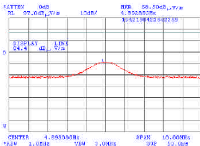
Plot 4.5.8 Radiated emission measurements at the 8 th harmonic
