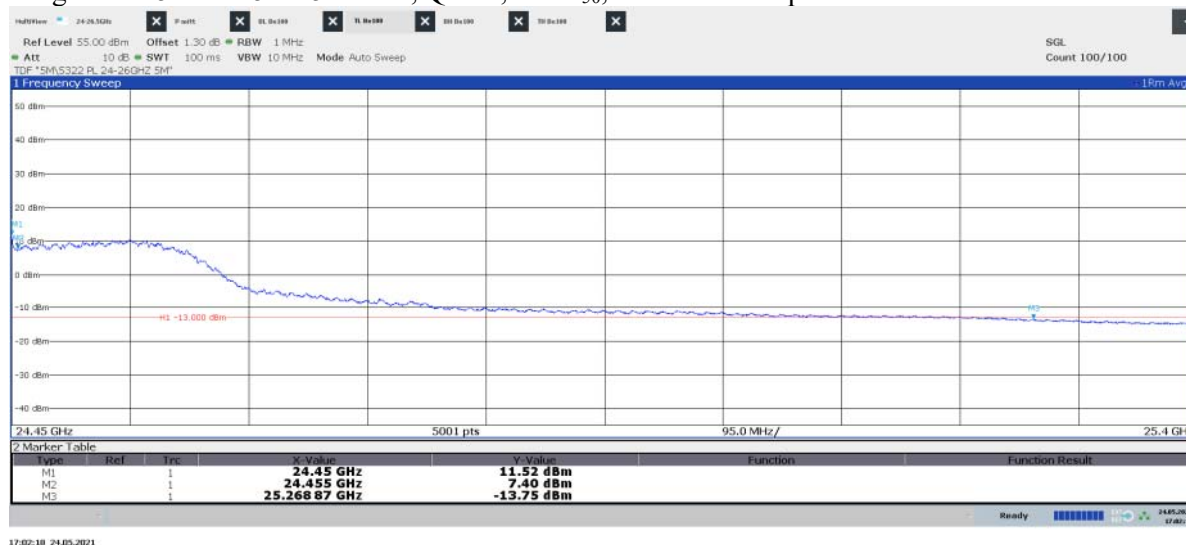
Diagram 2.15d: 24.45 – 25.4 GHz, QPSK, TimL 50 , EIRP Vertical polarization
