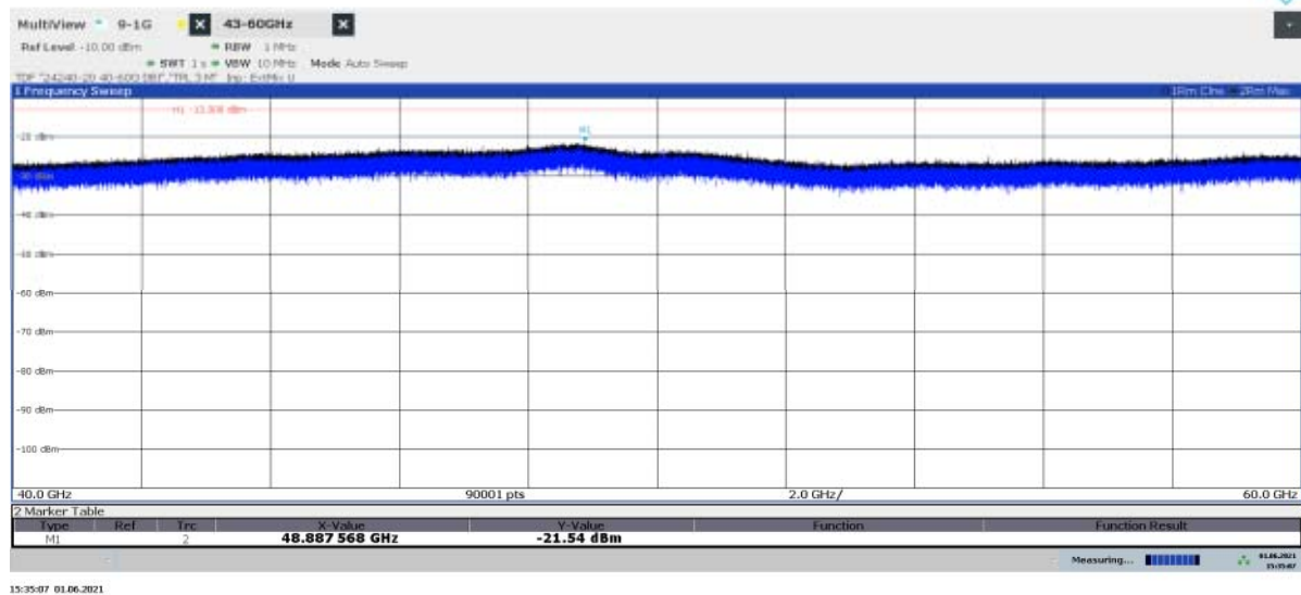
Diagram 2.29a: 40 – 60 GHz, QPSK, BT8 50 , EIRP Horizontal polarization
