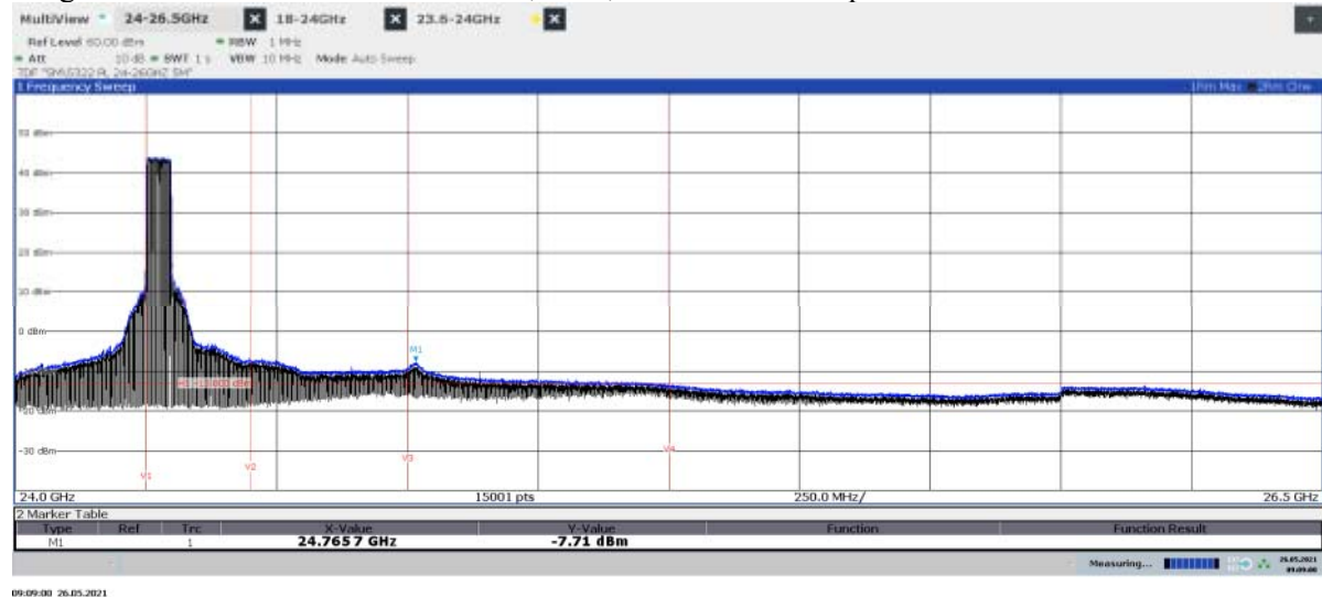
Diagram 2.12a: Pre scan 24 – 26.5 GHz, BL 50 , EIRP Horizontal polarization
