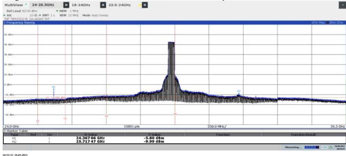
Diagram 2.18a: Pre scan 24 – 26.5 GHz, TH 50 , EIRP Horizontal polarization
