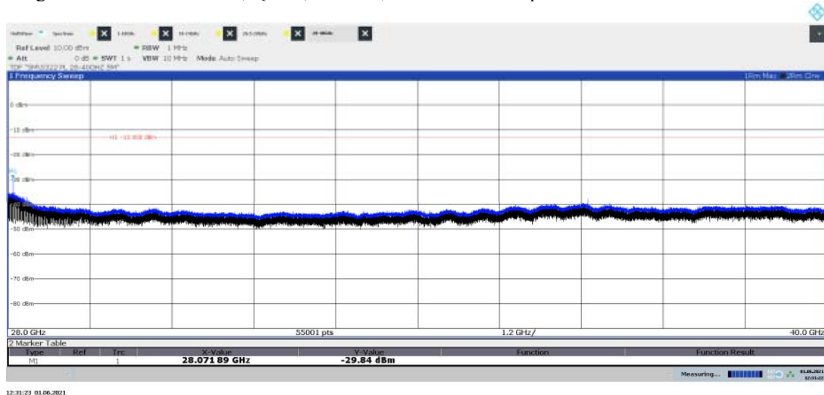
Diagram 2.27a: 28 – 40 GHz, QPSK, BMT8 50 , EIRP Horizontal polarization
