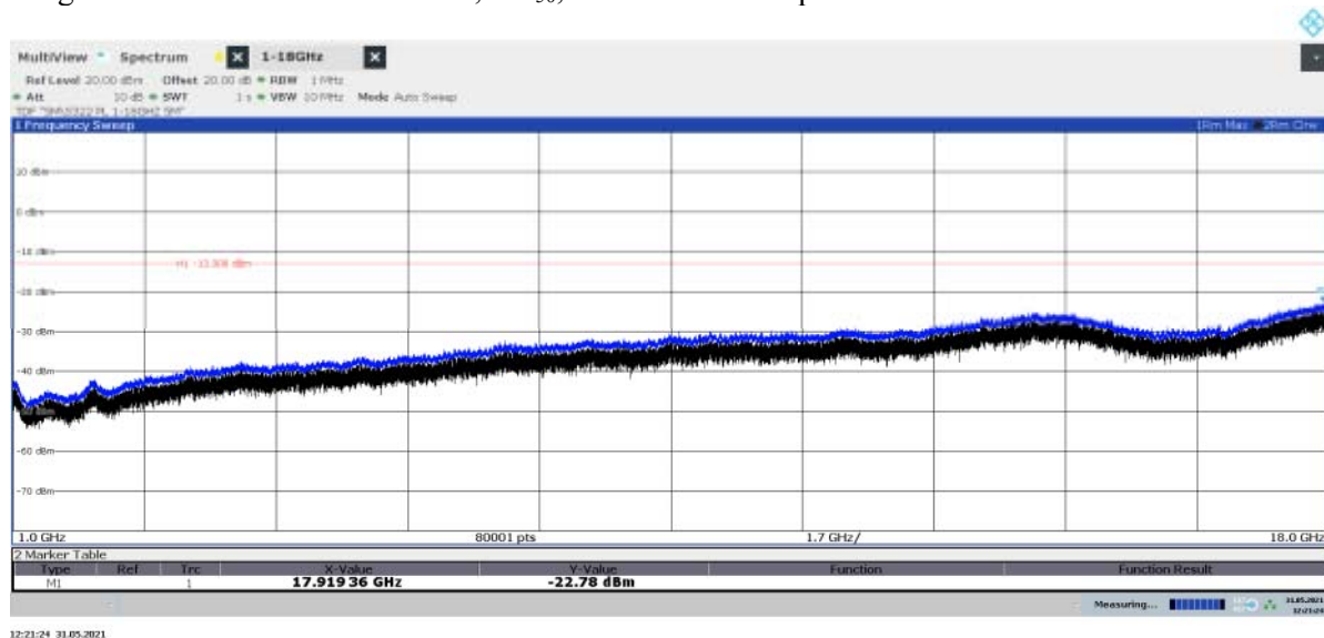
Diagram 2.4a: Pre scan 1 – 18 GHz, BH 50 , EIRP Horizontal polarization
