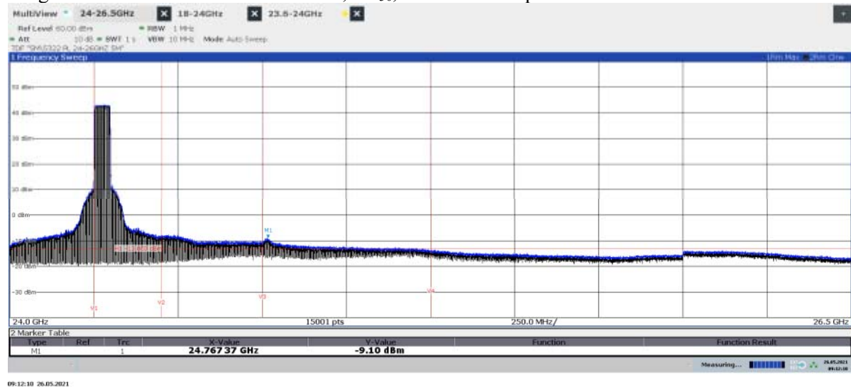
Diagram 2.12b: Pre scan 24 – 26.5 GHz, BL 50 , EIRP Vertical polarization
