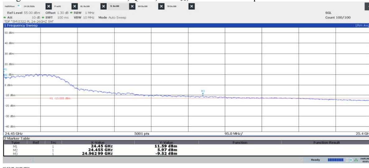
Diagram 2.15c: 24.45 – 25.4 GHz, QPSK, TimL 50 , EIRP Horizontal polarization
