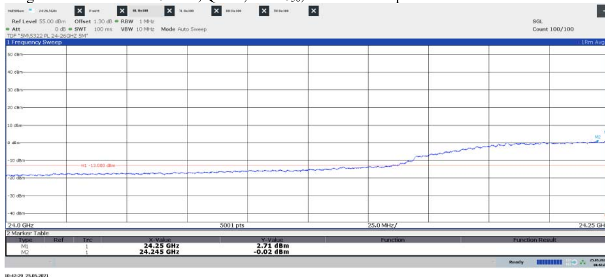
Diagram 2.21d: 24 – 24.25 GHz, QPSK, BMT8 50 , EIRP Vertical polarization
