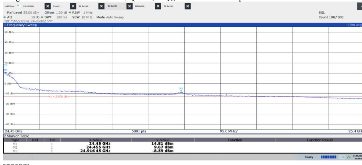
Diagram 2.14c: 24.45 – 25.4 GHz, QPSK, TL 50 , EIRP Horizontal polarization
