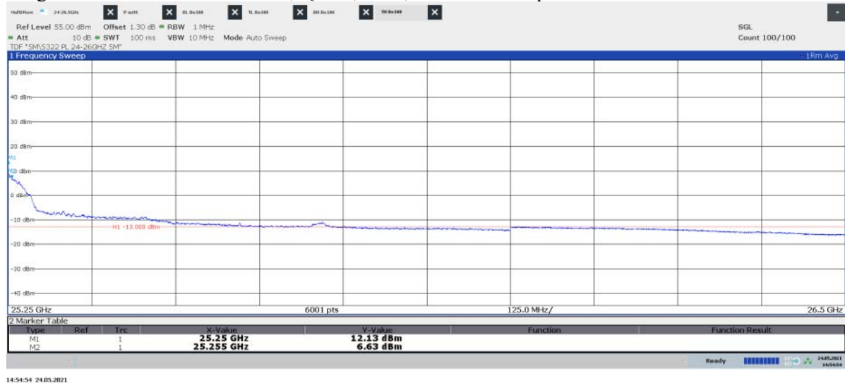
Diagram 2.18d: 25.25 – 26.5 GHz, QPSK, TH 50 , EIRP Vertical polarization
