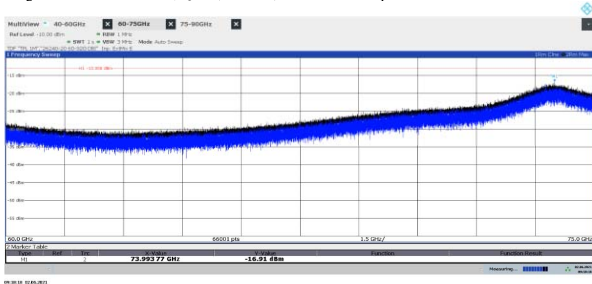
Diagram 2.33a: 60 – 75 GHz, QPSK, BMT8 50 , EIRP Horizontal polarization
