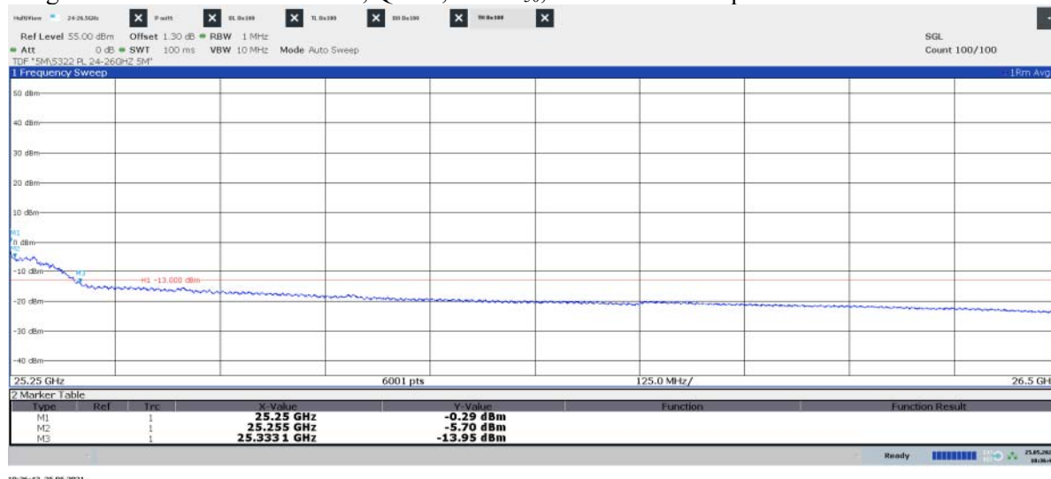
Diagram 2.21e: 25.25 – 26.5 GHz, QPSK, BMT8 50 , EIRP Horizontal polarization
