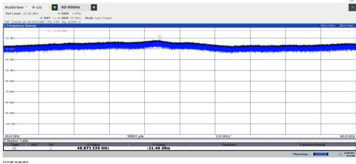
Diagram 2.29b: 40 – 60 GHz, QPSK, BT8 50 , EIRP Vertical polarization
