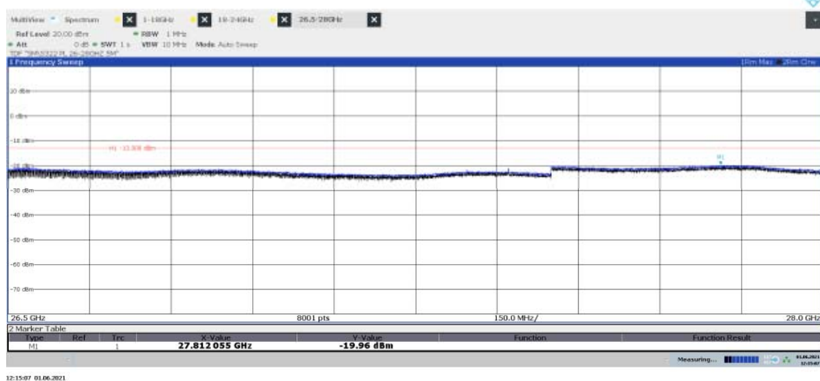
Diagram 2.23b: 26.5 – 28 GHz, QPSK, BT8 50 , EIRP Vertical polarization
