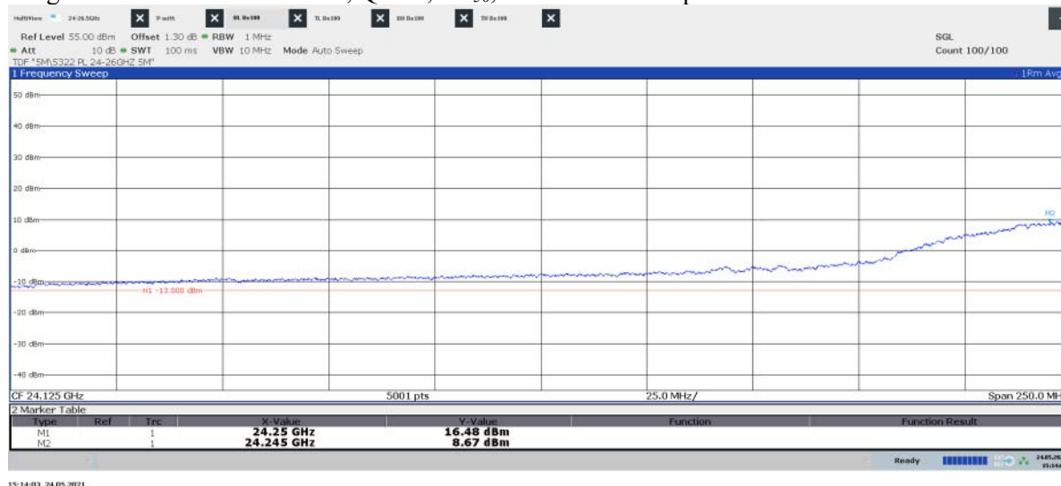
Diagram 2.12c: 24 – 24.25 GHz, QPSK, BL 50 , EIRP Horizontal polarization
