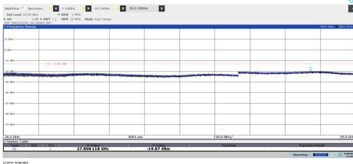
Diagram 2.24b: 26.5 – 28 GHz, QPSK, BMT8 50 , EIRP Vertical polarization
