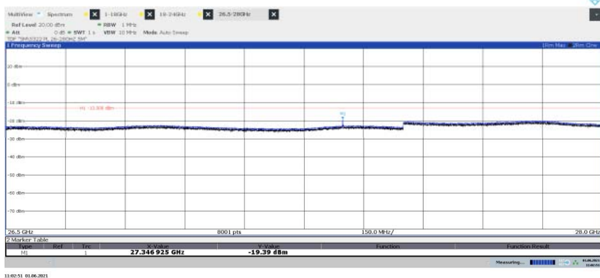
Diagram 2.22b: 26.5 – 28 GHz, QPSK, BL 50 , EIRP Vertical polarization
