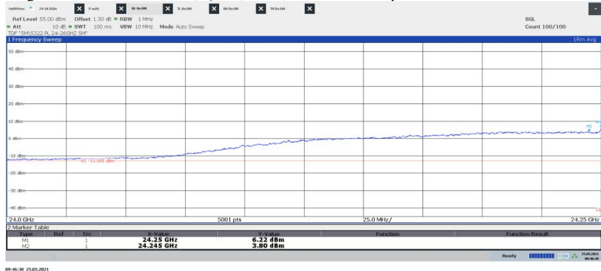
Diagram 2.20c: 24 – 24.25 GHz, QPSK, BT8 50 , EIRP Horizontal polarization
