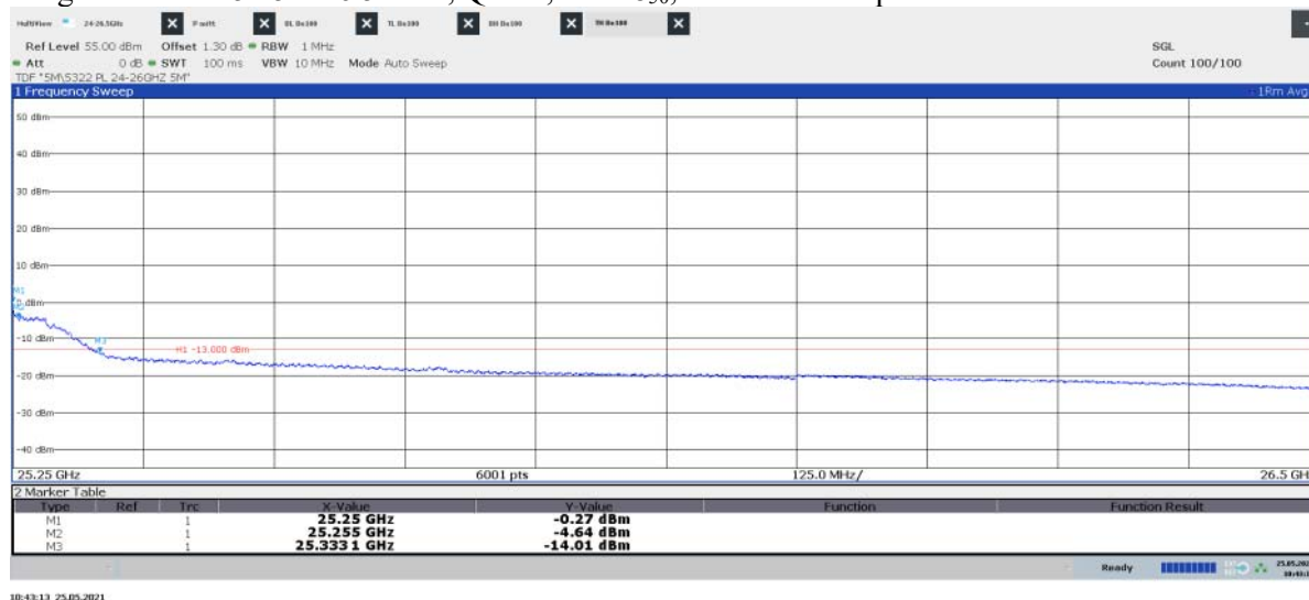
Diagram 2.21f: 25.25 – 26.5 GHz, QPSK, BMT8 50 , EIRP Vertical polarization
