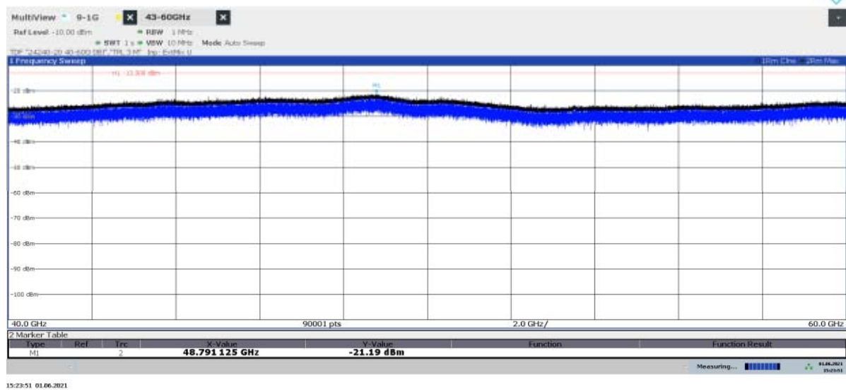
Diagram 2.28b: 40 – 60 GHz, QPSK, BH 50 , EIRP Vertical polarization
