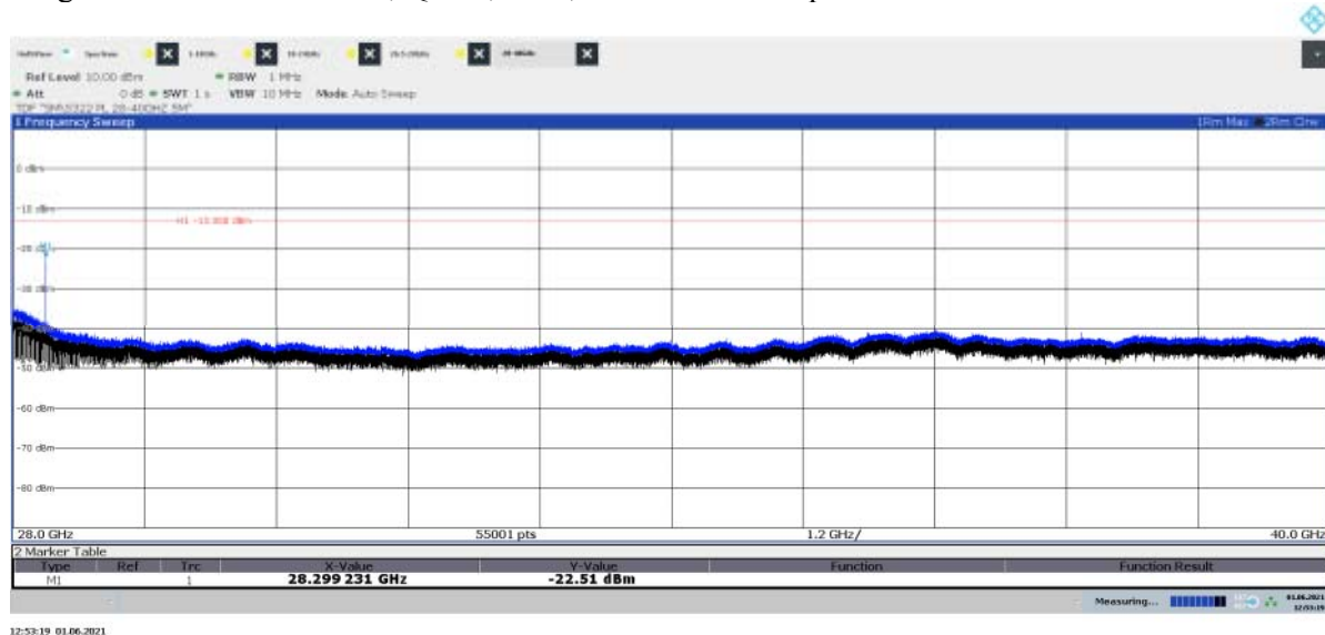
Diagram 2.25a: 28 – 40 GHz, QPSK, TH 50 , EIRP Horizontal polarization
