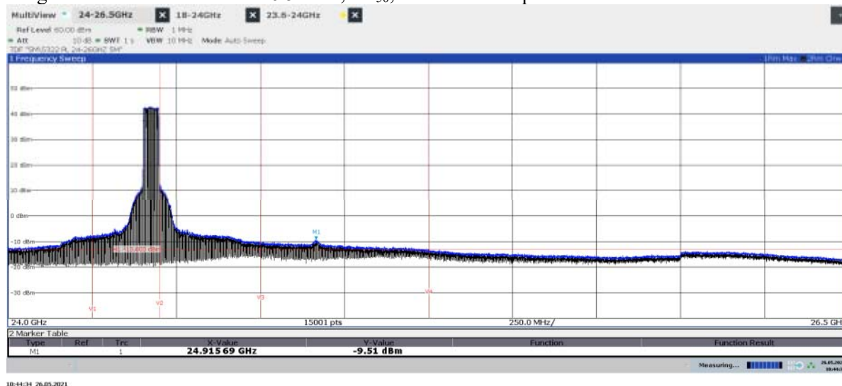
Diagram 2.14b: Pre scan 24 – 26.5 GHz, TL 50 , EIRP Vertical polarization
