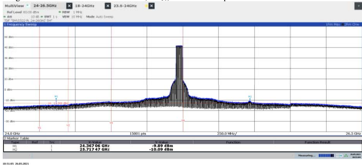
Diagram 2.18b: Pre scan 24 – 26.5 GHz, TH 50 , EIRP Vertical polarization
