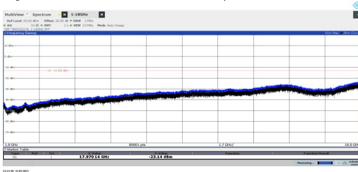
Diagram 2.6a: Pre scan 1 – 18 GHz, BMT 50 , EIRP Horizontal polarization
