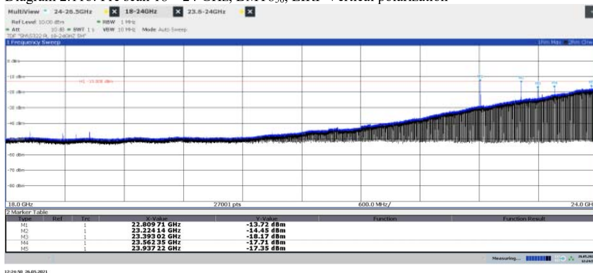
Diagram 2.11b: Pre scan 18 – 24 GHz, BMT8 50 , EIRP Vertical polarization
