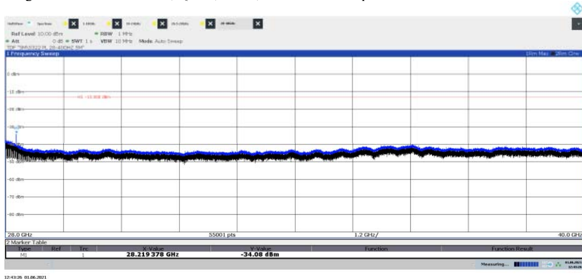
Diagram 2.26a: 28 – 40 GHz, QPSK, BT8 50 , EIRP Horizontal polarization
