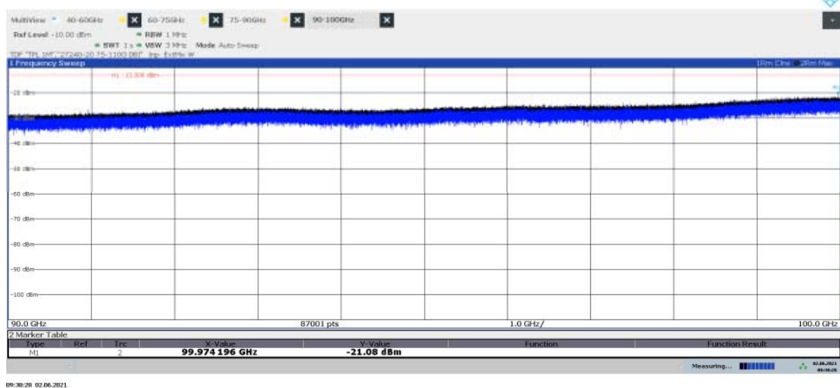
Diagram 2.39b: 90 – 100 GHz, QPSK, BMT8 50 , EIRP Vertical polarization
