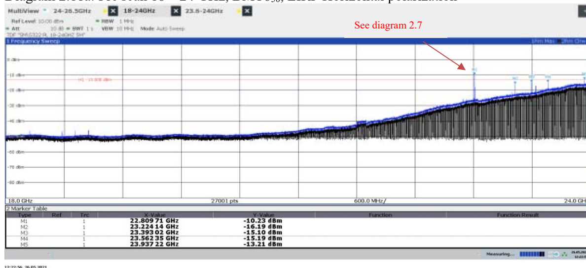
Diagram 2.11a: Pre scan 18 – 24 GHz, BMT8 50 , EIRP Horizontal polarization
