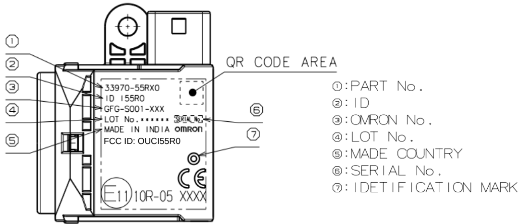
Figure 9.1 Label(marking) and I55R0 appearance
