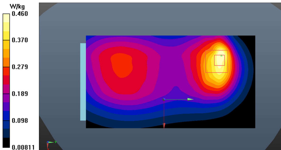
Fig.2 GSM850 Body
