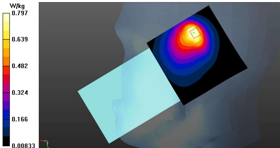
Fig.1 GSM850 Head
