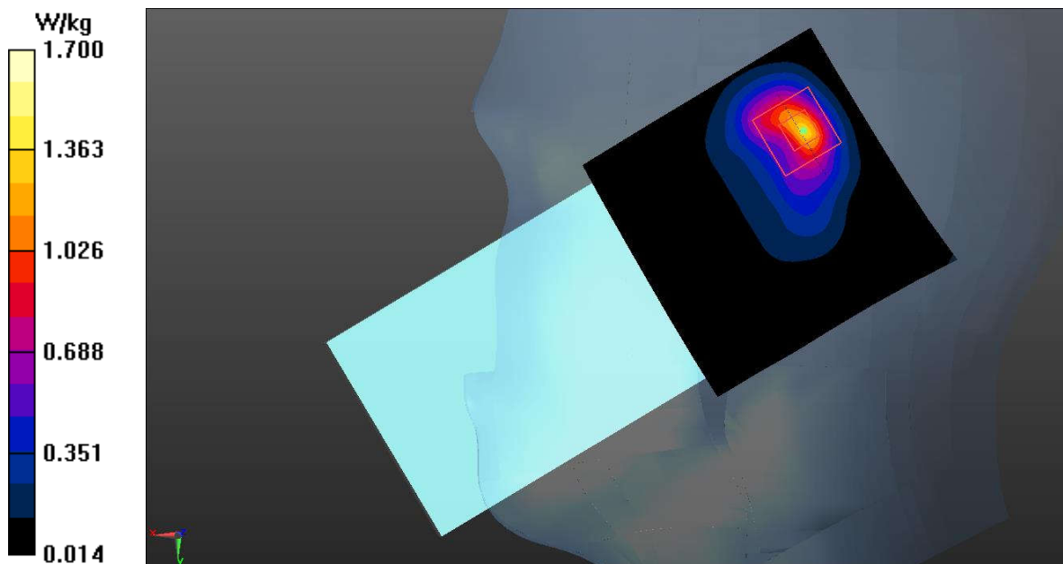
Fig.3 GSM1900 Head
