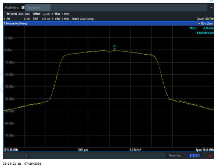
11AC20SISO_Ant2_5580
