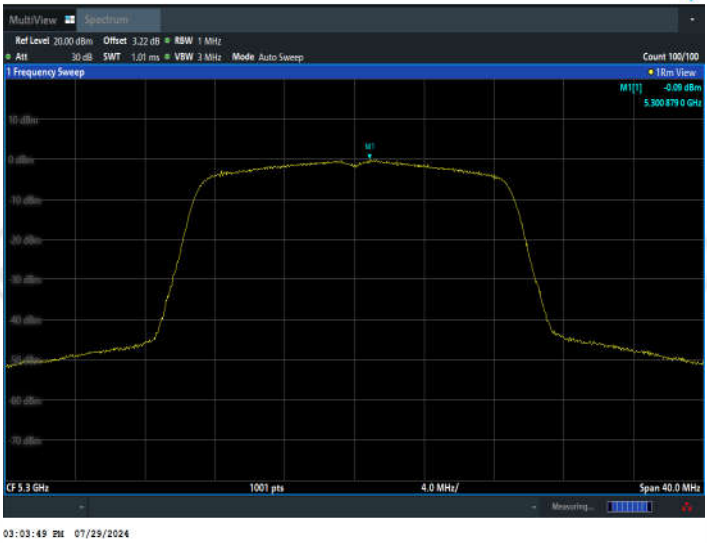
11AC20SISO_Ant2_5300
