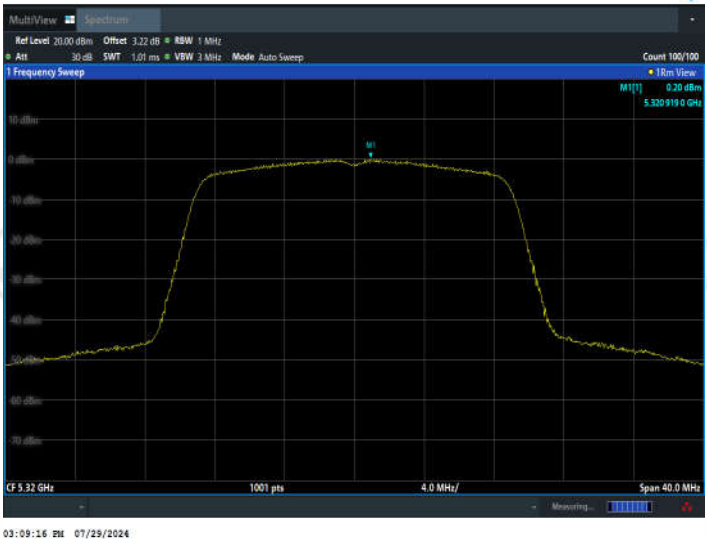
11AC20SISO_Ant2_5320
