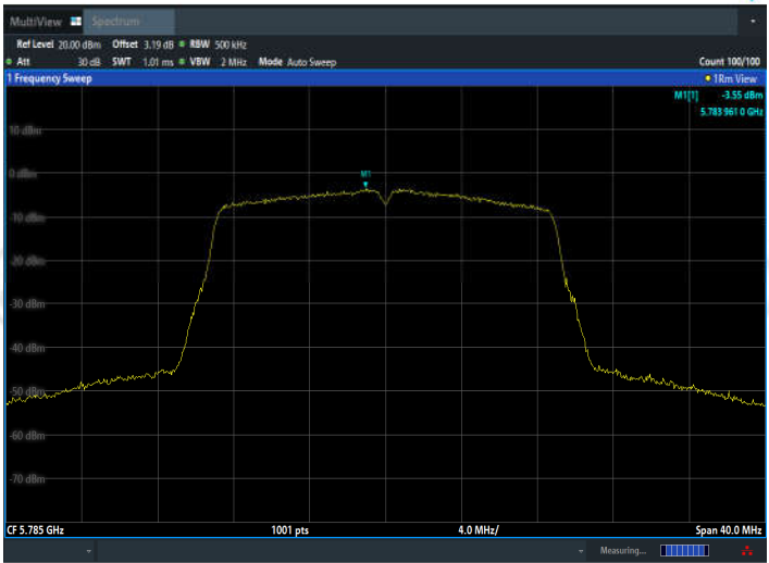
11AC20SISO_Ant2_5785
