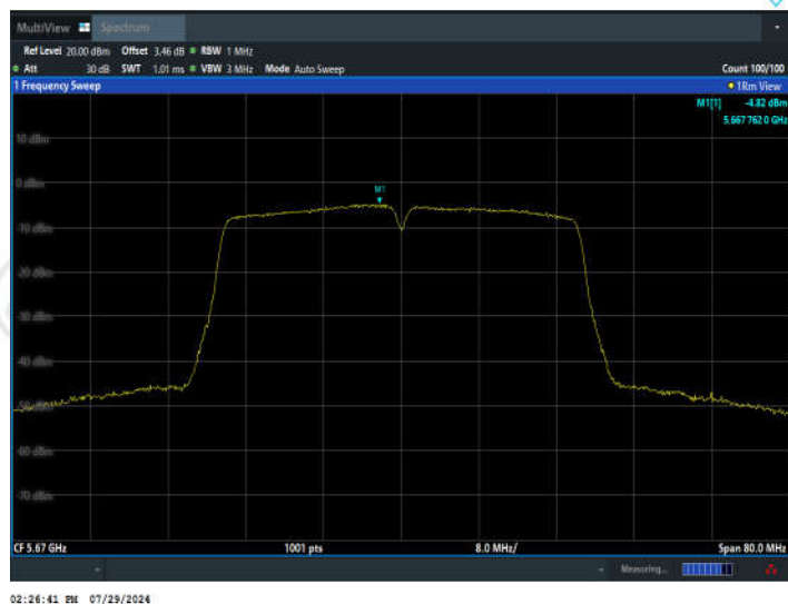
11N40SISO_Ant2_5670
