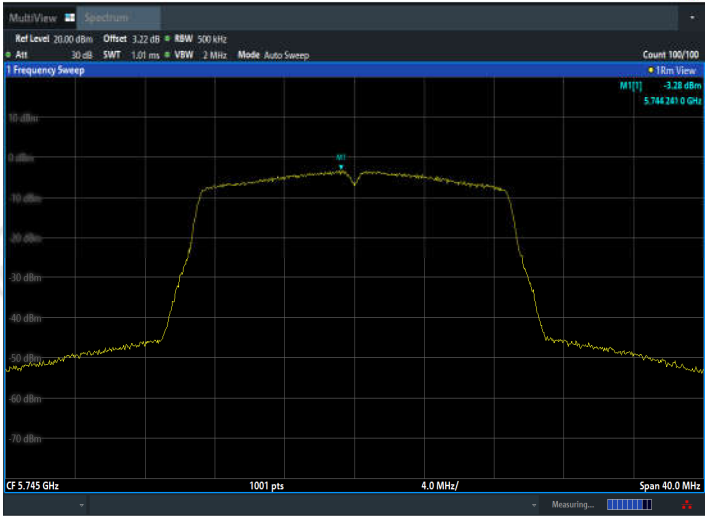
11AC20SISO_Ant2_5745
