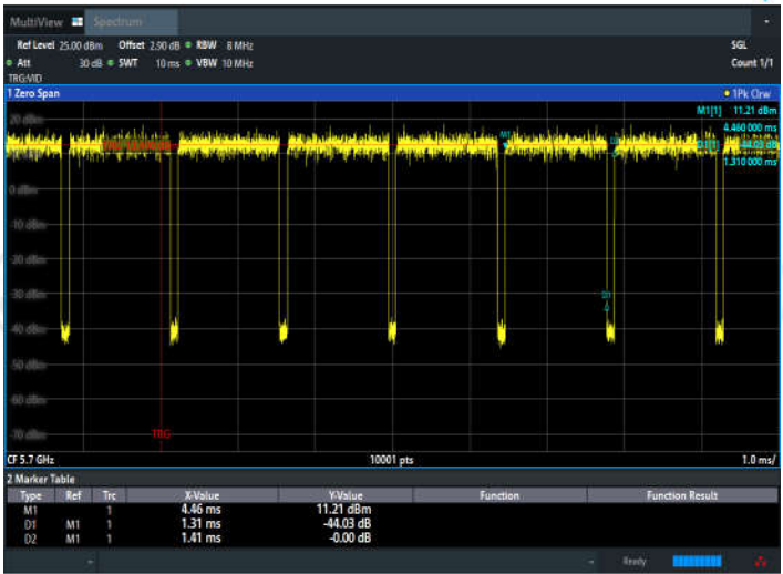
11AC20SISO_Ant2_5700
