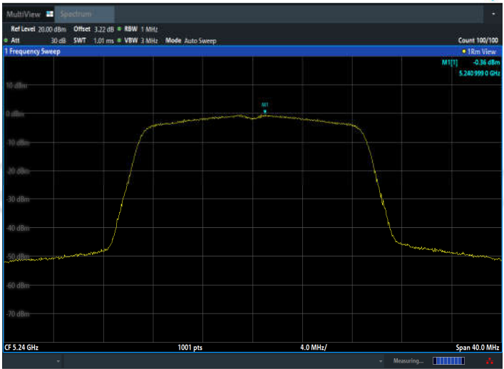
11AC20SISO_Ant2_5240
