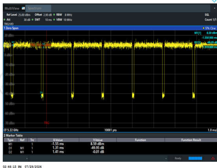
11AC20SISO_Ant2_5220
