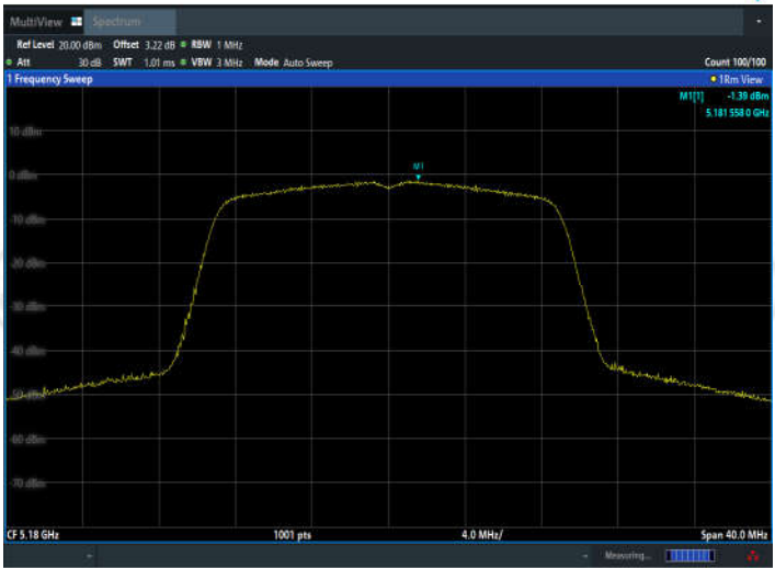
11N20SISO_Ant2_5180
