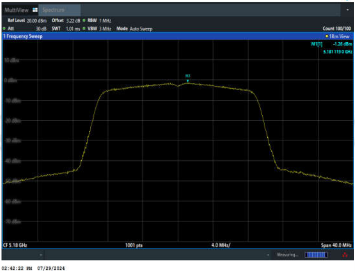
11AC20SISO_Ant2_5180
