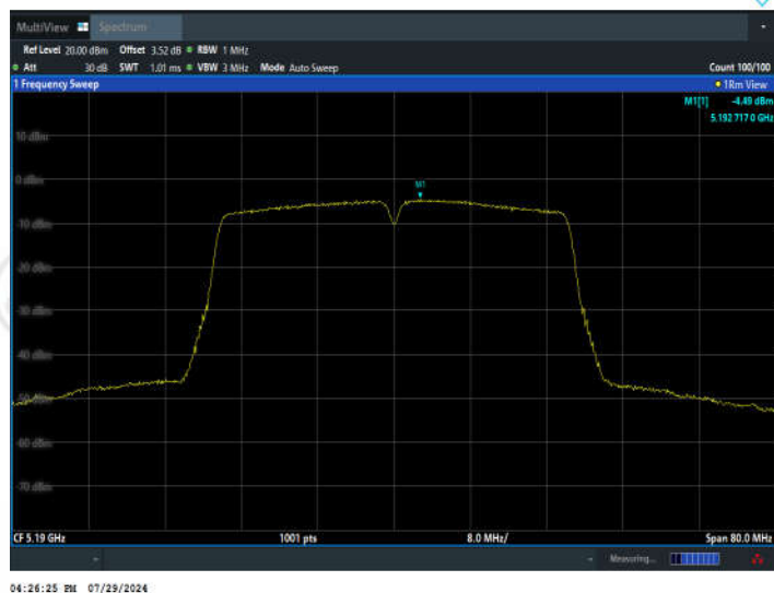
11AC40SISO_Ant2_5190
