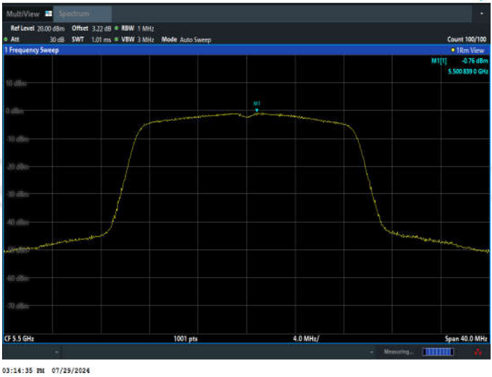
11AC20SISO_Ant2_5500
