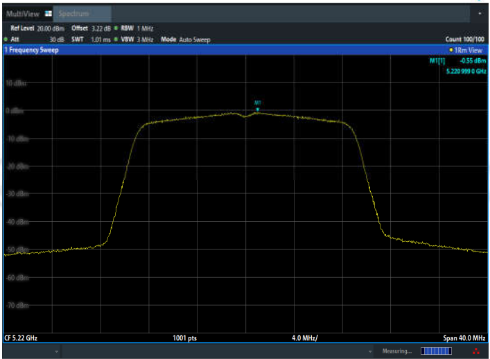
11AC20SISO_Ant2_5220
