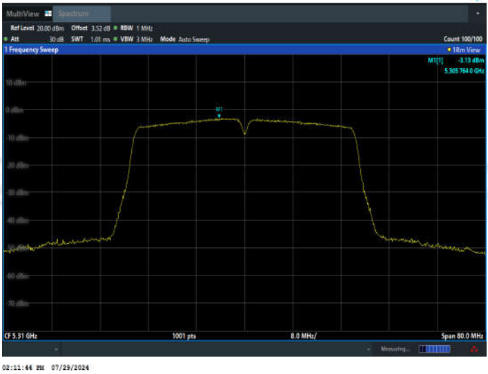
11N40SISO_Ant2_5310
