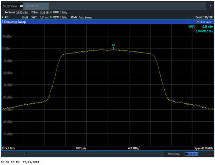
11AC20SISO_Ant2_5700
