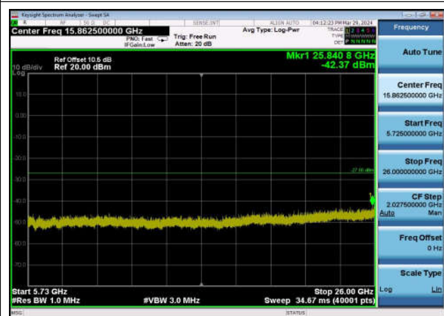
U-NII-2c ,Plot 3,5725MHz~26000MHz-802.11a(20MHz),5700MHz,Ant1
