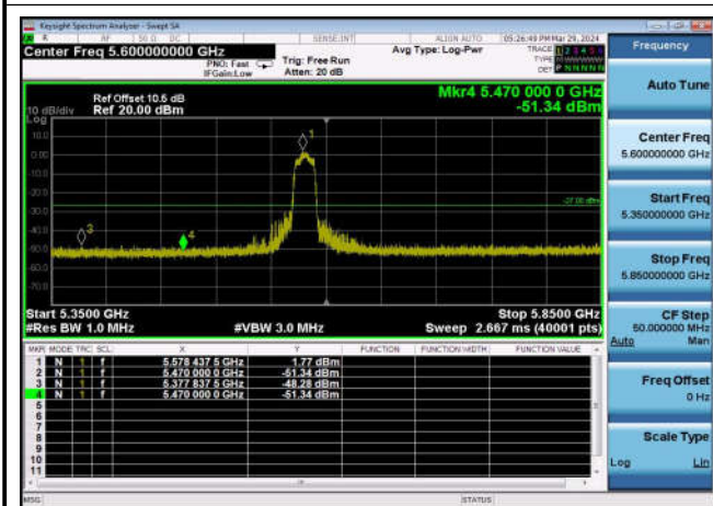
U-NII-2c ,Plot 1,Band Edge-802.11ac(20 MHz),5580MHz,Ant1
