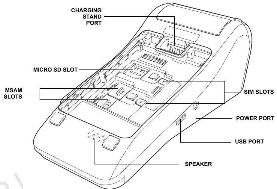
Figure 2 V400m Plus 3G Underside
