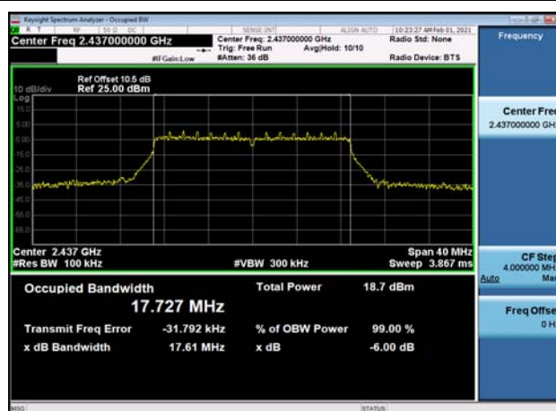
6dB Bandwidth-802.11n(HT20),2437MHz
