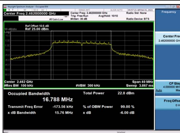
6dB Bandwidth-802.11g,2462MHz
