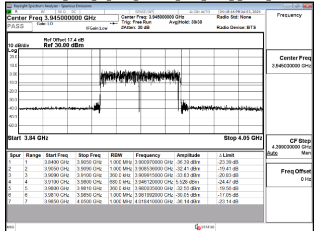
Band77-Part27_70MHz_CP_OFDM_SCS30kHz_QPSK_RB189_0_Chain0_CH663000
