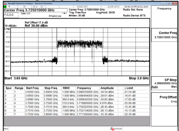
Band77-Part27_50MHz_CP_OFDM_SCS30kHz_QPSK_RB133_0_Chain0_CH656000
