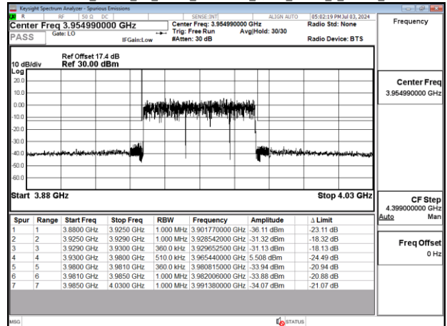
Band77-Part27_50MHz_CP_OFDM_SCS30kHz_QPSK_RB133_0_Chain0_CH663666
