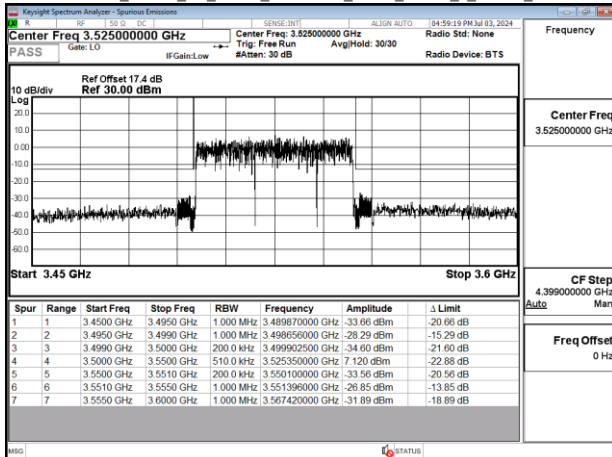
Band77-Part27_50MHz_CP_OFDM_SCS30kHz_QPSK_RB133_0_Chain0_CH635000
