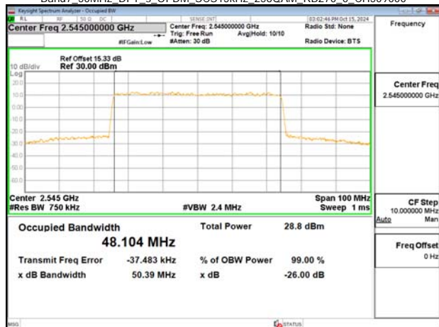
Band7_50MHz_DFT_s_OFDM_SCS15kHz_256QAM_RB270_0_CH509000
