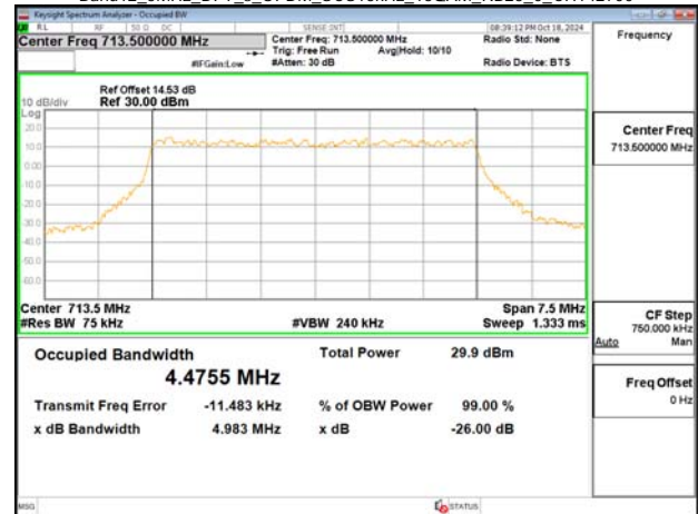
Band12_5MHz_DFT_s_OFDM_SCS15kHz_16QAM_RB25_0_CH142700
