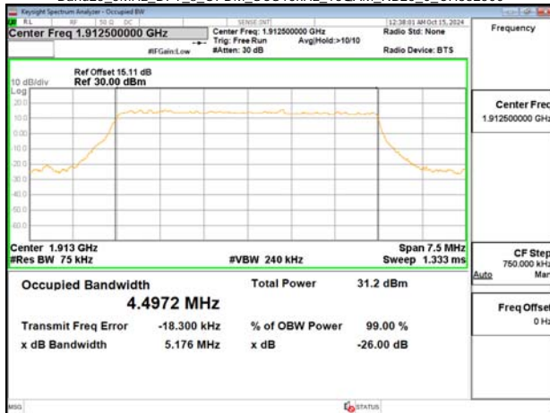
Band25_5MHz_DFT_s_OFDM_SCS15kHz_16QAM_RB25_0_CH382500
