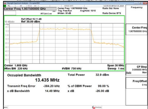
Band25_15MHz_DFT_s_OFDM_SCS15kHz_QPSK_RB75_0_CH381500
