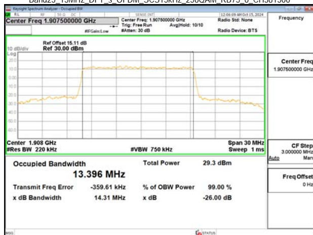
Band25_15MHz_DFT_s_OFDM_SCS15kHz_256QAM_RB75_0_CH381500
