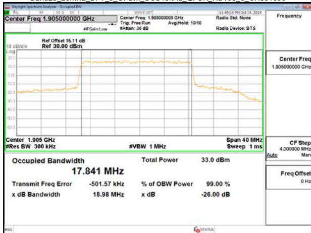
Band25_20MHz_DFT_s_OFDM_SCS15kHz_QPSK_RB100_0_CH381000
