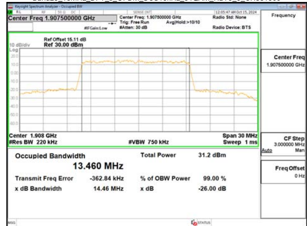
Band25_15MHz_DFT_s_OFDM_SCS15kHz_64QAM_RB75_0_CH381500
