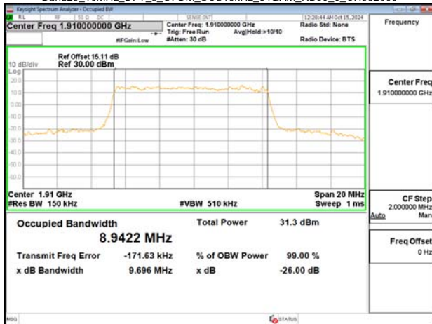
Band25_10MHz_DFT_s_OFDM_SCS15kHz_64QAM_RB50_0_CH382000
