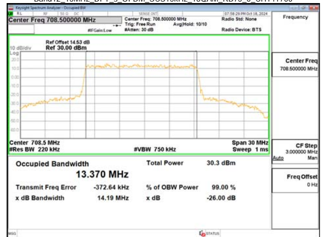
Band12_15MHz_DFT_s_OFDM_SCS15kHz_16QAM_RB75_0_CH141700
