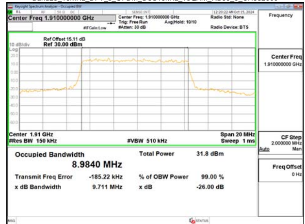
Band25_10MHz_DFT_s_OFDM_SCS15kHz_16QAM_RB50_0_CH382000
