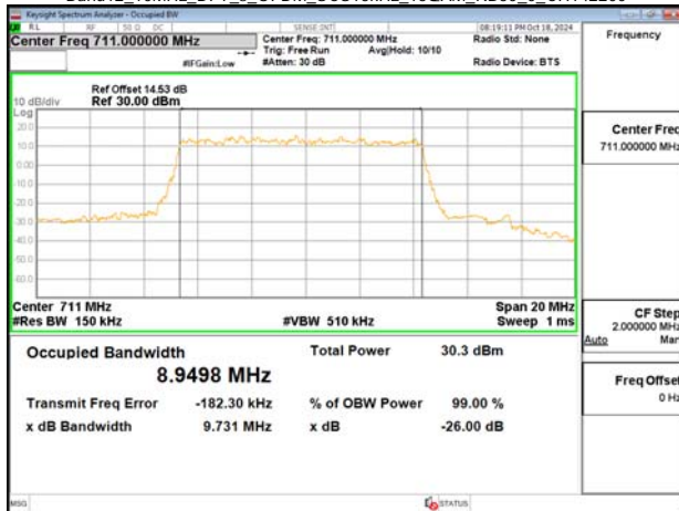
Band12_10MHz_DFT_s_OFDM_SCS15kHz_16QAM_RB50_0_CH142200
