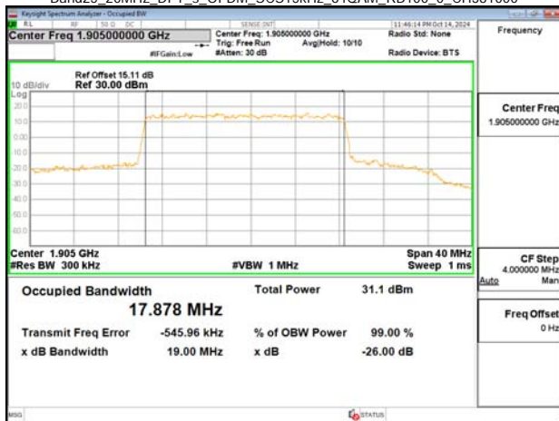
Band25_20MHz_DFT_s_OFDM_SCS15kHz_64QAM_RB100_0_CH381000
