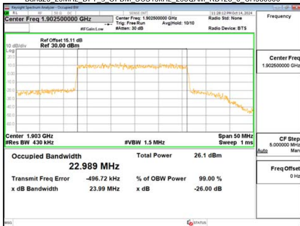
Band25_25MHz_DFT_s_OFDM_SCS15kHz_256QAM_RB128_0_CH380500
