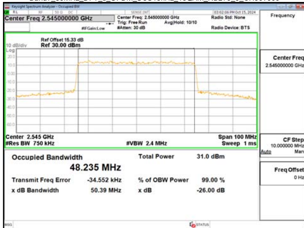
Band7_50MHz_DFT_s_OFDM_SCS15kHz_16QAM_RB270_0_CH509000
