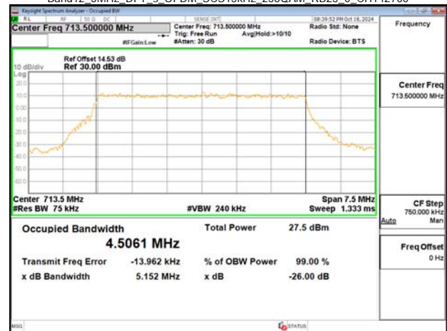
Band12_5MHz_DFT_s_OFDM_SCS15kHz_256QAM_RB25_0_CH142700
