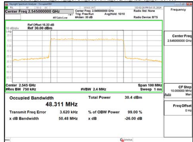
Band7_50MHz_DFT_s_OFDM_SCS15kHz_64QAM_RB270_0_CH509000
