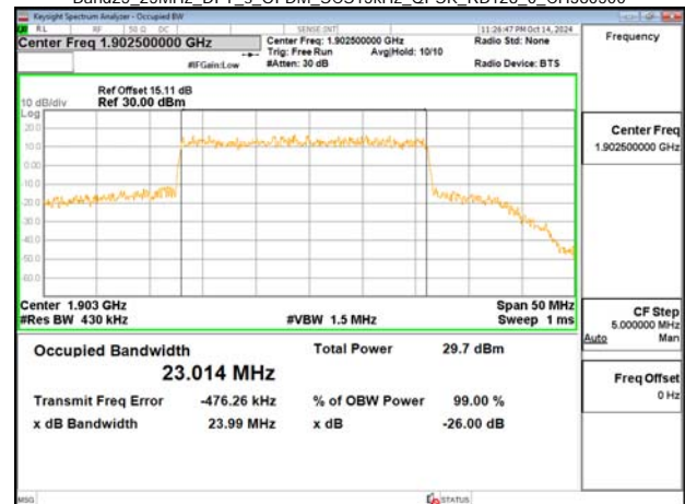
Band25_25MHz_DFT_s_OFDM_SCS15kHz_QPSK_RB128_0_CH380500
