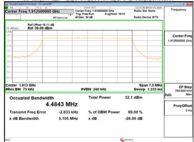
Band25_5MHz_DFT_s_OFDM_SCS15kHz_QPSK_RB25_0_CH382500
