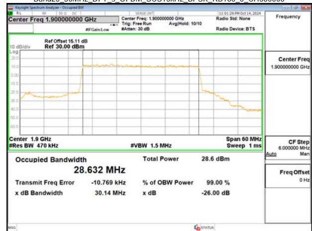
Band25_30MHz_DFT_s_OFDM_SCS15kHz_BPSK_RB160_0_CH380000
