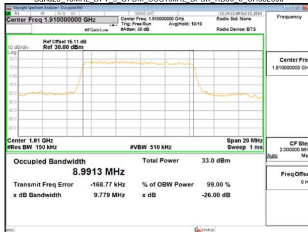
Band25_10MHz_DFT_s_OFDM_SCS15kHz_BPSK_RB50_0_CH382000
