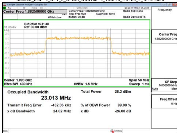
Band25_25MHz_DFT_s_OFDM_SCS15kHz_16QAM_RB128_0_CH380500
