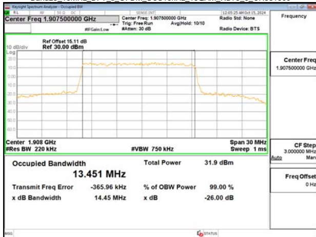
Band25_15MHz_DFT_s_OFDM_SCS15kHz_16QAM_RB75_0_CH381500
