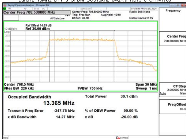
Band12_15MHz_DFT_s_OFDM_SCS15kHz_64QAM_RB75_0_CH141700
