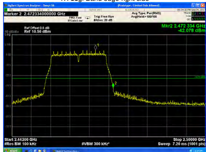
TX 11g: Band edge-right side
