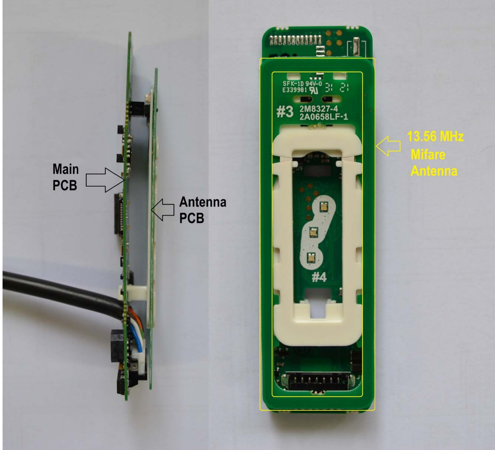
T15 Mifare - 13.56 MHz Mifare Antenna and Main PCB
