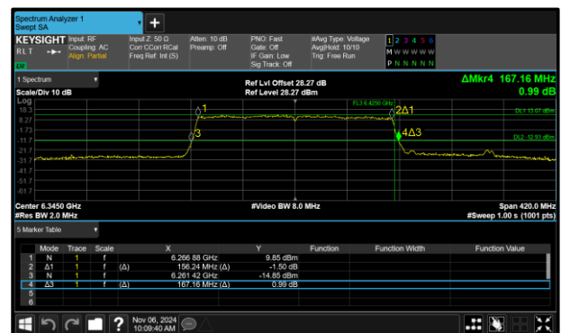
Figure 124 - 802.11ax HE160 SU SP Maximum 26 dB EBW
