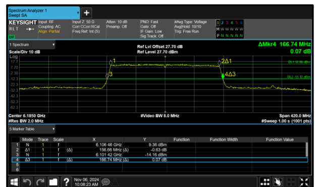
Figure 148 - 802.11ax HE160 SU SP Maximum 99% OBW
