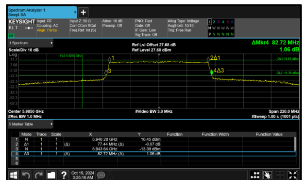
Figure 146 - 802.11ax HE80 SU SP Maximum 99% OBW
