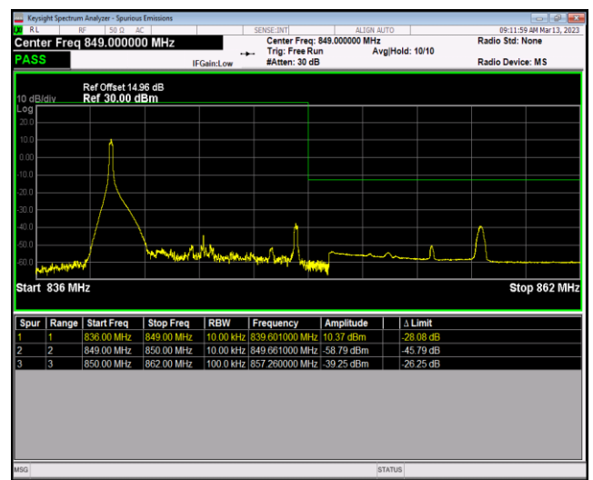
Band5-10MHz-64QAM-20600-50RB#0
