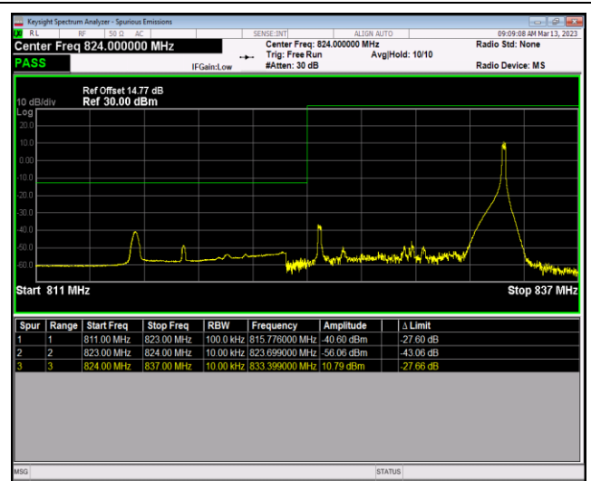
Band5-10MHz-64QAM-20600-1RB#0
