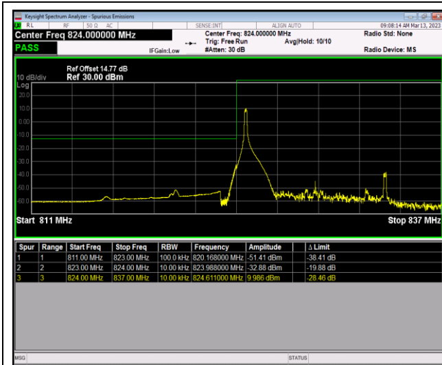
Band5-10MHz-64QAM-20450-50RB#0
