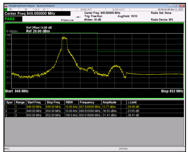
Band5-1.4MHz-QPSK-20643-6RB#0
