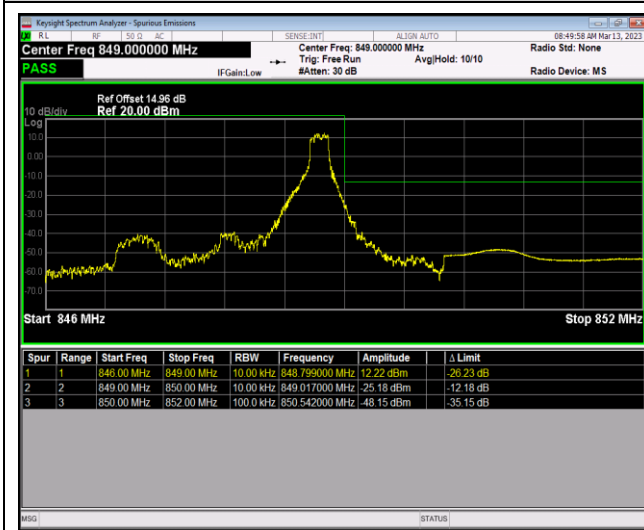
Band5-1.4MHz-64QAM-20407-1RB#0
