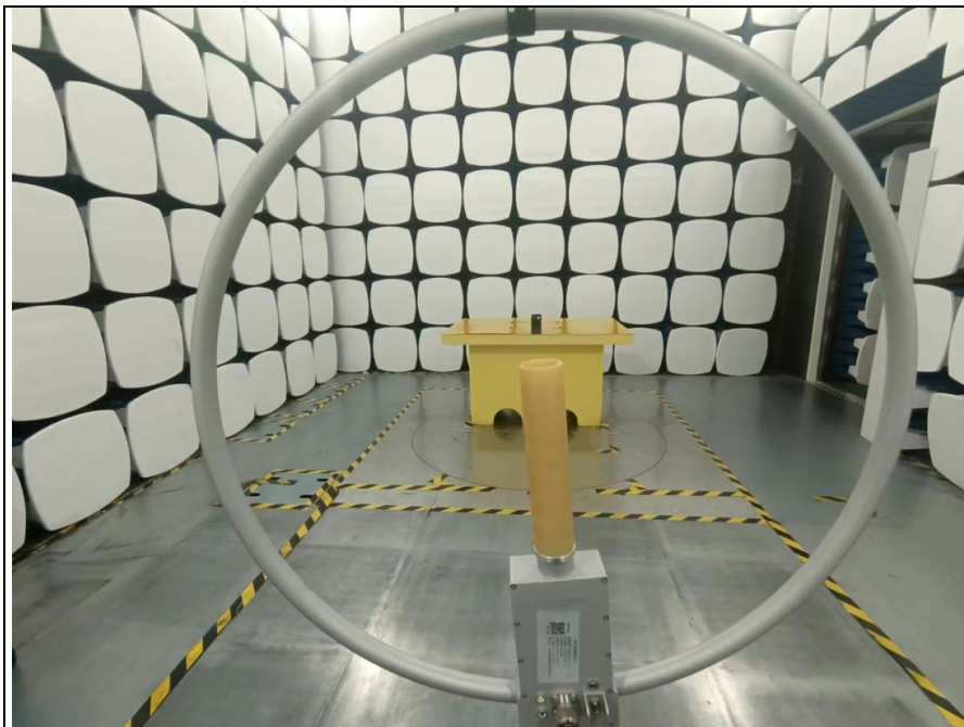
For NFC battery power supply,9kHz-30MHz&13.11MHz-14.01MHz(FCC&IC)
