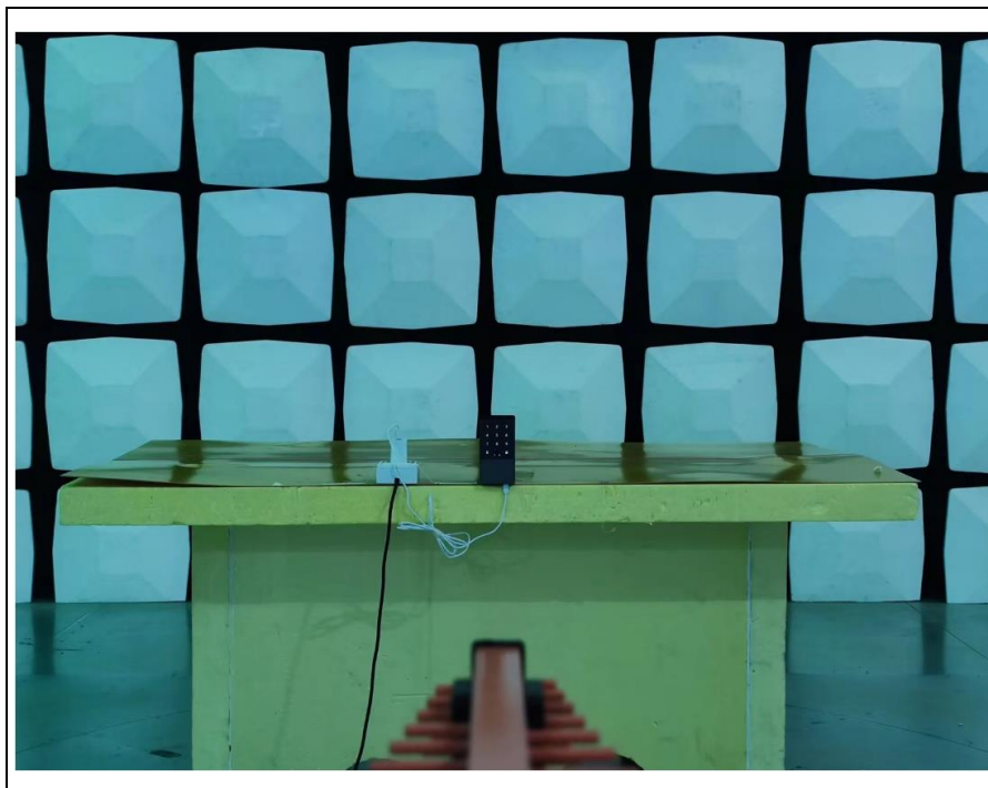
For NFC adapter power supply ,30MHz-1GHz(FCC&IC)
