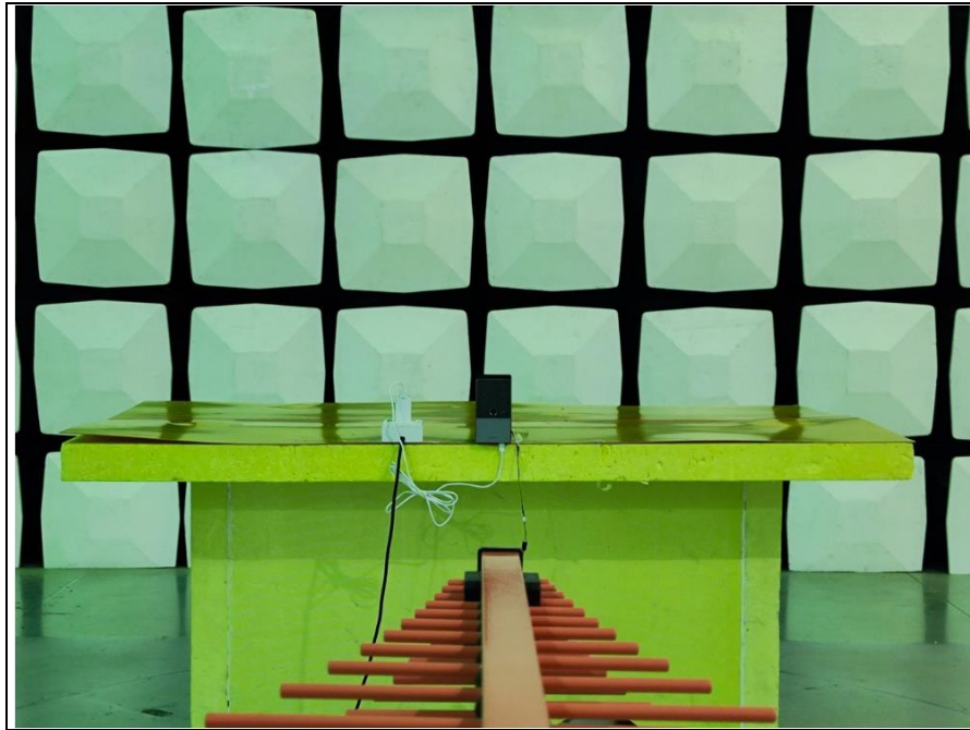
For Zigbee&BLE adapter power supply ,30MHz-1GHz(FCC&IC)
