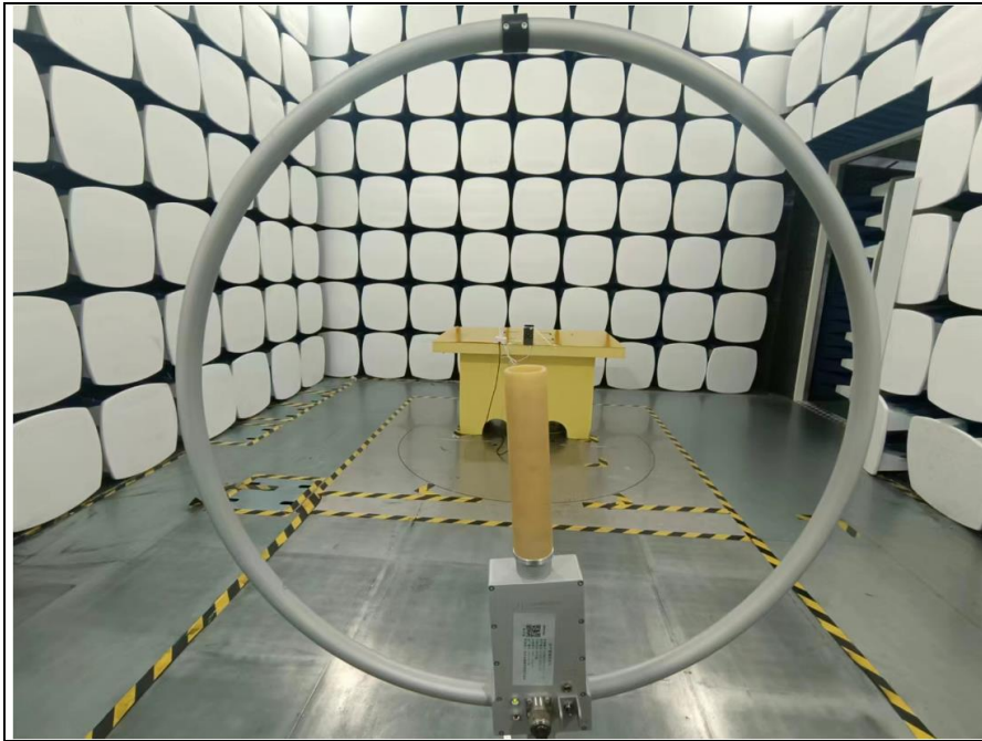
For NFC adapter power supply,9kHz-30MHz&13.11MHz-14.01MHz (FCC&IC)
