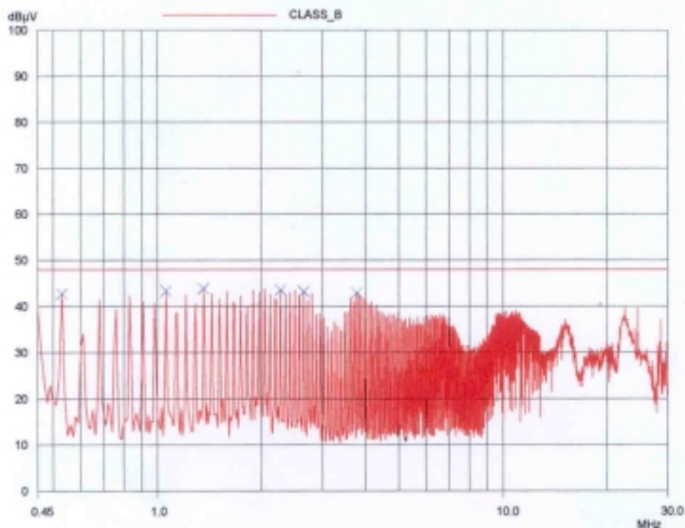
NEUTRAL LINE
