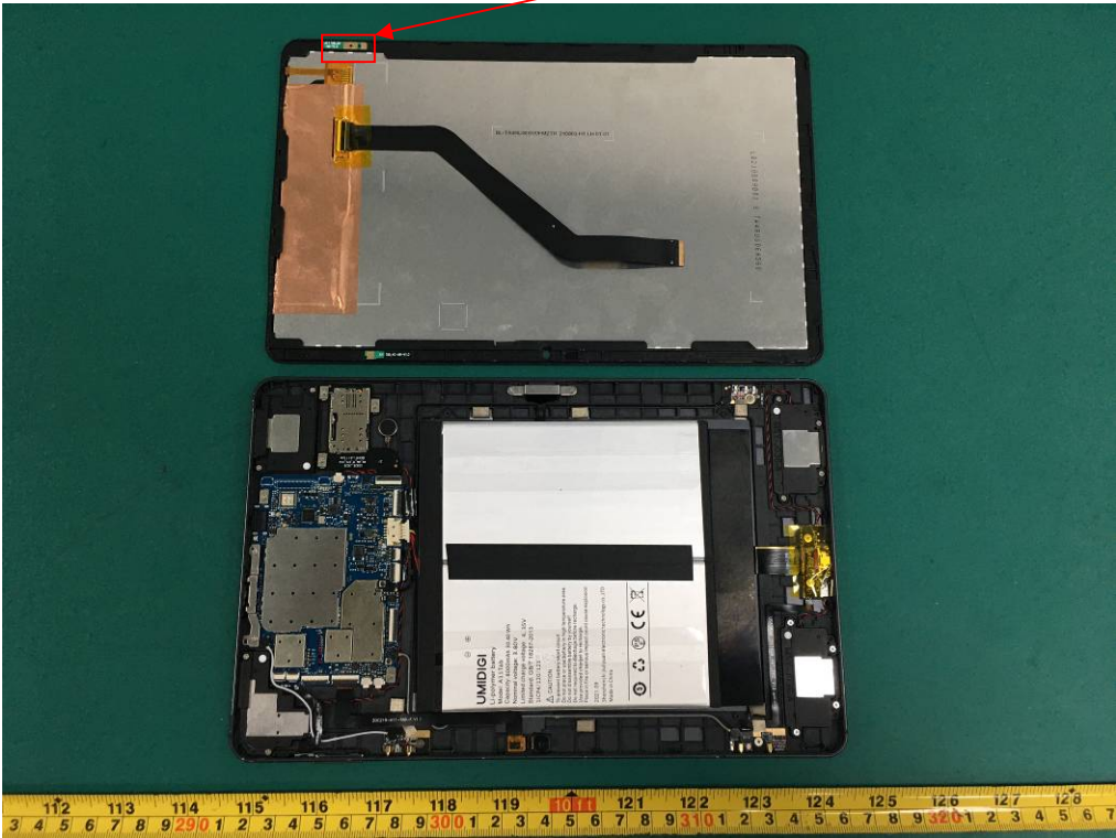
Aux Antenna
