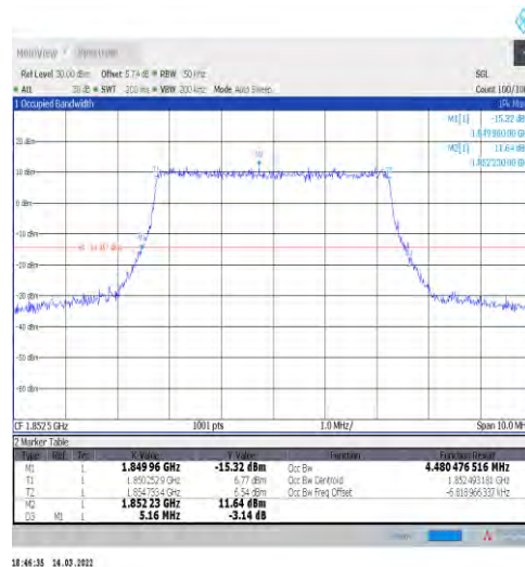
1-N25-15-5-L-4-DFT-64QAM-Outer_Full-25@0-Ant1-4 4.48-5.160-≤5-PASS
