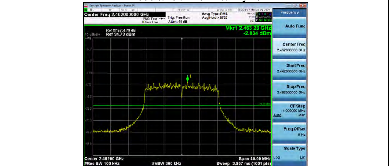
2 Bandedge 2 4GWiFi NVNT ANT2 802 11g 2462
