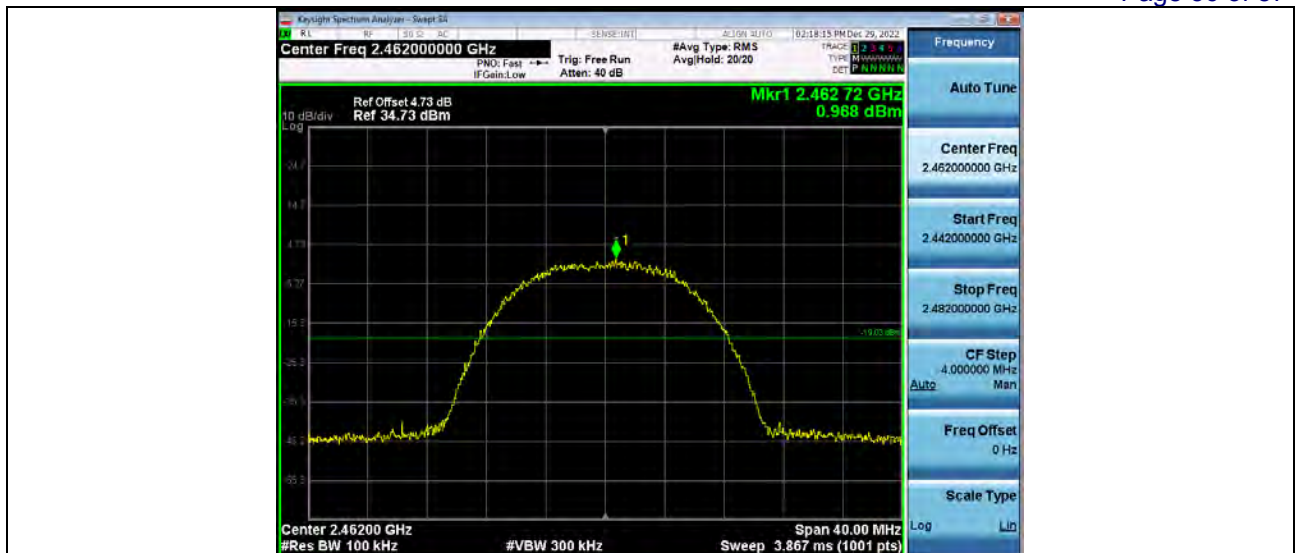
2_Bandedge_2_4GWiFi_NVNT_ANT2_802_11b_2462
