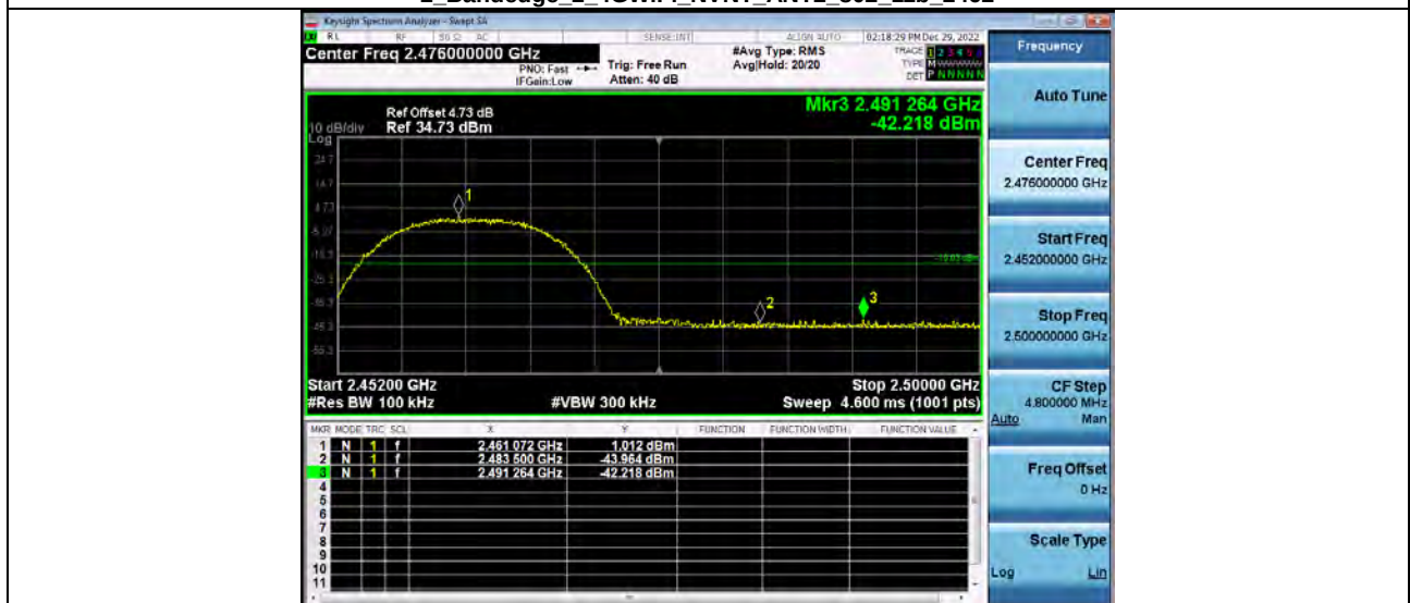
2_Bandedge_2_4GWiFi_NVNT_ANT2_802_11b_2462
