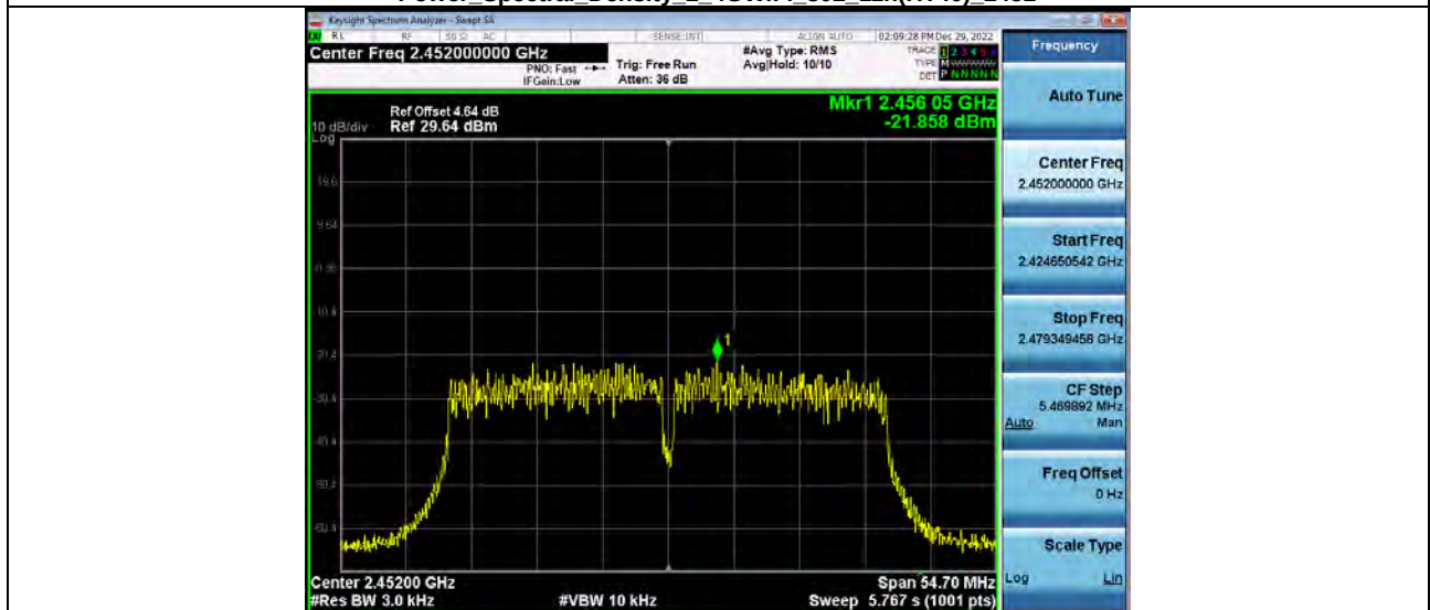
Power Spectral Density 2_4GWiFi 802_11n(HT40) 2452
