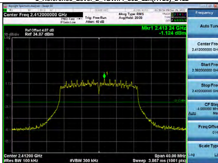
2 Bandedge 2 4GWiFi NVNT ANT1 802 11n(HT20) 2412
