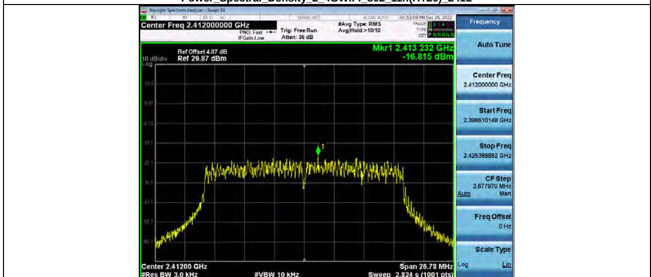
Power Spectral Density 2_4GWiFi 802_11n(HT20)_2412
