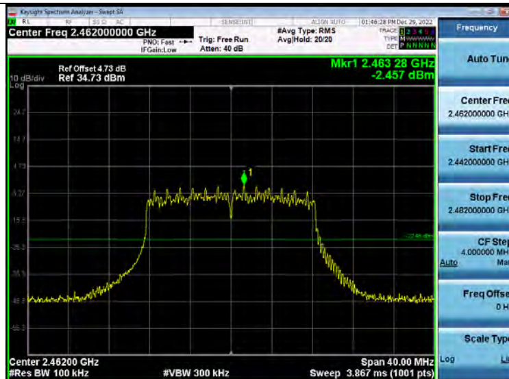
2 Bandedge 2 4GWiFi NVNT ANT1 802 11g 2462
