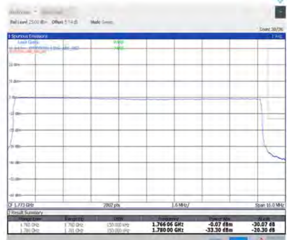
1-N66-PC3-15-15-H-6-CP-QPSK-Outer_Full-79@0-Ant1-seegraph-PASS-see graph
