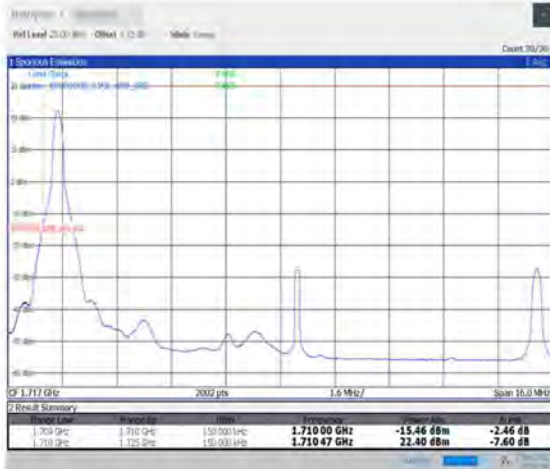
1-N66-PC3-15-15-L-1-DFT-PI2BPSK-Edge_1RB_Left-1@0-Ant1-seegraph-PASS-see graph
