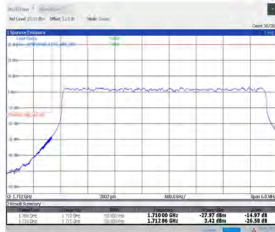
1-N66-PC3-15-5-L-3-DFT-PI2BPSK-Outer_Full-25@0-Ant1-seegraph-PASS-see graph
