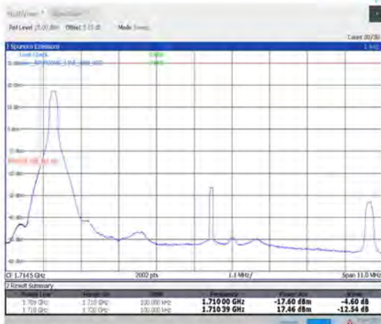
1-N66-PC3-15-10-L-4-CP-QPSK-Edge_1RB_Left-1@0-Ant1-seegraph-PASS-see graph
