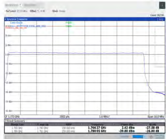
1-N66-PC3-15-15-H-3-DFT-PI2BPSK-Outer_Full-75@0-Ant1-seegraph-PASS-see graph
