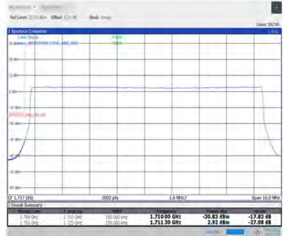
1-N66-PC3-15-15-L-3-DFT-PI2BPSK-Outer_Full-75@0-Ant1-seegraph-PASS-see graph
