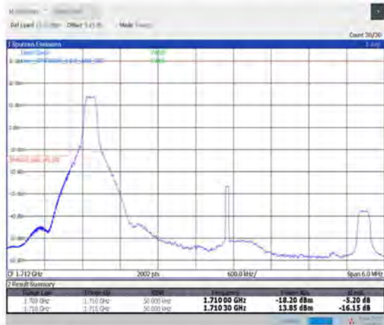
1-N66-PC3-15-5-L-4-CP-QPSK-Edge_1RB_Left-1@0-Ant1-seegraph-PASS-see graph
