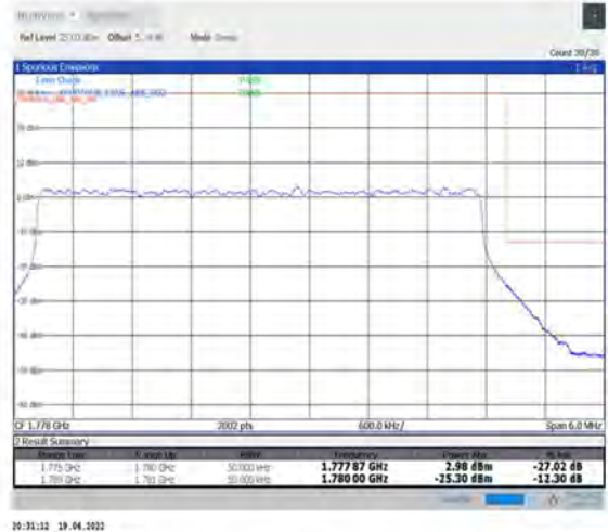
1-N66-PC3-15-5-H-3-DFT-PI2BPSK-Outer_Full-25@0-Ant1-seegraph-PASS-see graph
