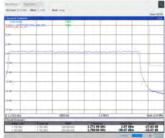
1-N66-PC3-15-10-H-3-DFT-PI2BPSK-Outer_Full-50@0-Ant1-seegraph-PASS-see graph
