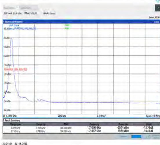
1-N66-PC3-15-30-L-4-CP-QPSK-Edge_1RB_Left-1@0-Ant1-seegraph-PASS-see graph
