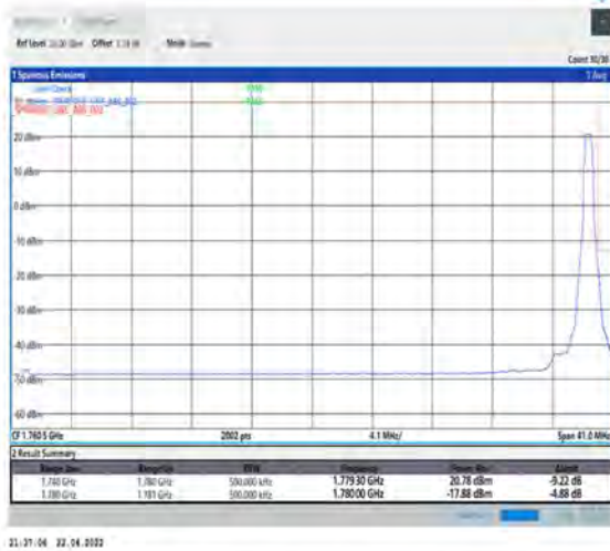
1-N66-PC3-15-40-H-2-DFT-PI2BPSK-Edge_1RB_Right-1@215-Ant1-seegraph-PASS-see graph
