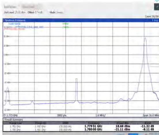
1-N66-PC3-15-15-H-5-CP-QPSK-Edge_1RB_Right-1@78-Ant1-seegraph-PASS-see graph
