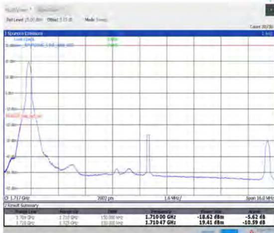
1-N66-PC3-15-15-L-4-CP-QPSK-Edge_1RB_Left-1@0-Ant1-seegraph-PASS-see graph
