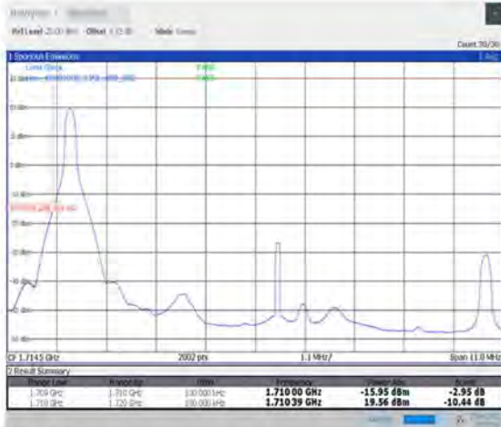
1-N66-PC3-15-10-L-1-DFT-PI2BPSK-Edge_1RB_Left-1@0-Ant1-seegraph-PASS-see graph
