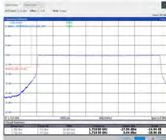
1-N66-PC3-15-5-L-6-CP-QPSK-Outer_Full-25@0-Ant1-seegraph-PASS-see graph
