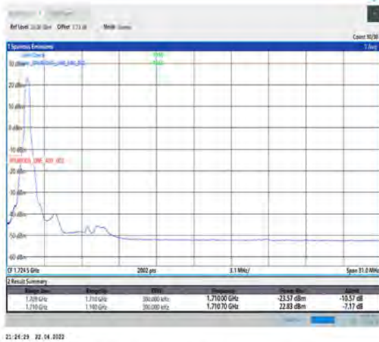
1-N66-PC3-15-30-L-1-DFT-PI2BPSK-Edge_1RB_Left-1@0-Ant1-seegraph-PASS-see graph
