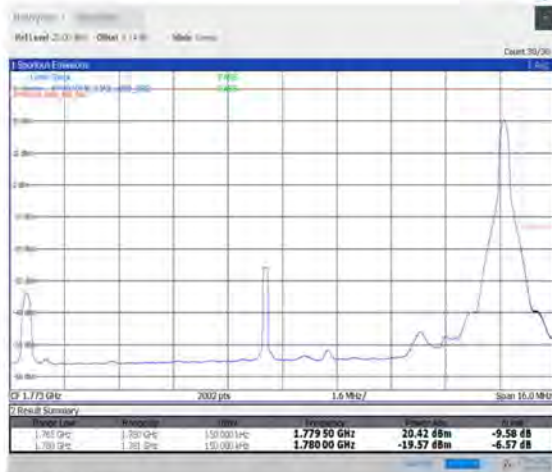
1-N66-PC3-15-15-H-2-DFT-PI2BPSK-Edge_1RB_Right-1@78-Ant1-seegraph-PASS-see graph
