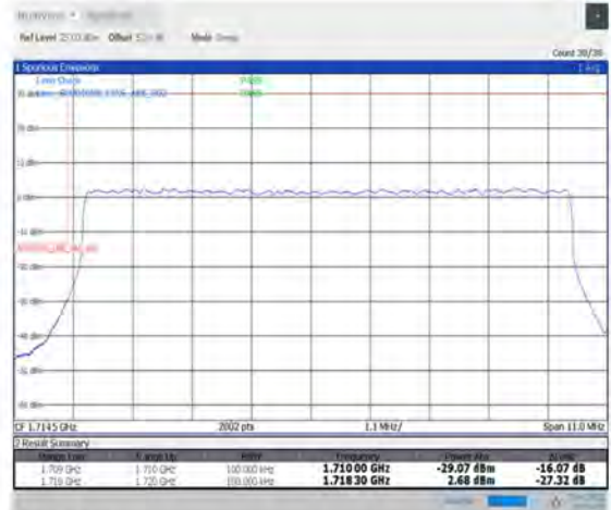
1-N66-PC3-15-10-L-3-DFT-PI2BPSK-Outer_Full-50@0-Ant1-seegraph-PASS-see graph
