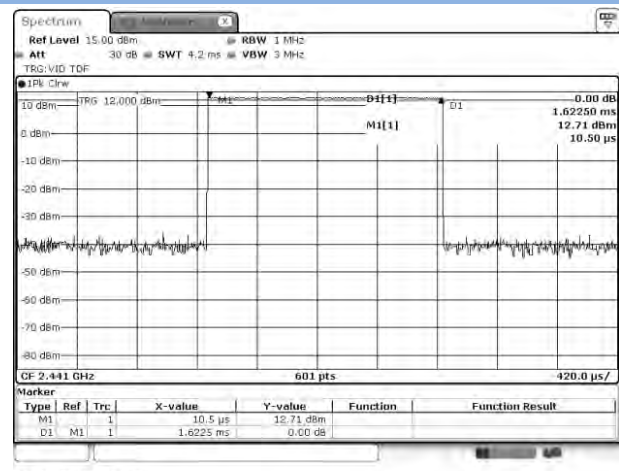
GFSK DH3
