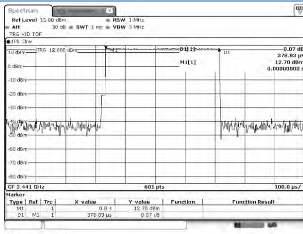
GFSK DH1
