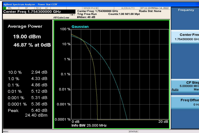
Band4-1.4MHz-16QAM-20393-6RB#0
