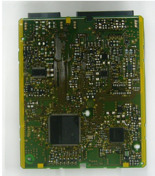
Figure 8.8 R515E PCB assy (back view)
