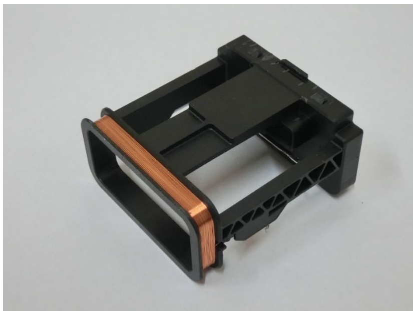
Figure 8.12 C8Z-F116M internal (back view)
