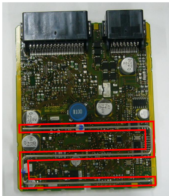
Figure 8.7.2 R515E integral antenna ( for UHF receiving ) location
