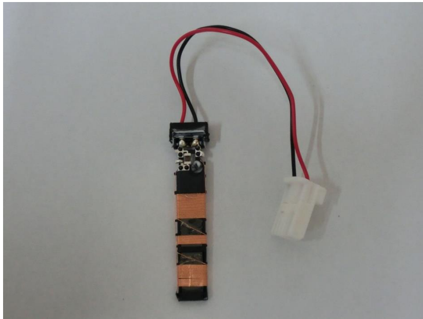
Figure 8.15 CGF-M004-T03 internal (front view)
