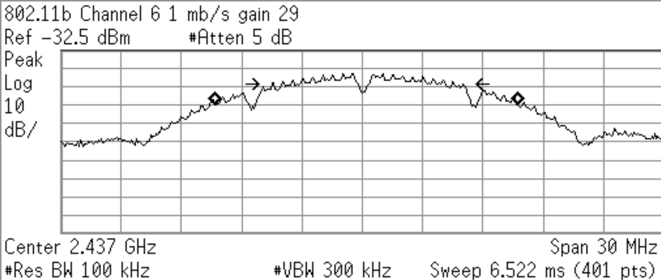
Plot A-2 - 6 dB Bandwidth Mid Channel (802.11b)
