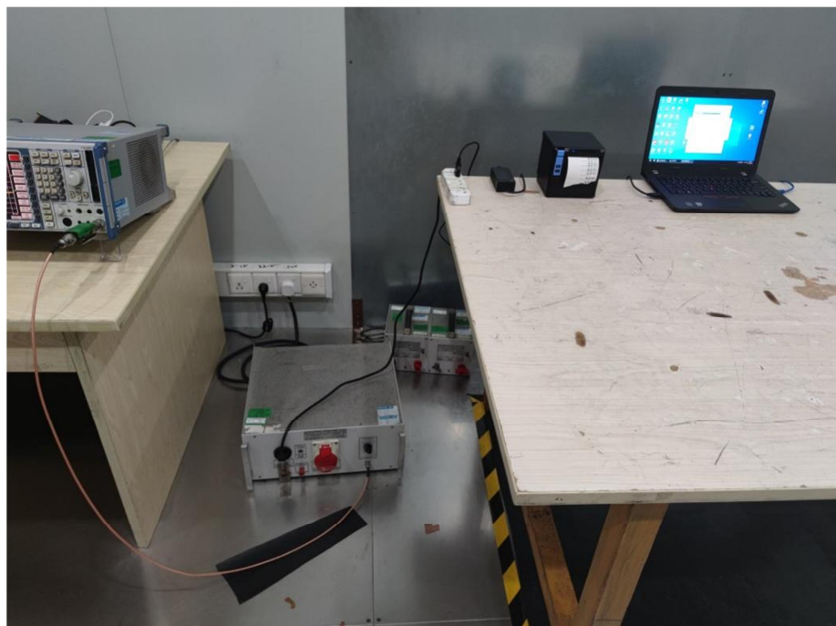
Conducted Emission Test Setup(AP113G-240200)
