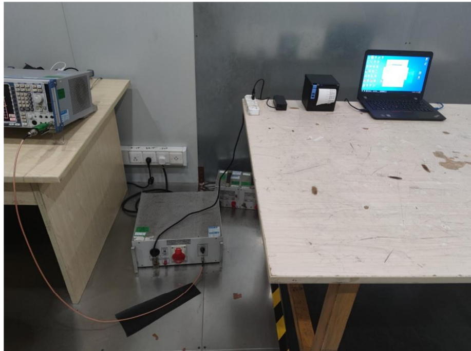
Conducted Emission Test Setup(GM53-240200-D)
