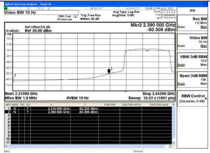
802.11n(HT40)-Low channel(Average)
