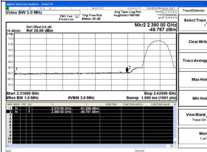
802.11b-Low channel(Peak)
