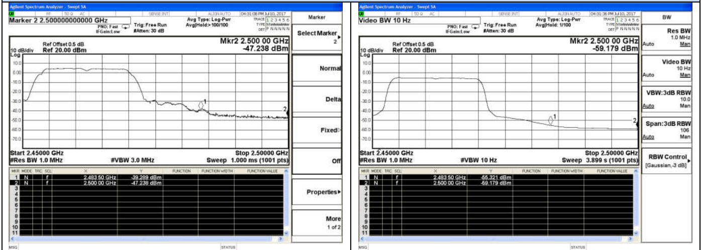
802.11g-High channel(Peak)
