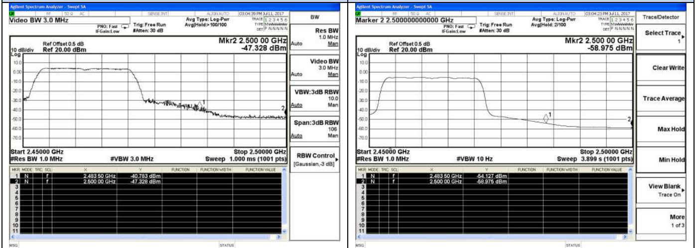
802.11n(HT20)-High channel(Peak)
