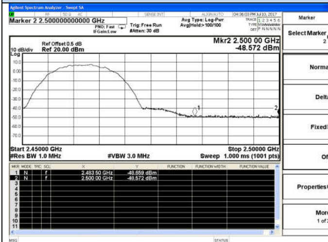
802.11b-High channel(Peak)
