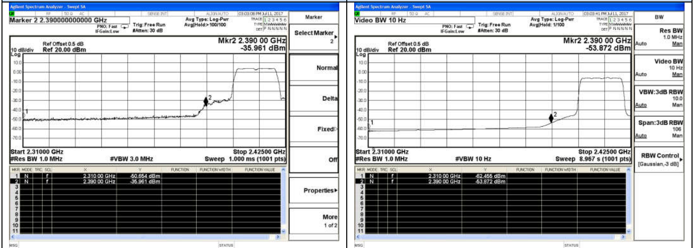
802.11n(HT20)-Low channel(Peak)
