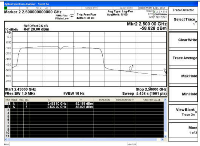
802.11n(HT40)-High channel(Average)
