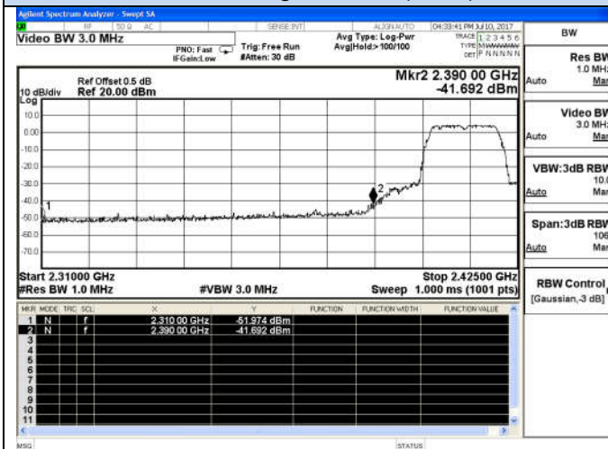
802.11g-Low channel(Peak)
