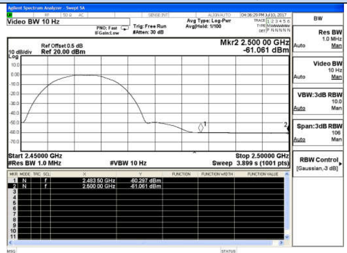
802.11b-High channel(Average)
