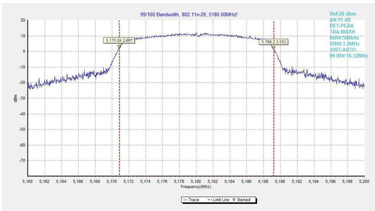
Fig.61 99% Occupied bandwidth (802.11n-HT20, 5180MHz)
