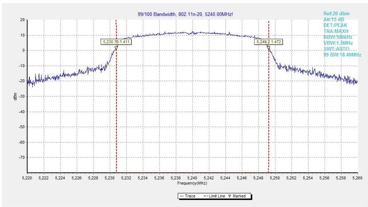
Fig.63 99% Occupied bandwidth (802.11n-HT20, 5240MHz)
