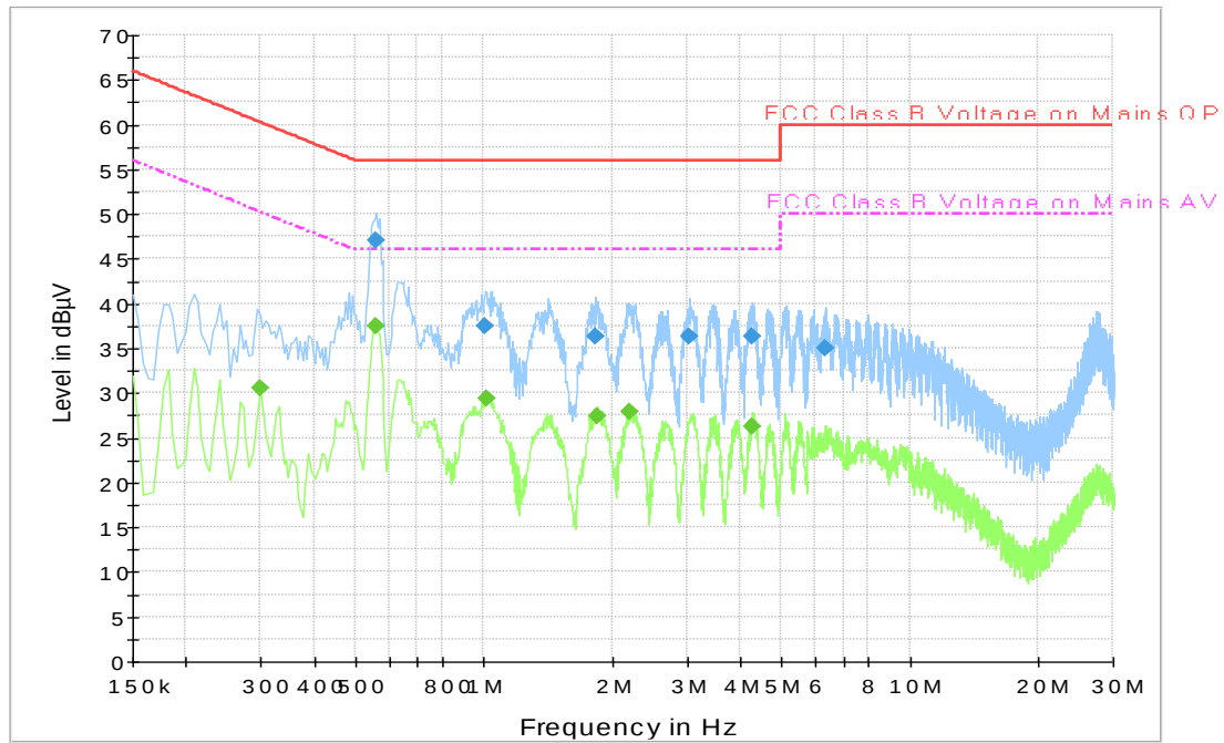
Fig.57 AC Powerline Conducted Emission-Idle
