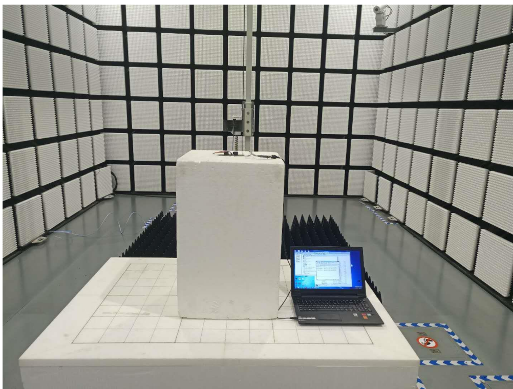
Radiated spurious emission(1GHz~26GHz)
