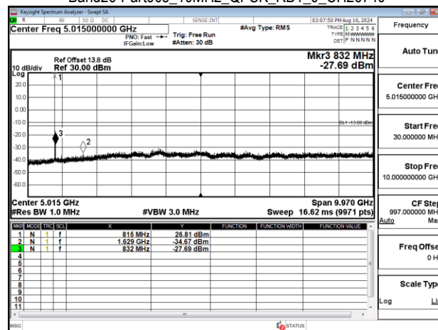
Band26-Part90s_10MHz_QPSK_RB1_0_CH26740
