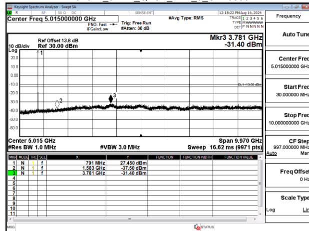
Band14_5MHz_QPSK_RB1_0_CH23330
