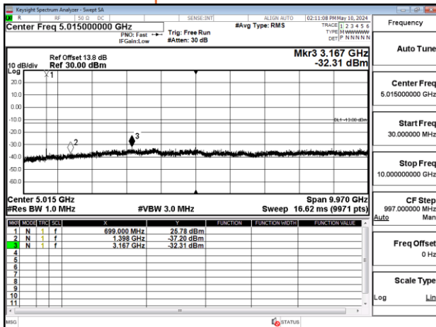
Band12_1.4MHz_QPSK_RB1_0_CH23095
