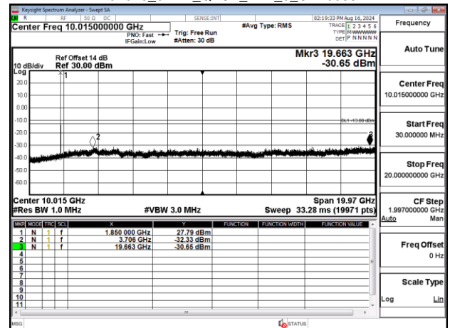
Band25_1.4MHz_QPSK_RB1_0_CH26055
