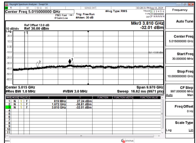
Band26-Part90s_1.4MHz_QPSK_RB1_0_CH26783
