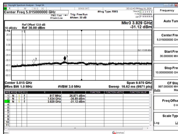
Band26-Part90s_5MHz_QPSK_RB1_0_CH26765
