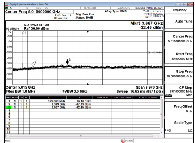
Band12_3MHz_QPSK_RB1_0_CH23095
