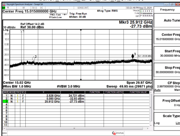
Band7_15MHz_QPSK_RB1_0_CH21375
