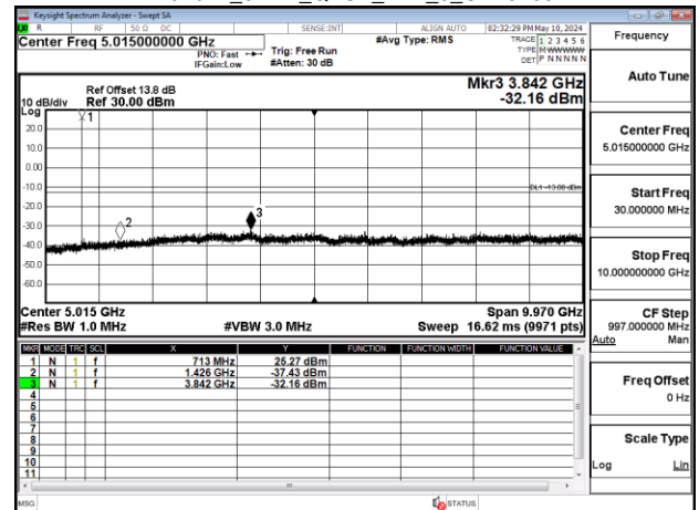
Band12_3MHz_QPSK_RB1_0_CH23165
