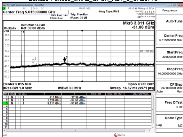
Band26-Part90s_5MHz_QPSK_RB1_0_CH26715
